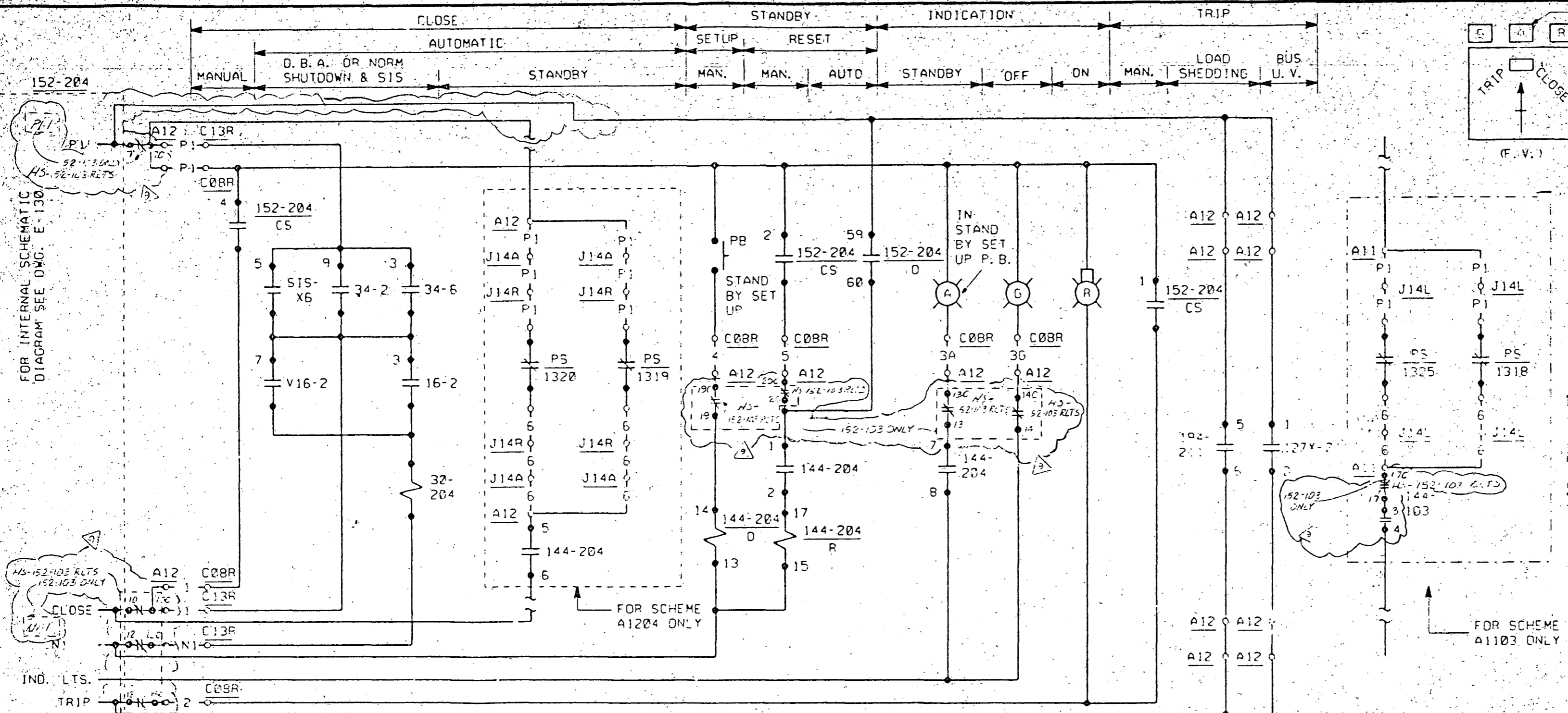
SERVICE WATER PUMP P7A SCHEME A1204
