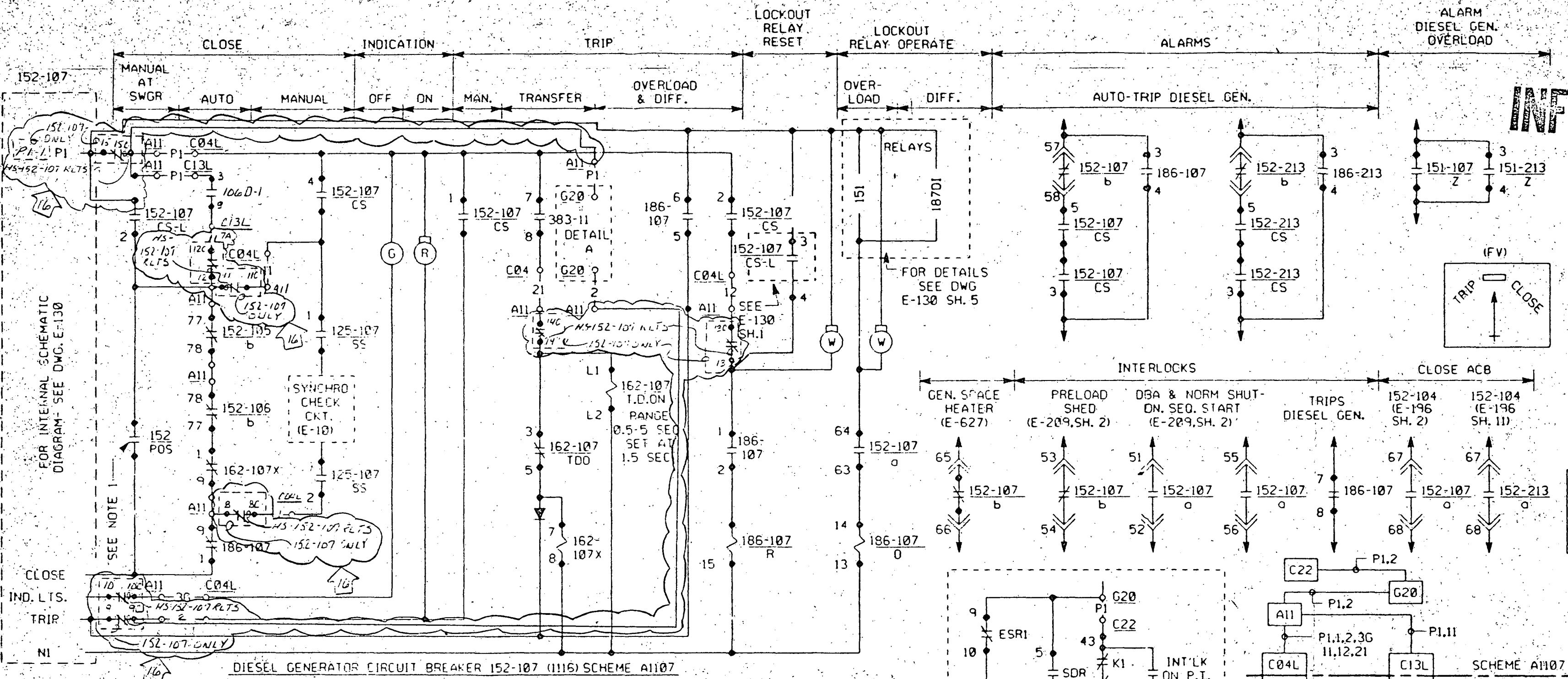
CONTROL SWITCH 152-107 CS G.E. TYPE SBM SPRING RETURN LOCATION C04 - NOT USED
