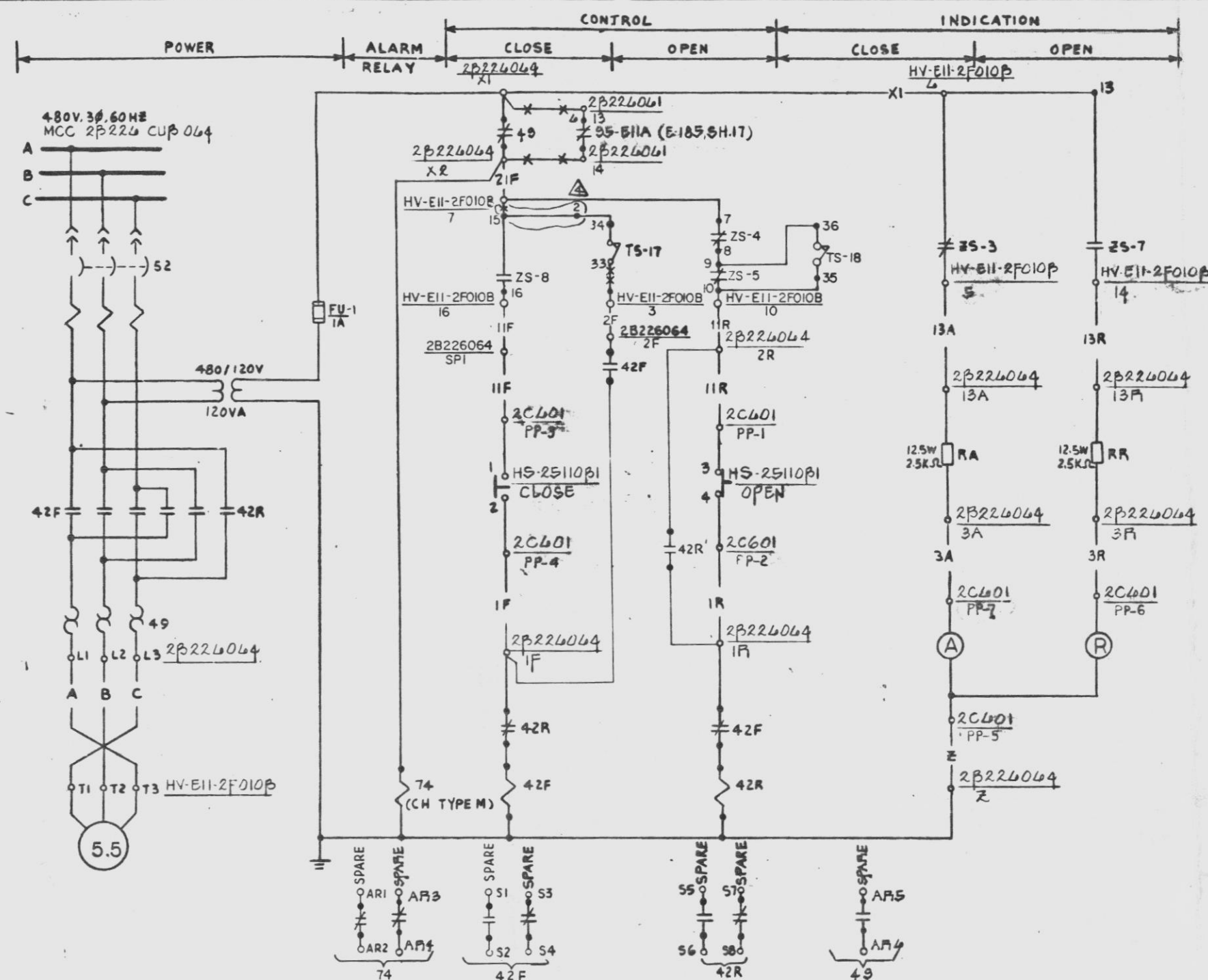
RHR CROSS HEADER SHUTOFF VALVE HV-E11-2F010B II
