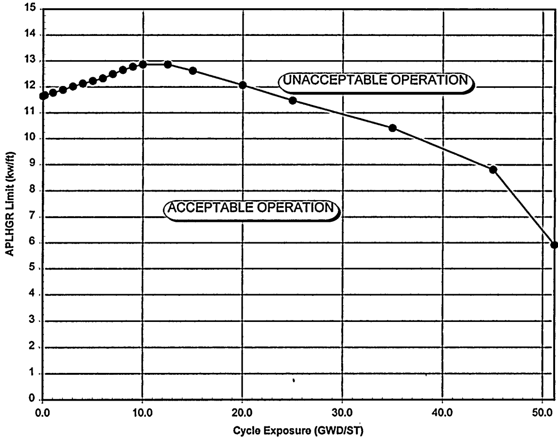
Figure 4 APLHGR Limits for Bundle Type GE9B-P8DWB319-9GZ (GE8X8NB)
