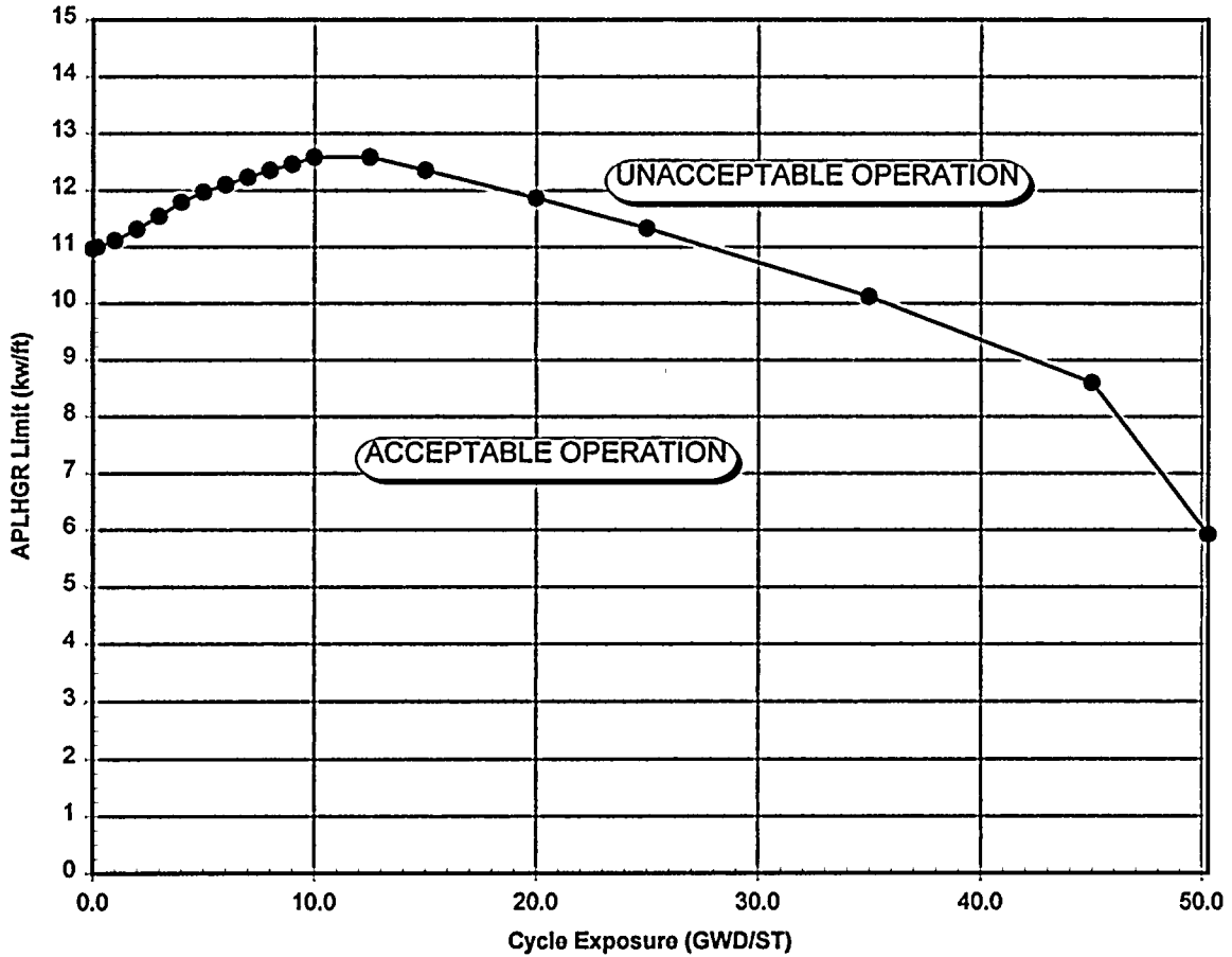
Figure 5 APLHGR Limits for Bundle Type GE9B-P8DWB325-10GZ (GE8X8NB)
