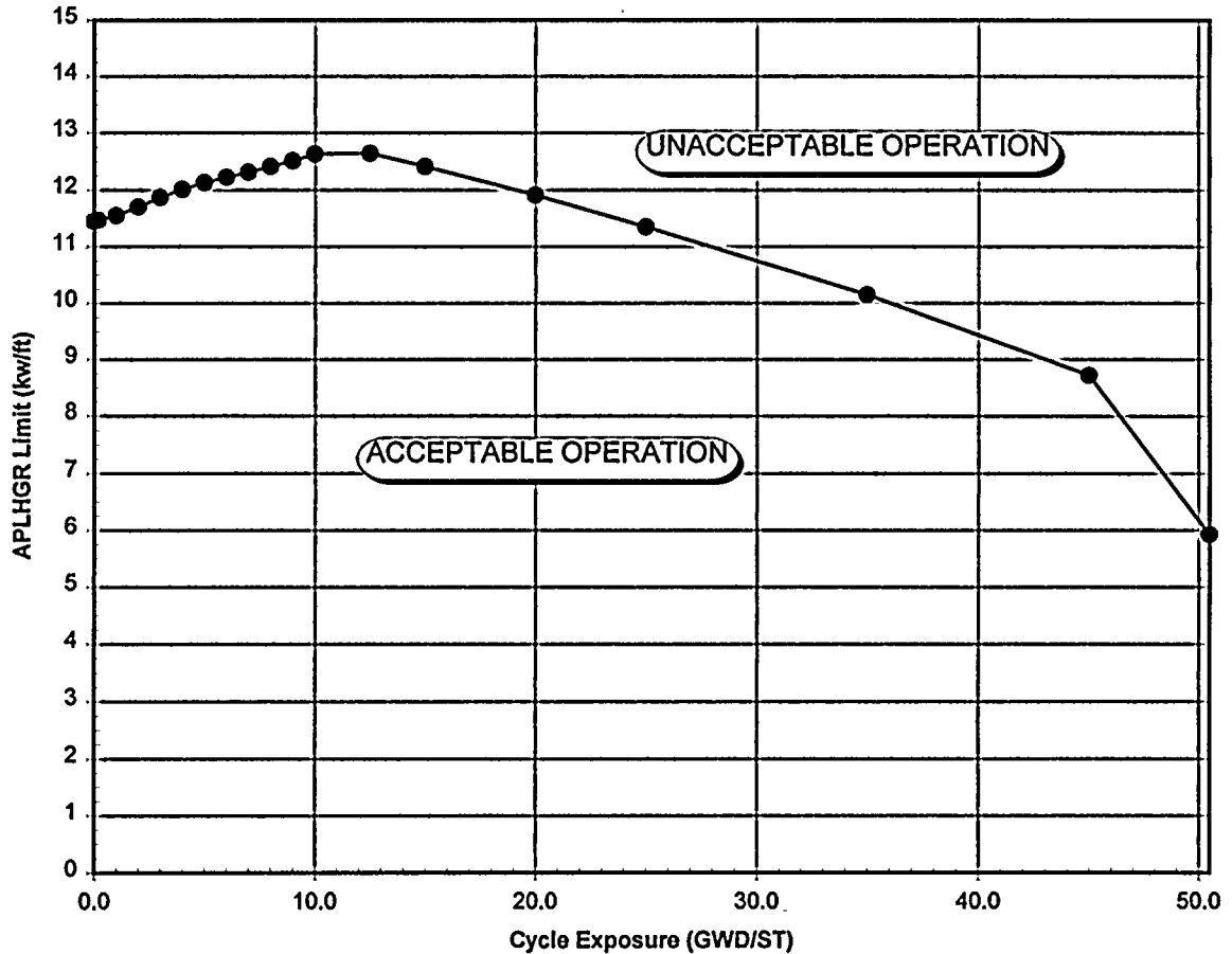
Figure 6 APLHGR Limits for Bundle Type GE9B-P8DWB326-7GZ (GE8X8NB)
