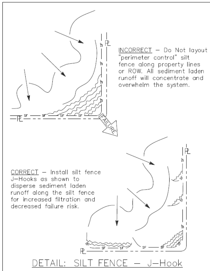
Figure 4 - J-Hook Details.
