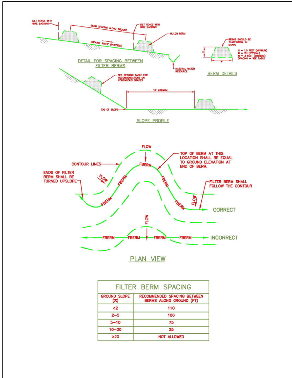
Figure 3 - Mulch Berm.
