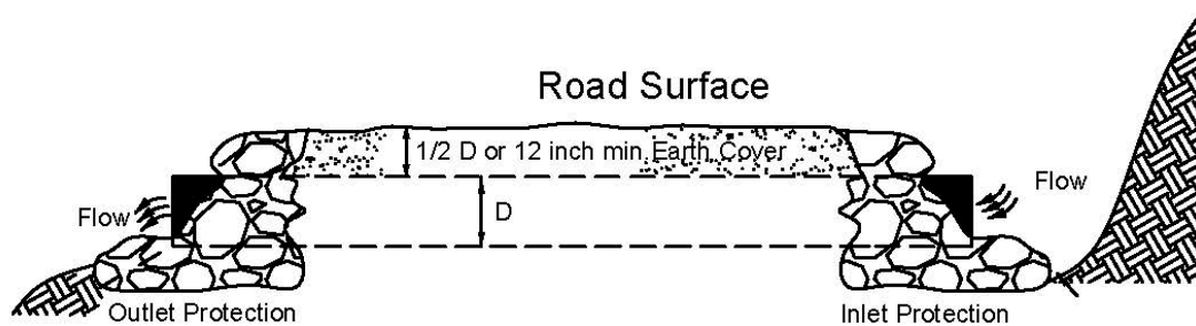
B. CROSS-SECTION
