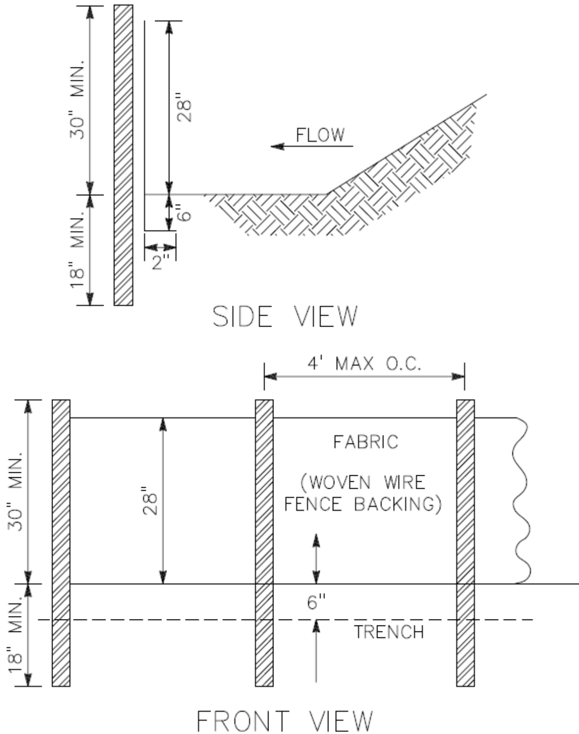
DETAIL: SILT FENCE — TYPE C
