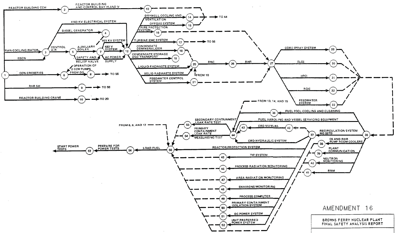
Typical Preoperational Test Sequence FIGURE 13.4-1
