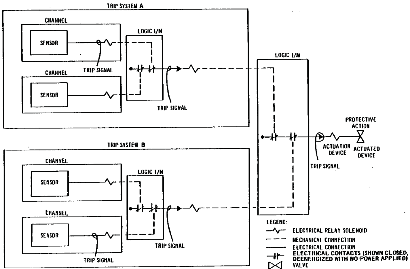
TYPICAL PROTECTION SYSTEM (CONTROL AND INSTRUMENTATION PORTIONS) (NOT A 1/2 x 2 SYSTEM)
