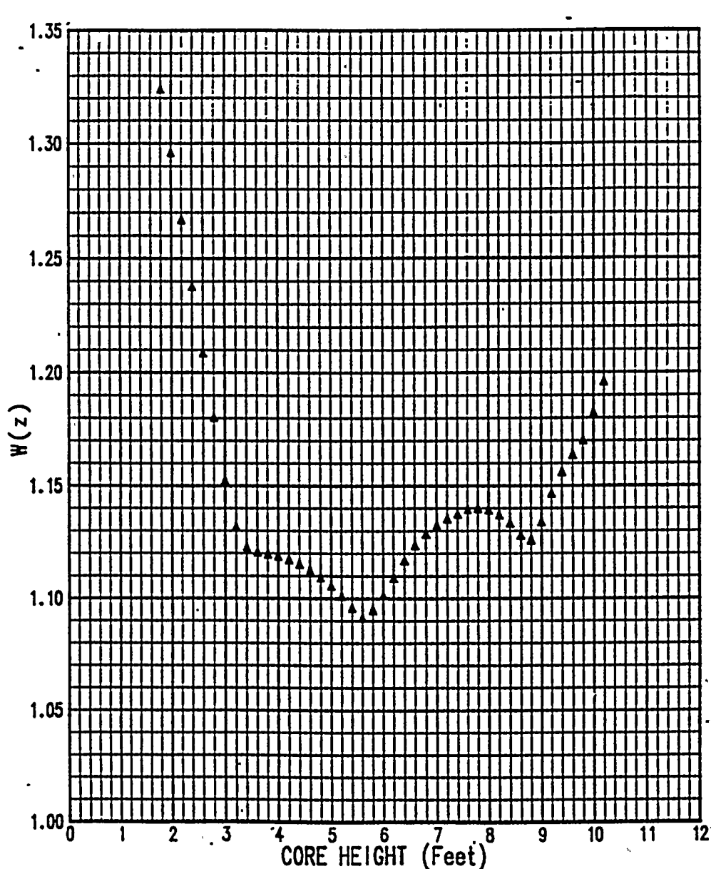
FIGURE 4 RAOC W(Z) AT 150 MWD/MTU (3.6 EFPD)
