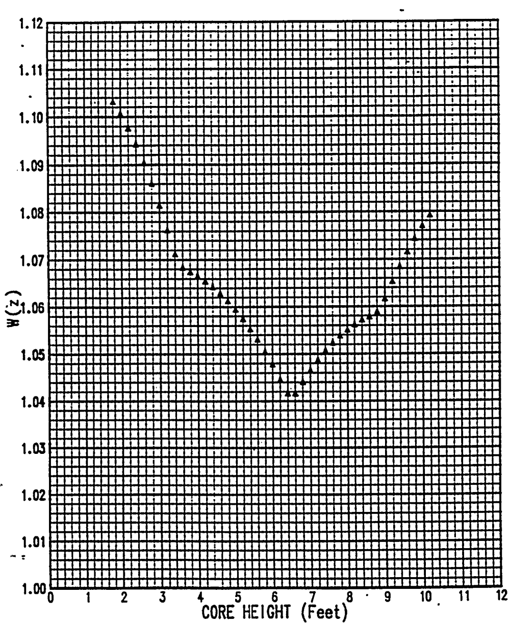
FIGURE 8 BASE LOAD W(Z) AT 9000 MWD/MTU (216.9 EFPD) FOR POWER LEVELS ABOVE 85% OF RATED THERMAL POWER
