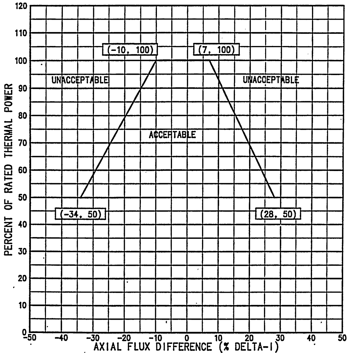
FIGURE 2 AXIAL FLUX DIFFERENCE LIMITS AS A FUNCTION OF RATED THERMAL POWER FOR RAOC
