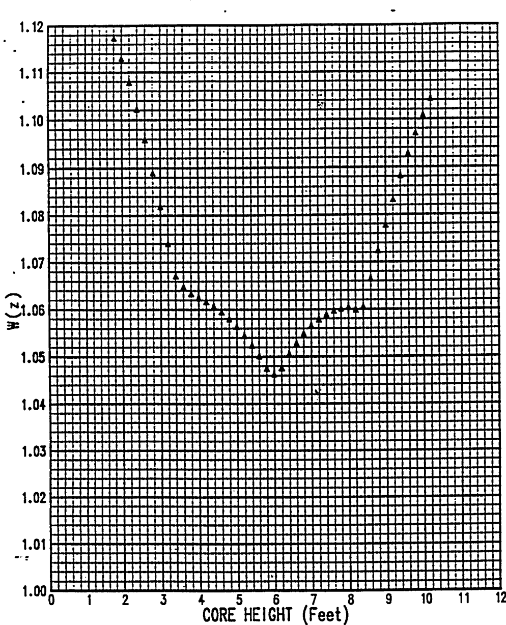
FIGURE 9 BASE LOAD W(z) AT 15000 MWD/MTU (361.5 EFPD) FOR POWER LEVELS ABOVE 85% OF RATED THERMAL POWER
