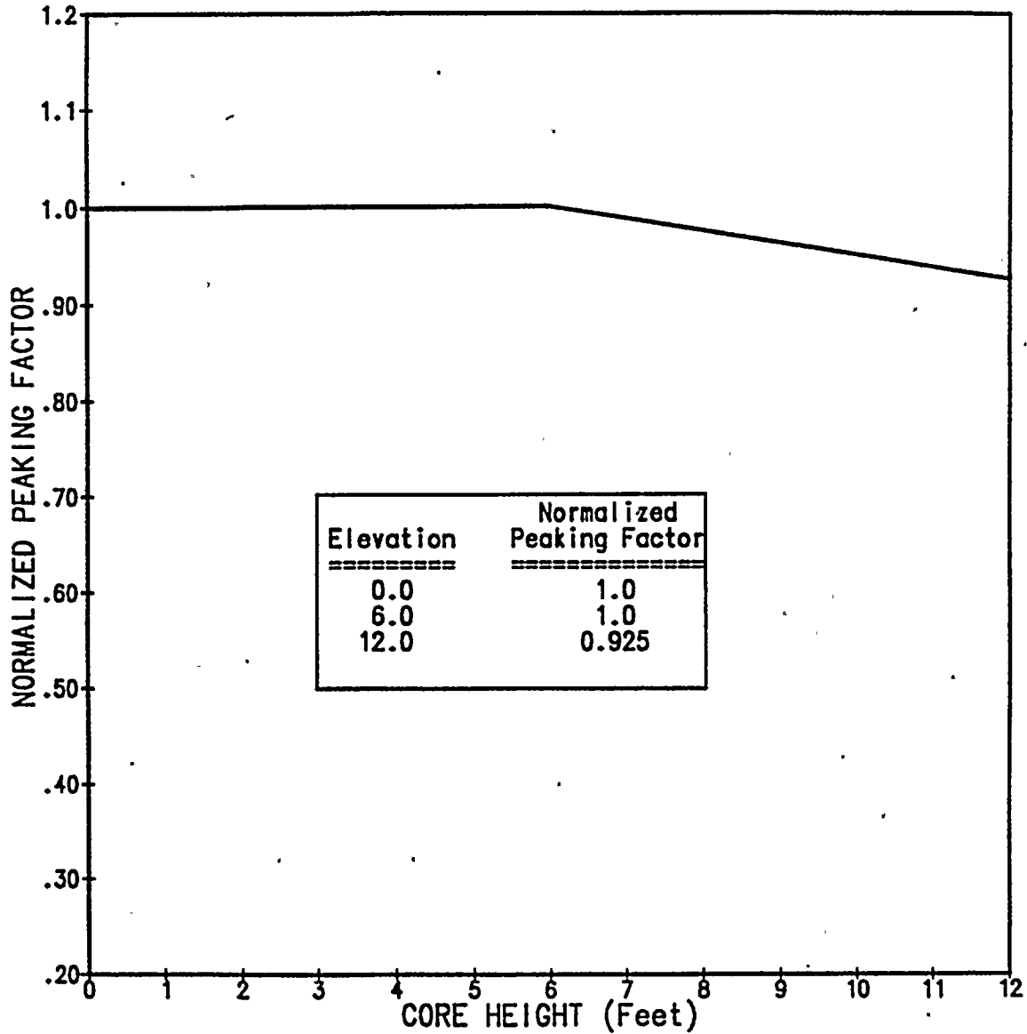
FIGURE 3 K(z) - LOCAL AXIAL PENALTY FUNCTION FOR F_Q(z)
