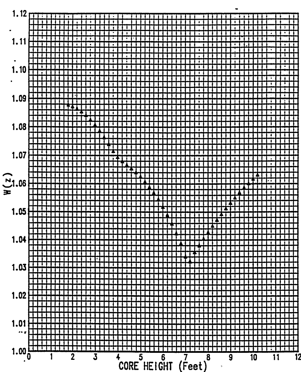
FIGURE 7 BASE LOAD W(Z) AT 150 MWD/MTU (3.6 EFPD) FOR POWER LEVELS ABOVE 85% OF RATED THERMAL POWER
