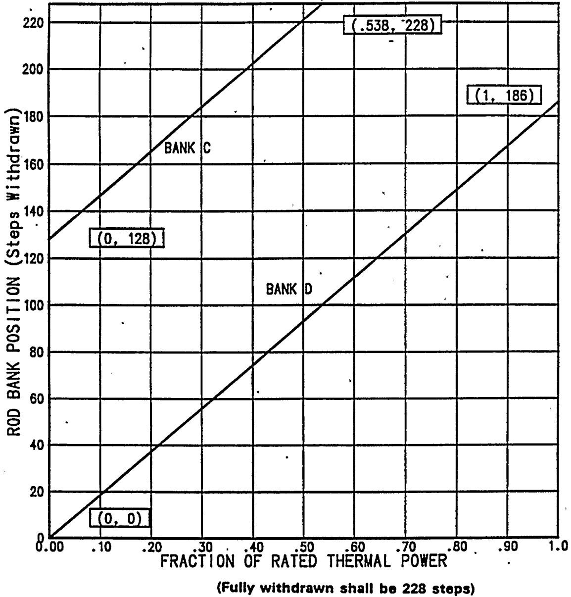
FIGURE 1 ROD GROUP INSERTION LIMITS VERSUS THERMAL POWER (THREE-LOOP OPERATION)
