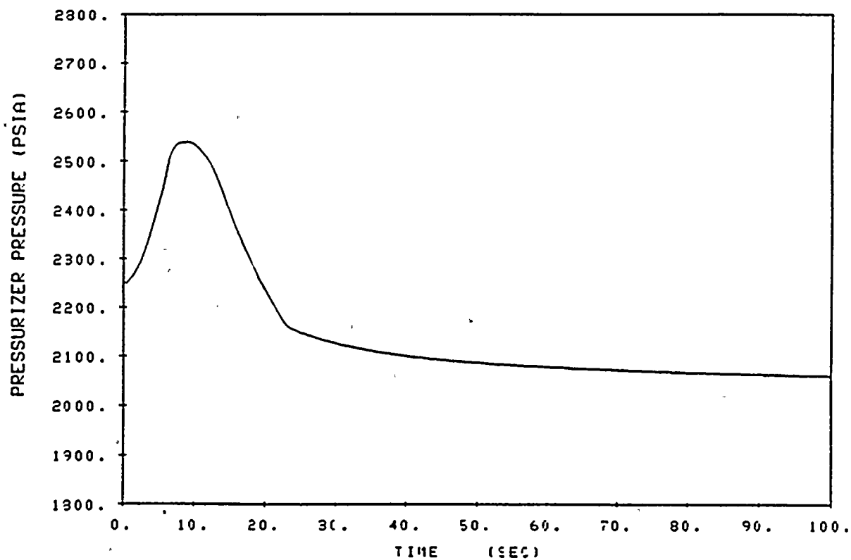
Figure B.3-35A Loss of Load Nuclear Power and Pressurizer Pressure Versus Time for Maximum Reactivity Feedback without Pressurizer Spray and PORVs
