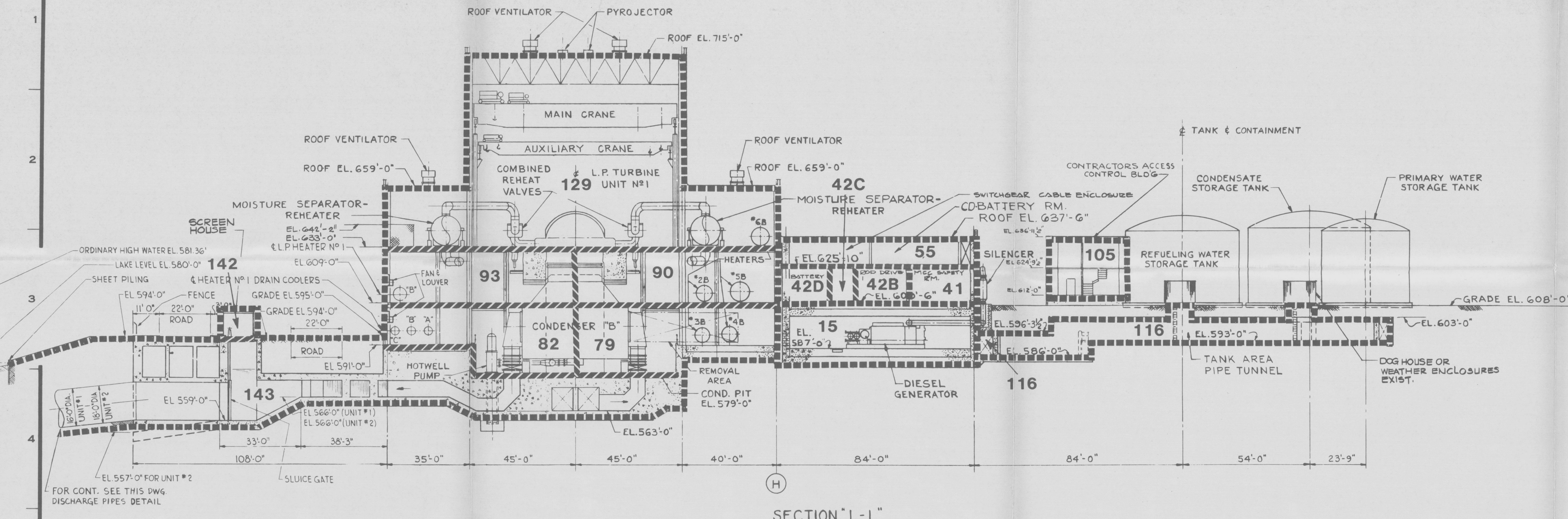
SECTION "L-L"
