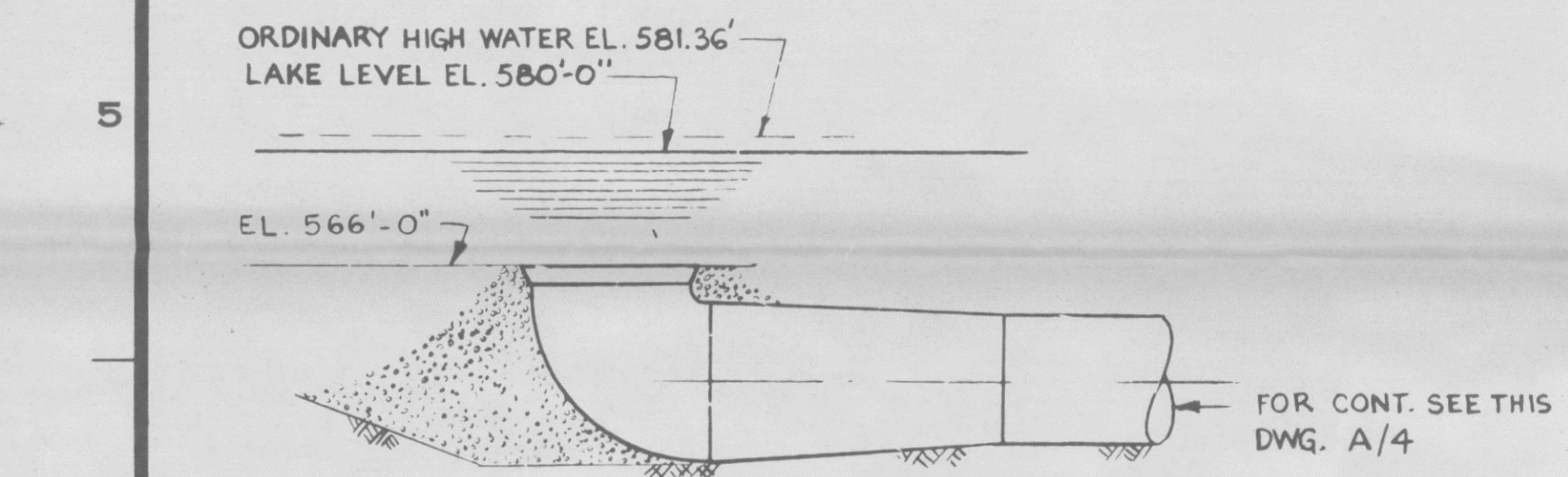
DISCHARGE PIPES DETAIL
