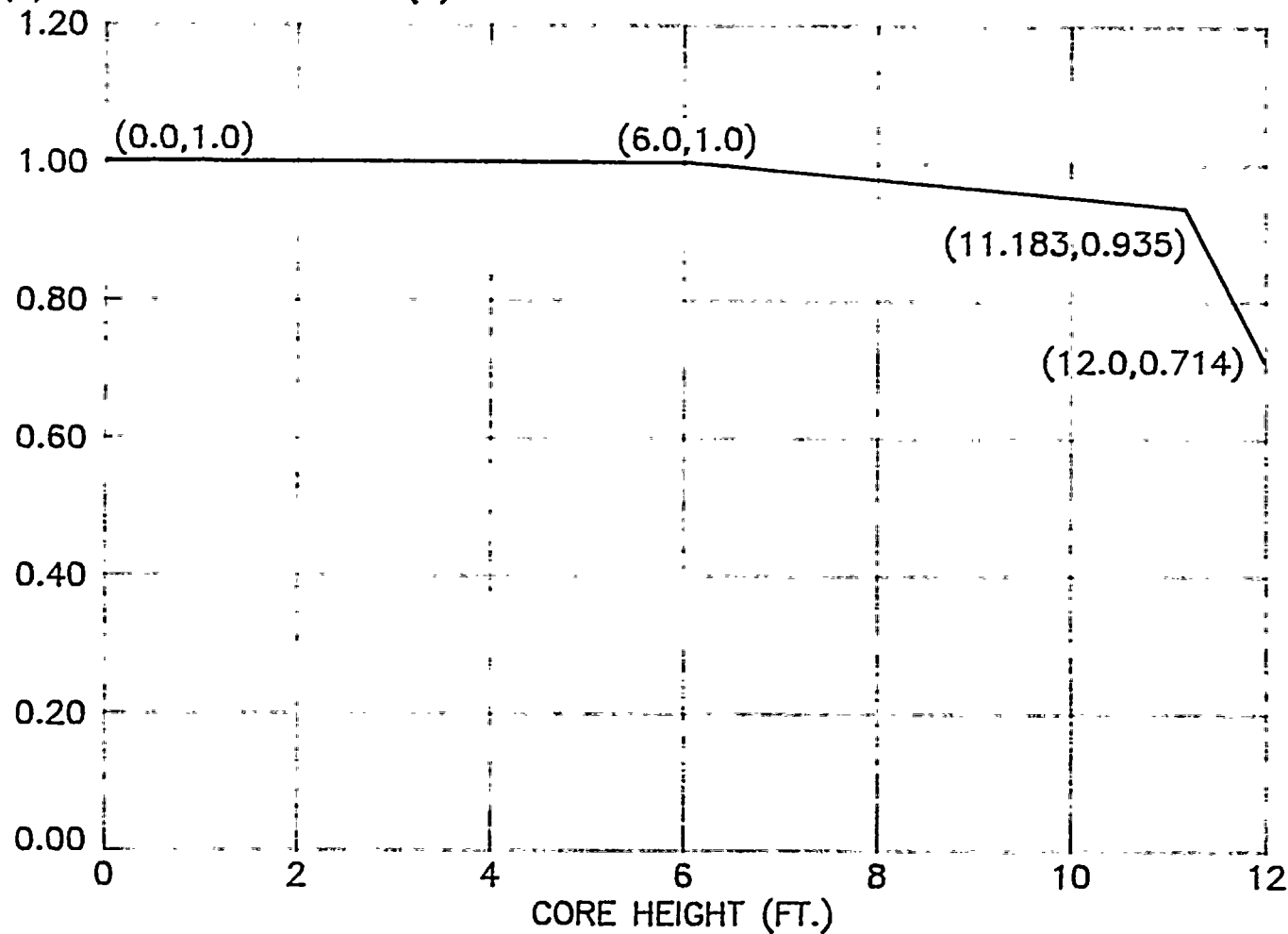
FIGURE 3.2-3 WESTINGHOUSE FUEL K(Z) NORMALIZED VS. CORE HEIGHT
