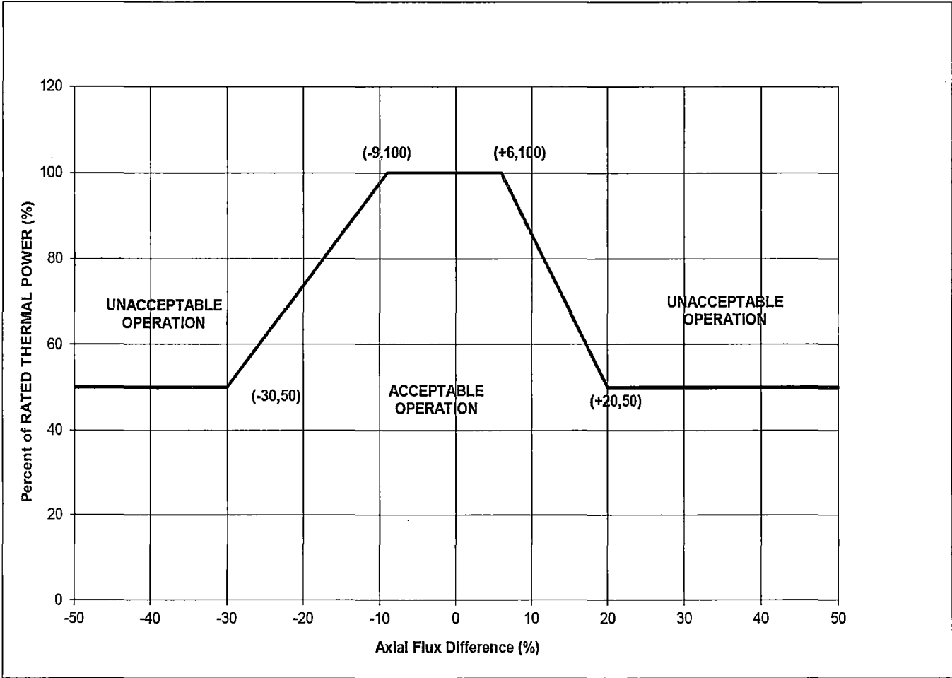
Axial Flux Difference as a Function of Rated Thermal Power Turkey Point Unit 4 Cycle 30
