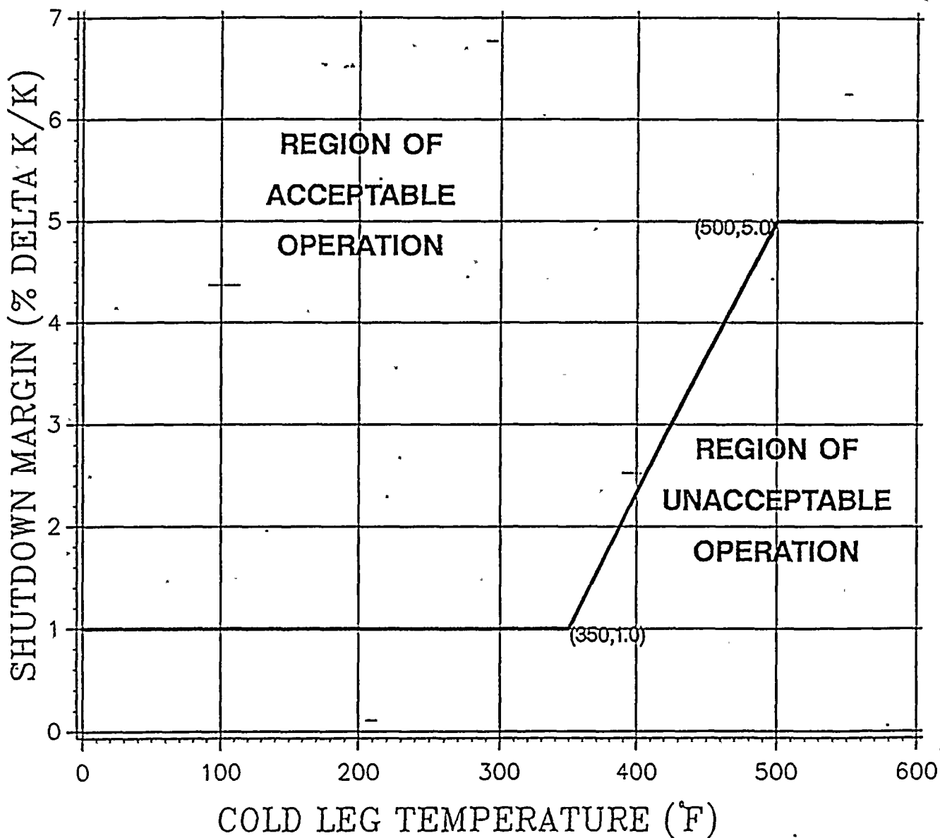
FIGURE 3.1.1.1-1 SHUTDOWN MARGIN VERSUS COLD LEG TEMPERATURE REACTOR TRIP BREAKERS OPEN
