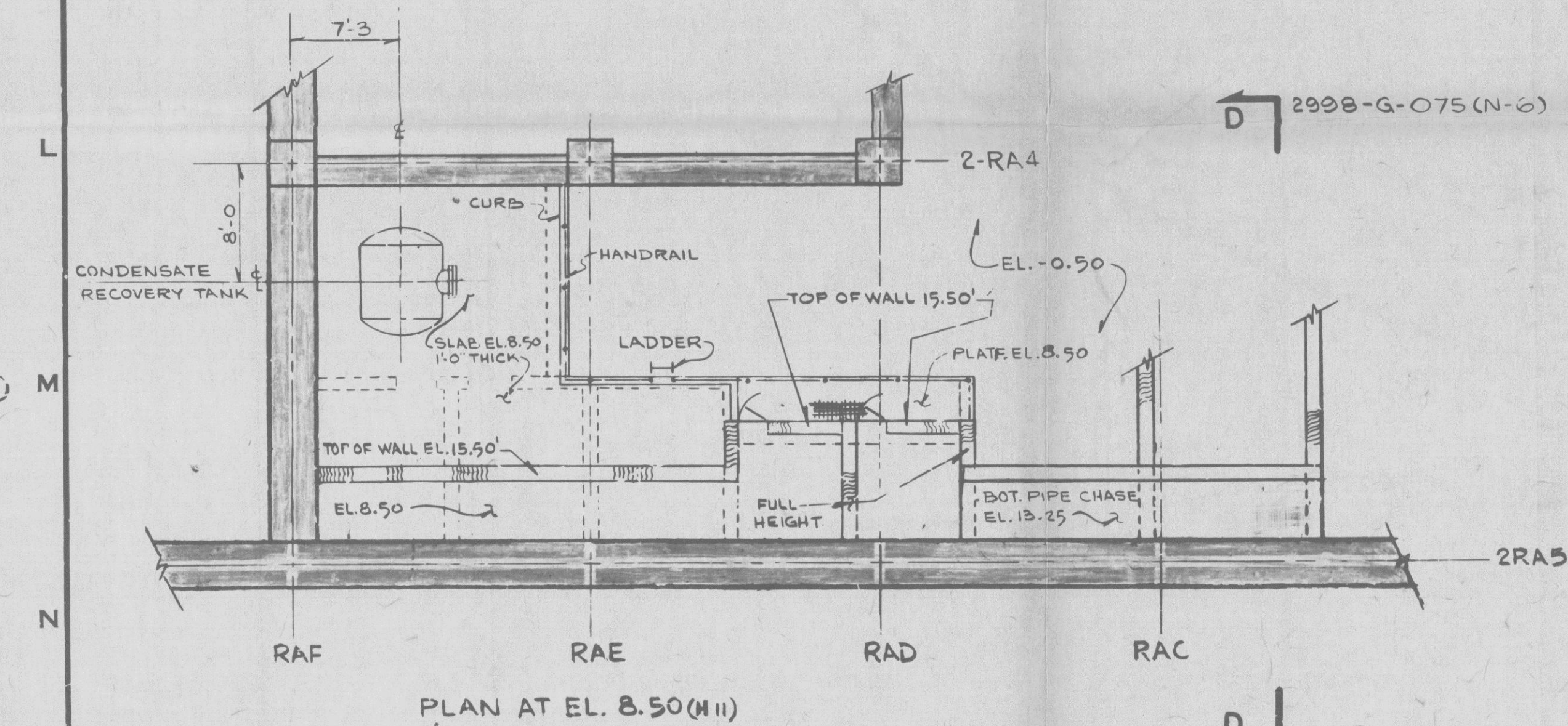
PLAN AT EL. 8.50' (H11)
