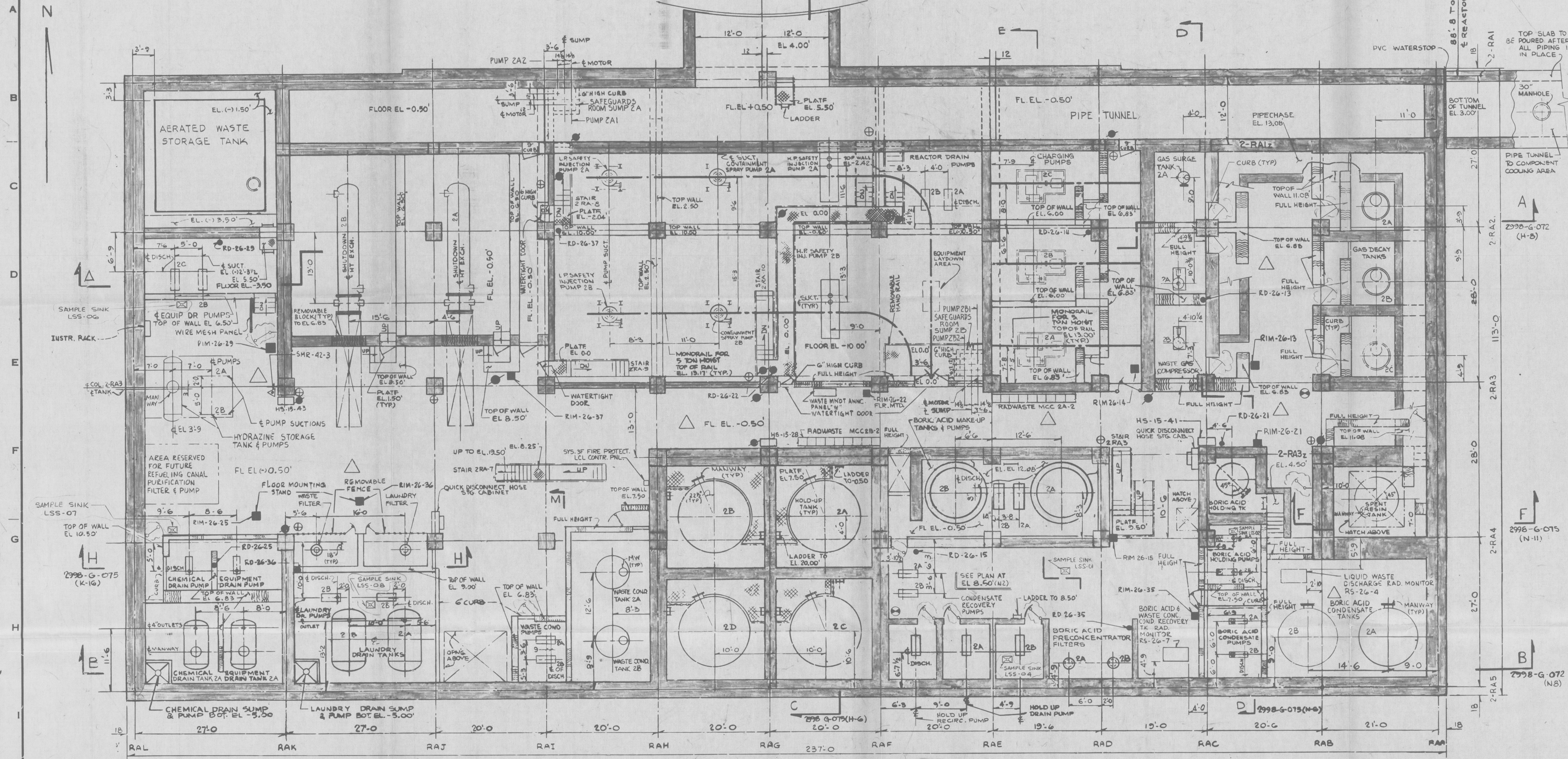
PLAN AT EL. -0.50'
