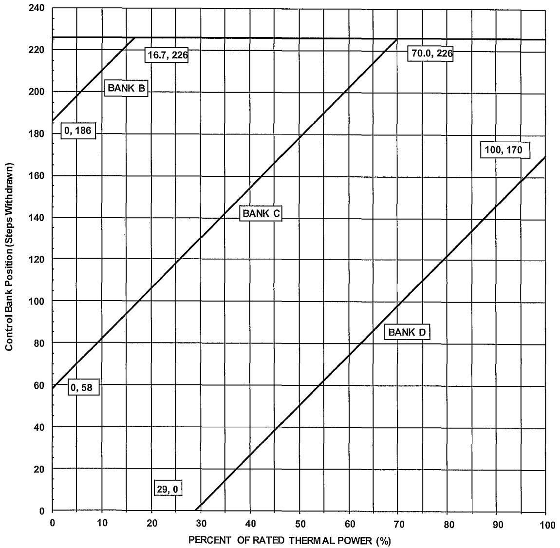
FIGURE 1 ROD BANK INSERTION LIMITS VS. THERMAL POWER
