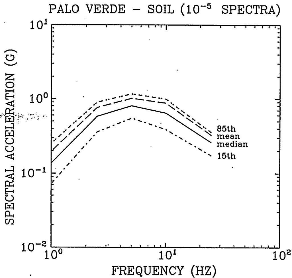
Figure 3-10. Mean, 15th-fractile, median, and 85th-fractile uniform seismic-hazard spectra for an annual exceedance frequency of 1 \times 10^{-5} ; Palo Verde site (Soil).
