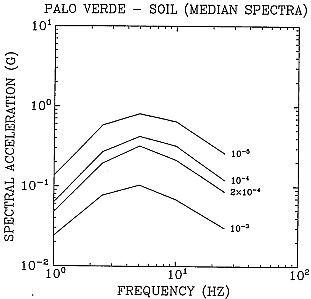
Figure 3-11. Median uniform seismic-hazard spectra for annual exceedance frequencies of 1 \times 10^{-3} , 2 \times 10^{-4} , 1 \times 10^{-4} , and 1 \times 10^{-5} ; Palo Verde site (Soil).
