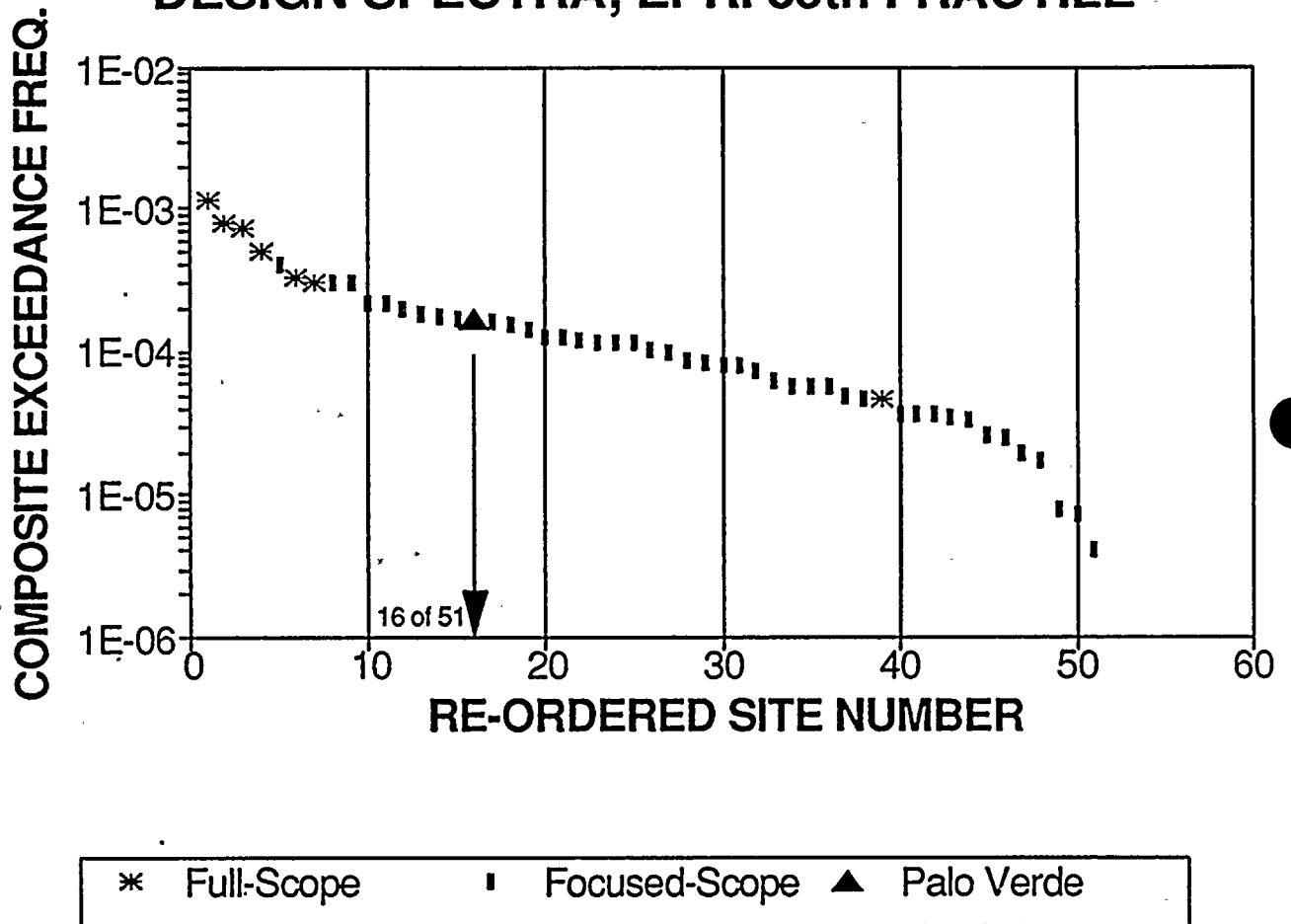
Figure 5-9. 85th-fractile composite probabilities of exceeding the seismic design-basis spectrum: comparison of results for the the Palo Verde site with similar results for 50 full-scope and focused-scope 0.3g plants in the central and eastern U.S.
