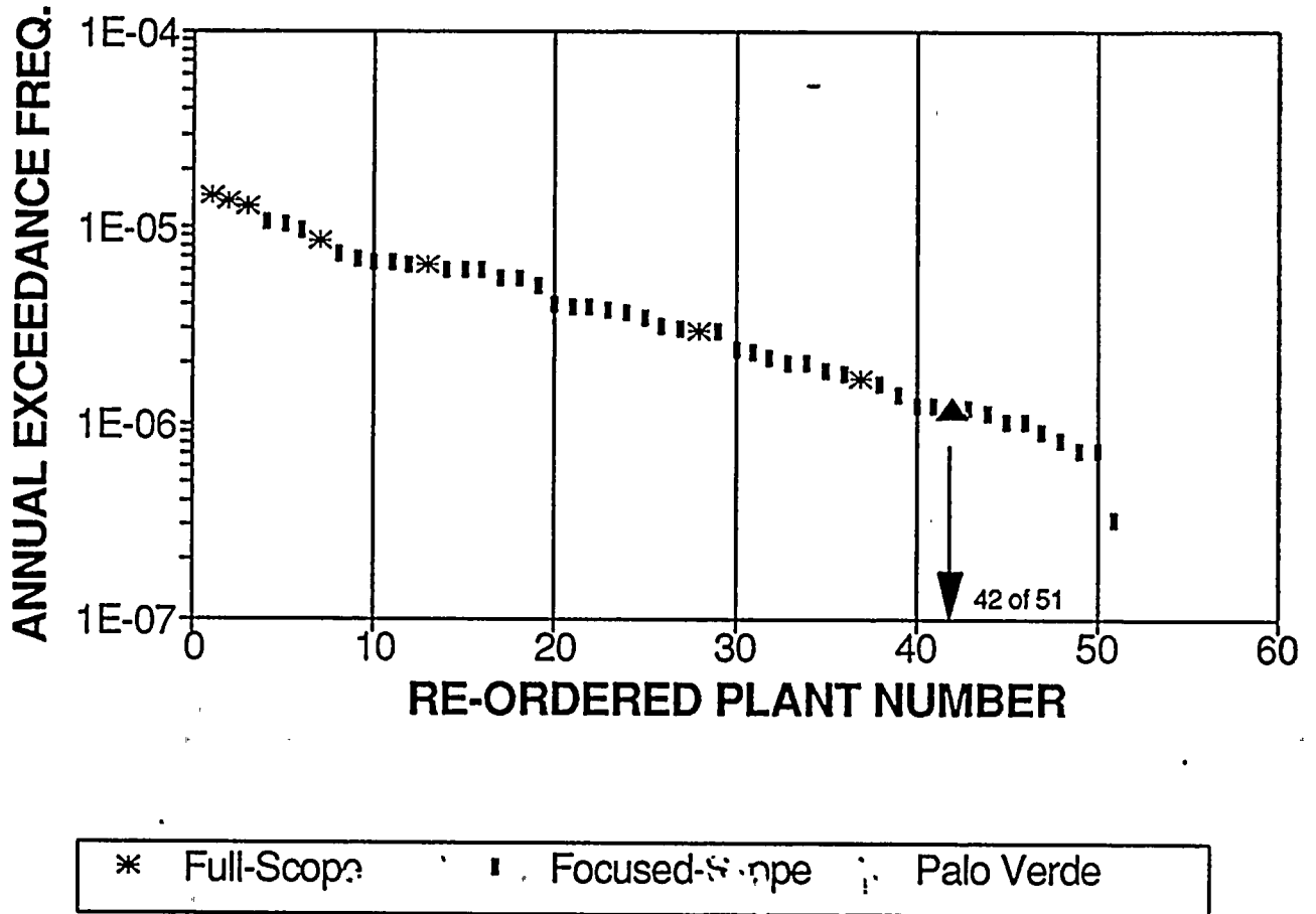
Figure B-4. Mean probability of exceeding a peak ground acceleration of 0.5g: comparison of results for the Palo Verde site with similar results for 50 full-scope and focused-scope 0.3g plants in the central and eastern U.S.
