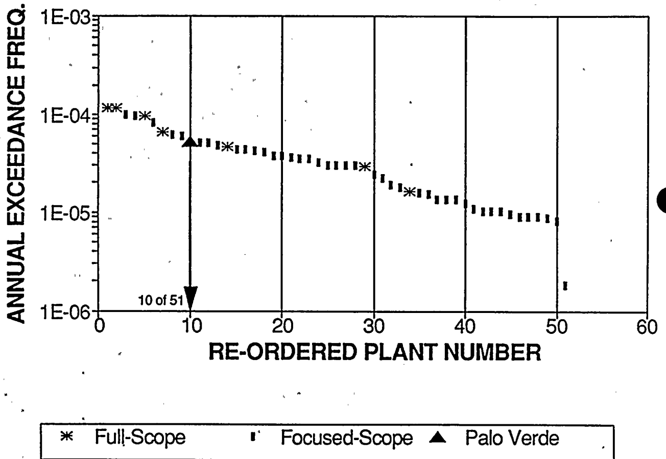
Figure B-3. 85th-fractile probability of exceeding a peak ground acceleration of 0.3g: comparison of results for the Palo Verde site with similar results for 50 full-scope and focused-scope 0.3g plants in the central and eastern U.S.
