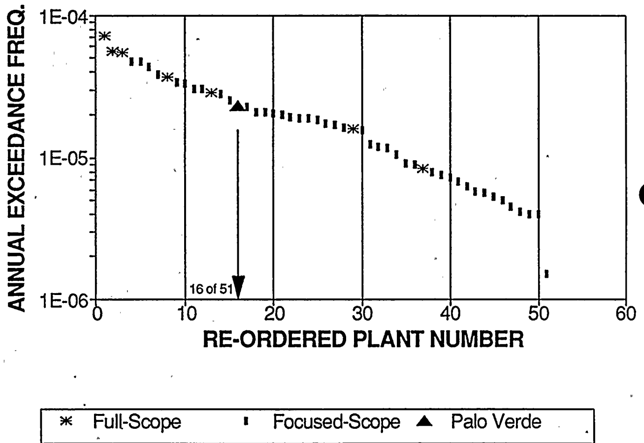
Figure B-1. Mean probability of exceeding a peak ground acceleration of 0.3g: comparison of results for the Palo Verde site with similar results for 50 full-scope and focused-scope 0.3g plants in the central and eastern U.S.
