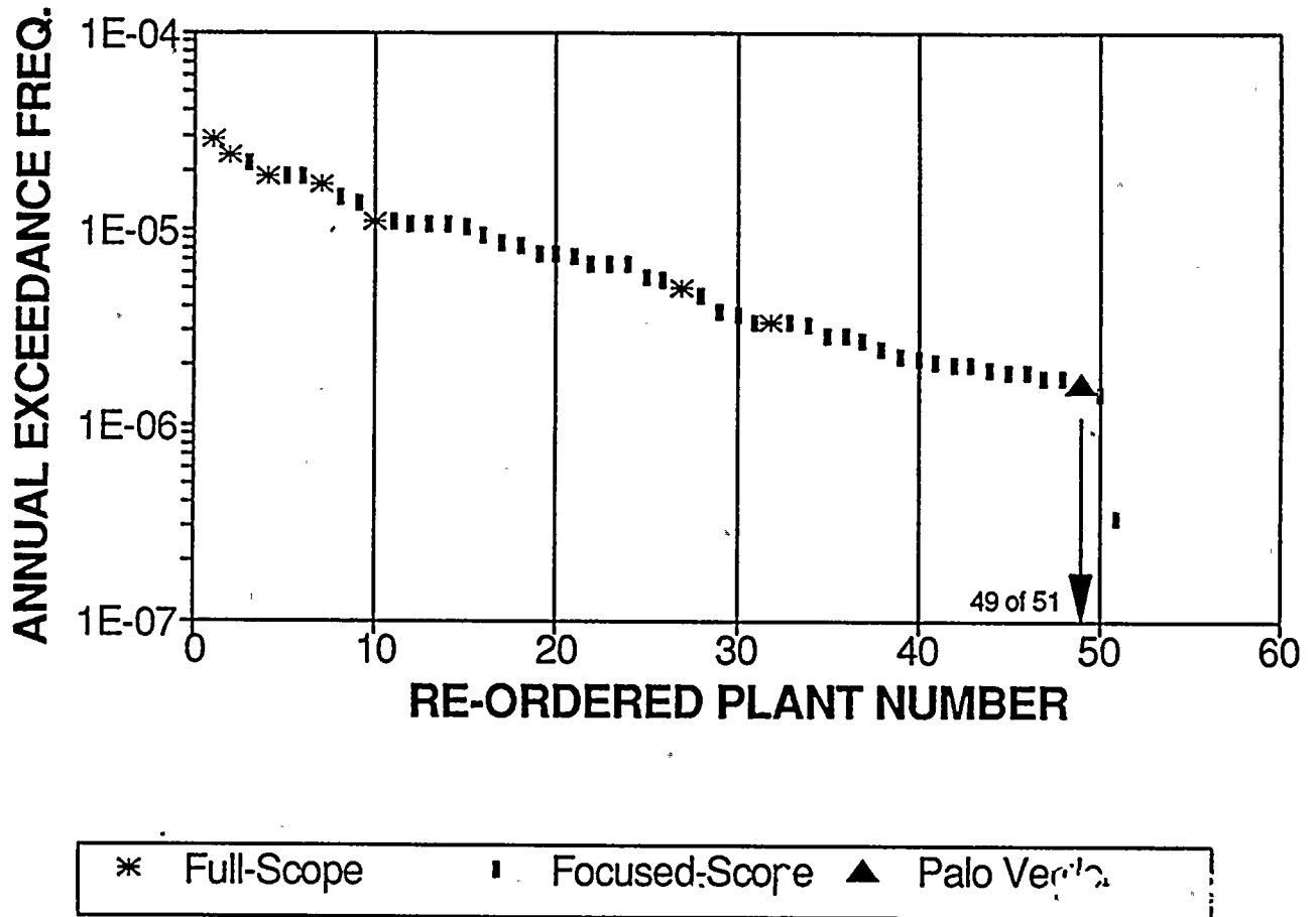
Figure B-6. 85th-fractile probability of exceeding a peak ground acceleration of 0.5g: comparison of results for the Palo Verde site with similar results for 50 full-scope and focused-scope 0.3g plants in the central and eastern U.S.
