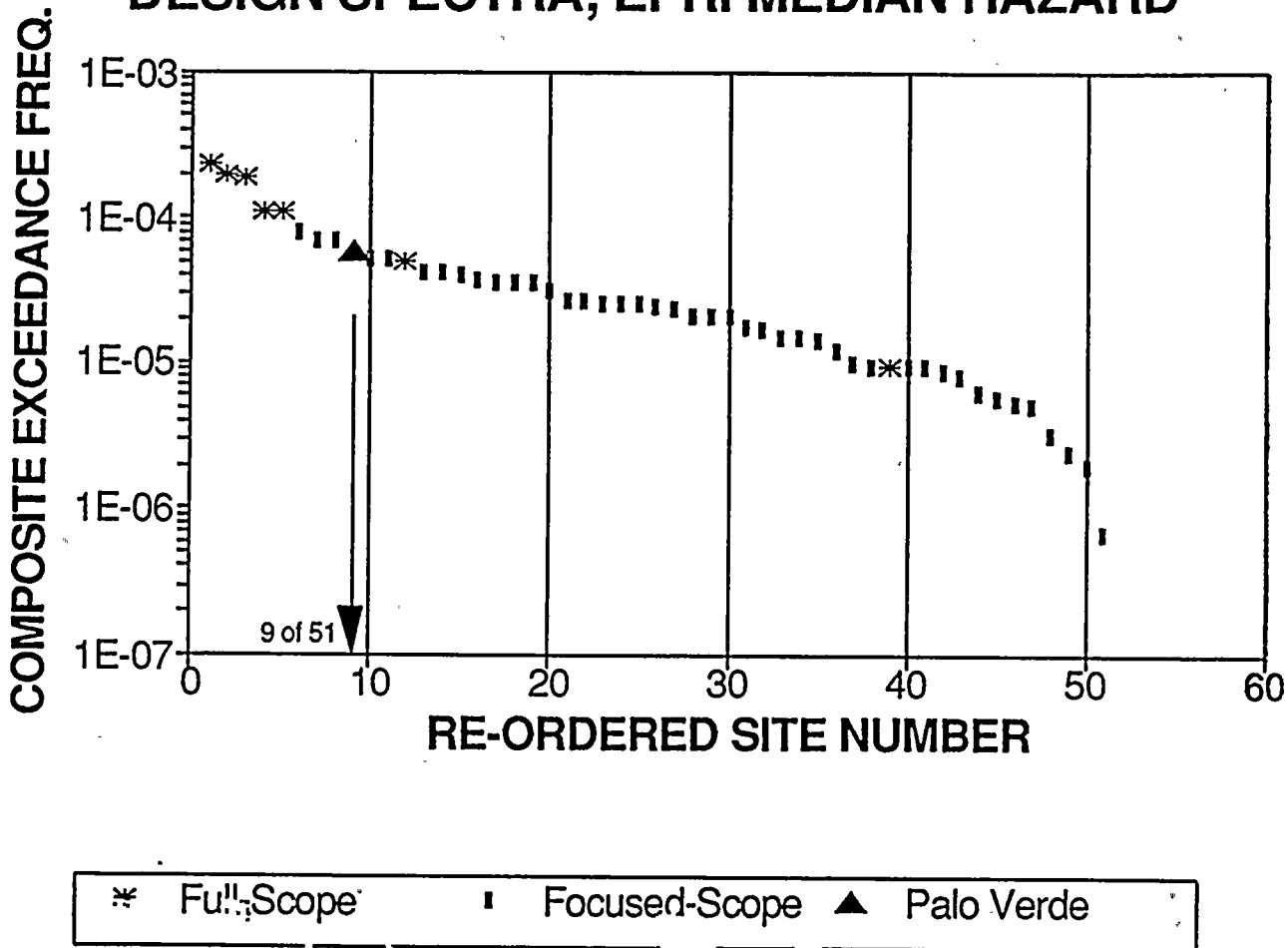
Figure 5-8. Median composite probabilities of exceeding the seismic design-basis spectrum: comparison of results for the the Palo Verde site with similar results for 50 full-scope and focused-scope 0.3g plants in the central and eastern U.S.
