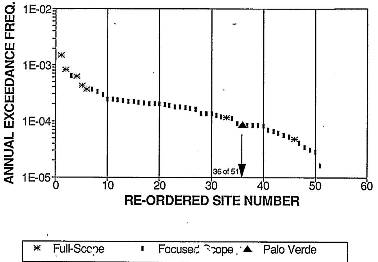
Figure C-3. 85th-fractile probability of exceeding the seismic design-basis PGA: comparison of results for the Palo Verde site with similar results for 50 full-scope and focused-scope 0.3g plants in the central and eastern U.S.
