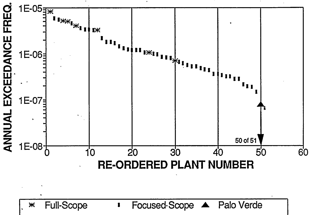
Figure B-5. Median probability of exceeding a peak ground acceleration of 0.5g: comparison of results for the Palo Verde site with similar results for 50 full-scope and focused-scope 0.3g plants in the central and eastern U.S.
