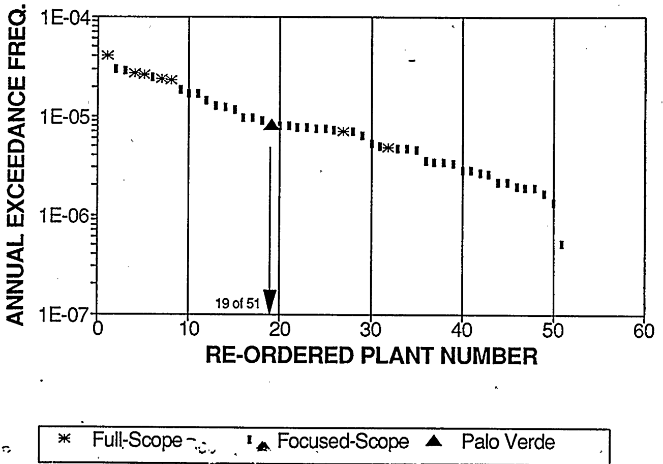
Figure B-2. Median probability of exceeding a peak ground acceleration of 0.3g: comparison of results for the Palo Verde site with similar results for 50 full-scope and focused-scope 0.3g plants in the central and eastern U.S.
