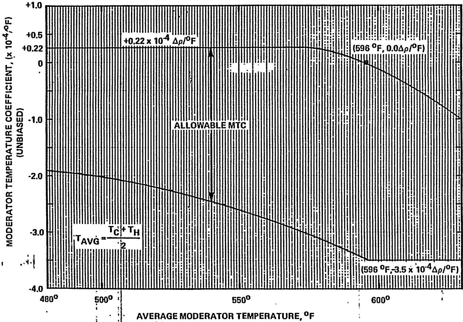
FIGURE 3.1-1 ALLOWABLE MTC MODES 1 AND 2 PALO VERDE UNIT 2 CYCLE 1
