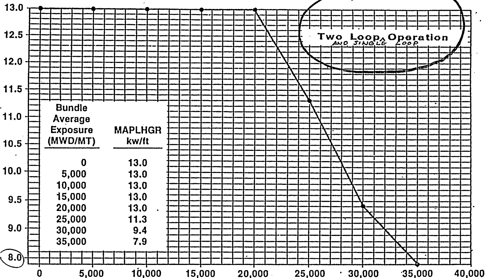
Bundle Average Exposure (MWD/MT) ANF 8x8 Reload Fuel Maximum Average Planar Linear Heat Generation Rate (MAPLHGR) Versus Bundle Average Exposure
