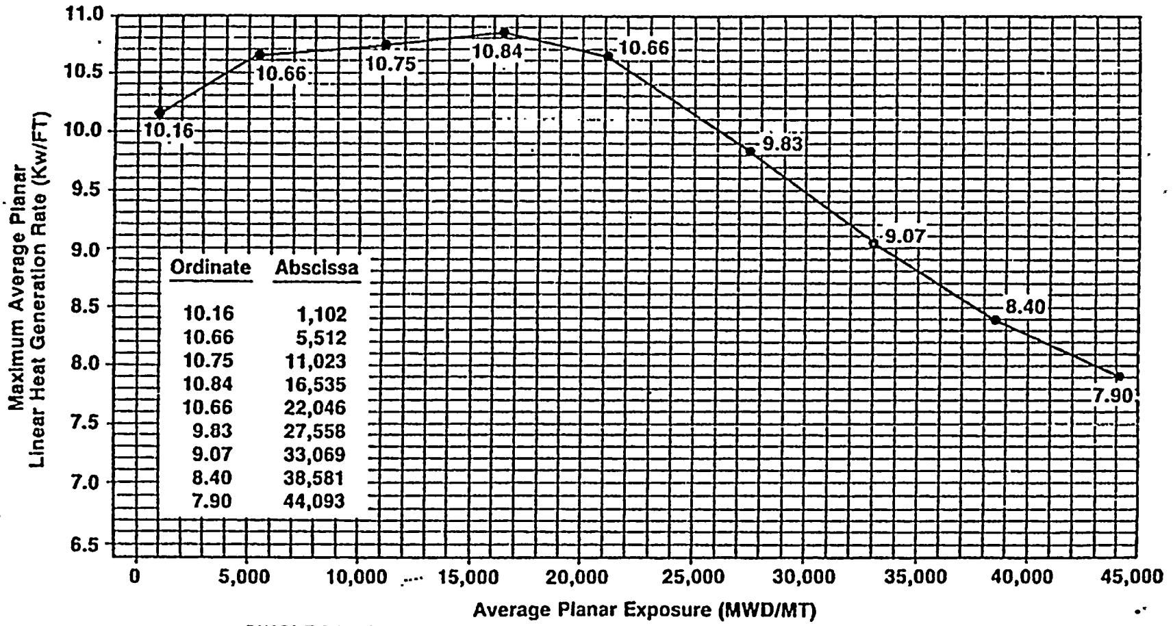
Maximum Average Planar Linear Heat Generation Rate (MAPLHGR) Versus Average Planar Exposure Initial Core Fuel Type 8CR183
