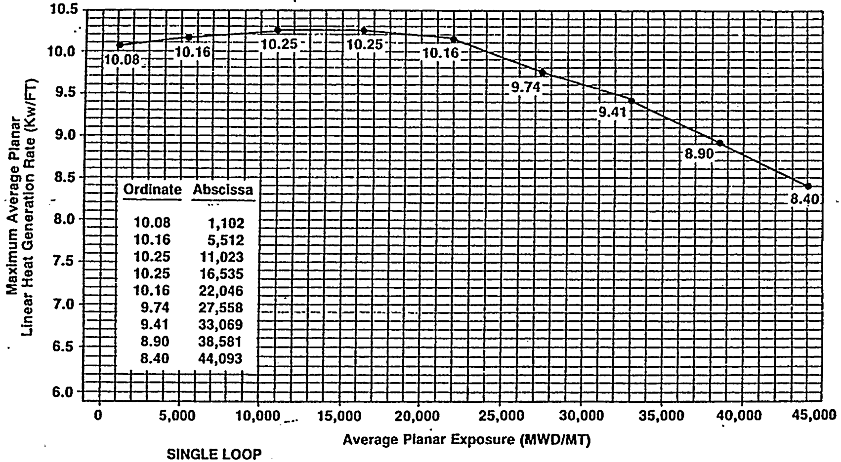
SINGLE LOOP Maximum Average Planar Linear Heat Generation Rate (MAPLHGR) Versus Average Planar Exposure Initial Core Fuel Type 8CR233 Figure 3.2.1-5
