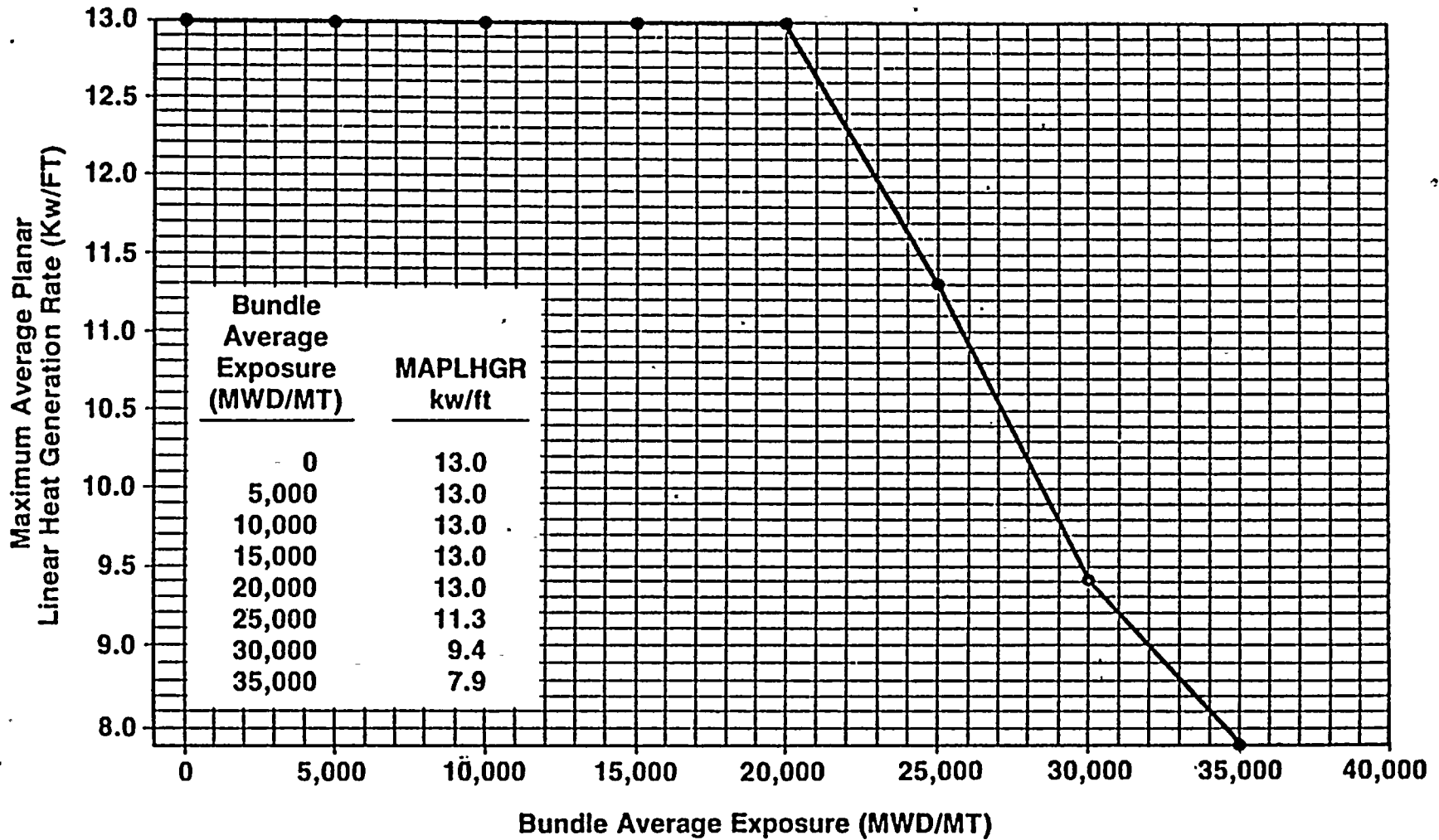
Maximum Average Planar Linear Heat Generation Rate (MAPLHGR) Versus Bundle Average Exposure ENC XN-1 Fuel Figure 3.2.1-3
