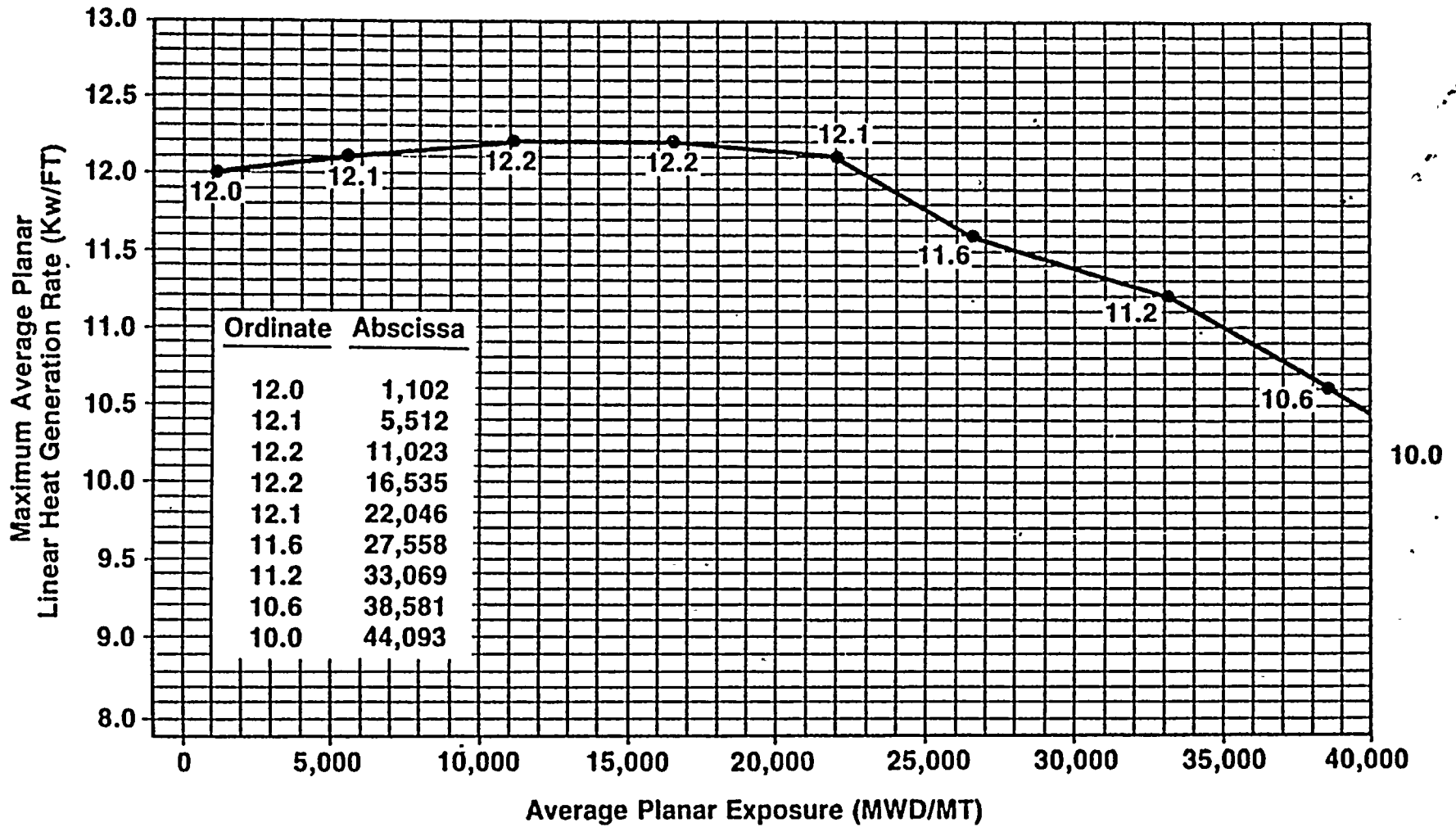
Maximum Average Planar Linear Heat Generation Rate (MAPLHGR) Versus Average Planar Exposure Initial Core Fuel Type 8CR233 Figure 3.2.1-2
