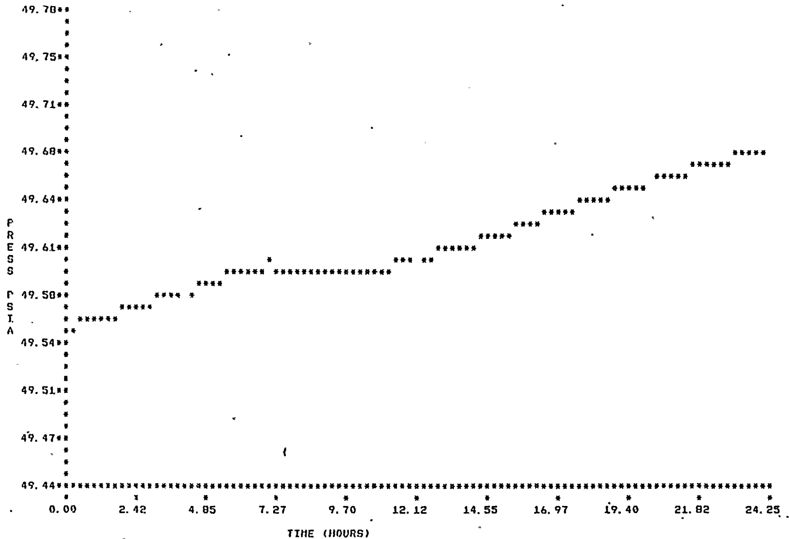
FIGURE VII.3 PCTLR1 AVERAGED ABSOLUTE PRESSURE VS TIME
