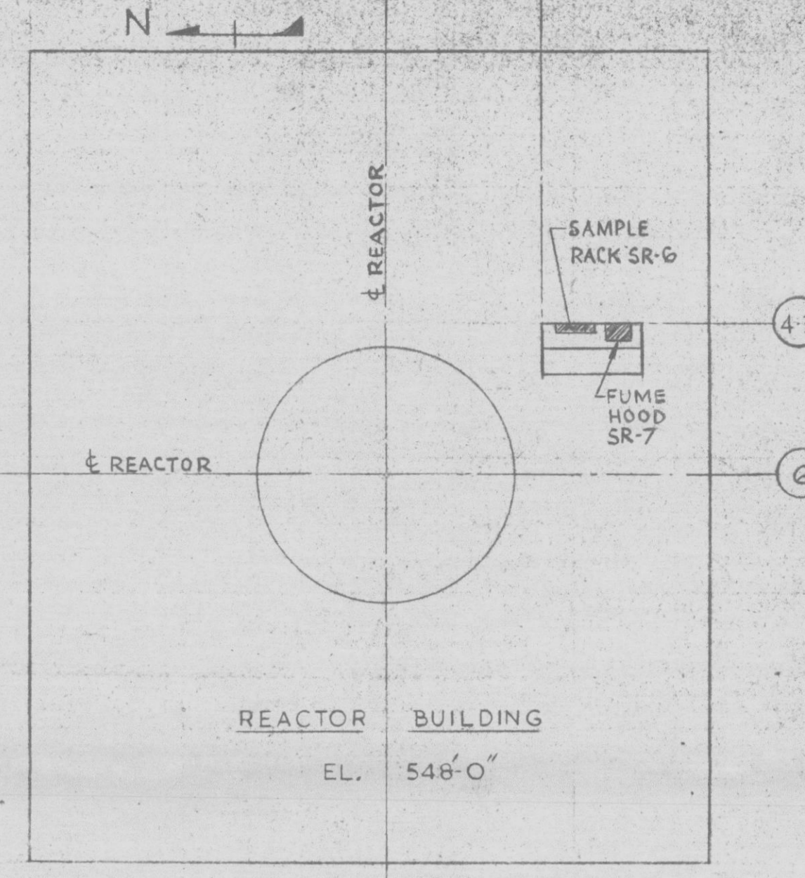
ENLARGED PLAN OF REACTOR BUILDING SHOWING LOCATION OF SAMPLE RACK SR-6 AND FUME HOOD SR-7.
