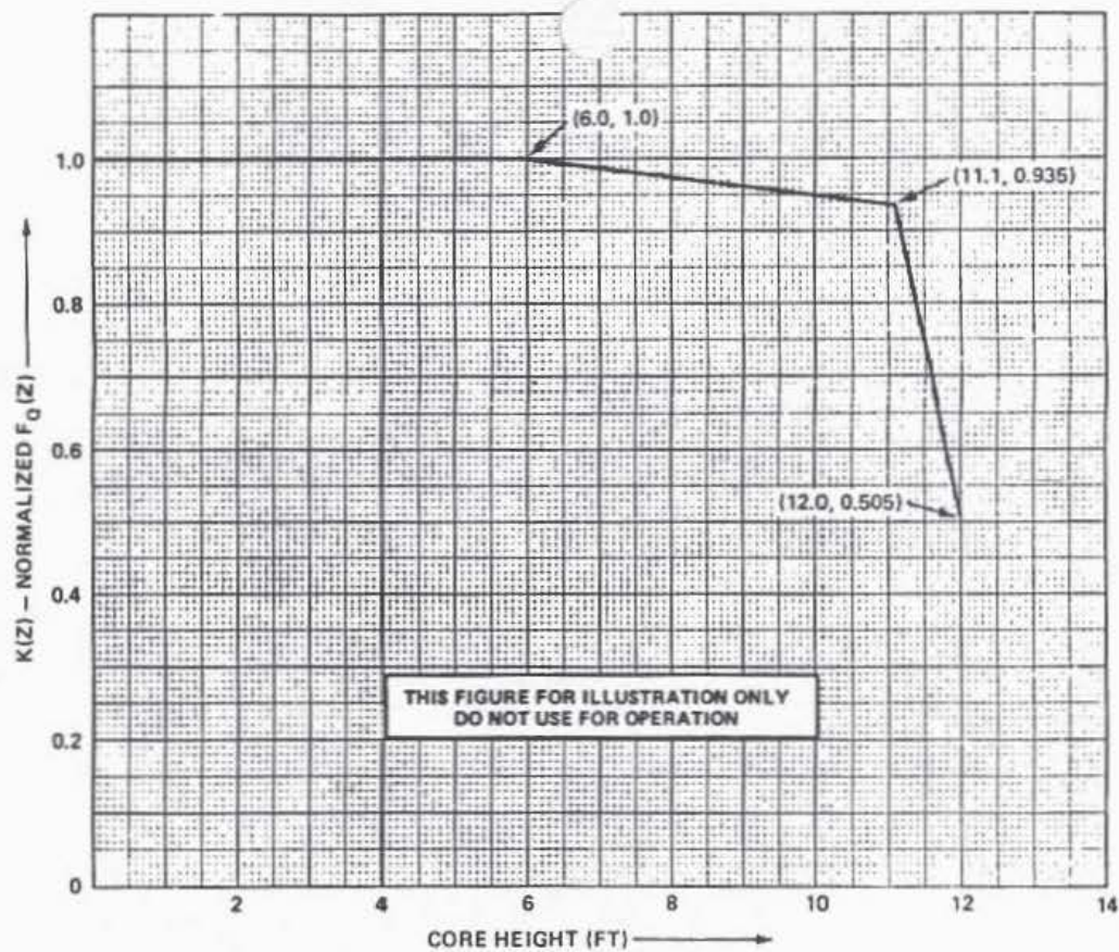
FIGURE 3.2-2 K(Z) - \text{NORMALIZED } F_O(Z) AS A FUNCTION OF CORE HEIGHT
