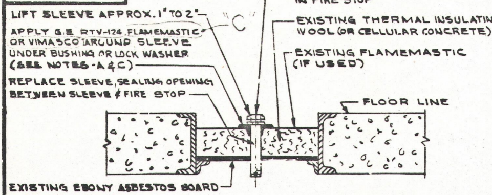
DETAIL 1 SLEEVE THRU FIRE STOP AT BASE OF CONTROL BOARD
