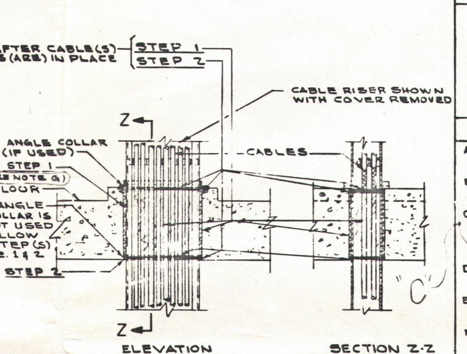
DETAIL 6 CRACK IN EXISTING CELLULAR CONCRETE FIRE-STOP
