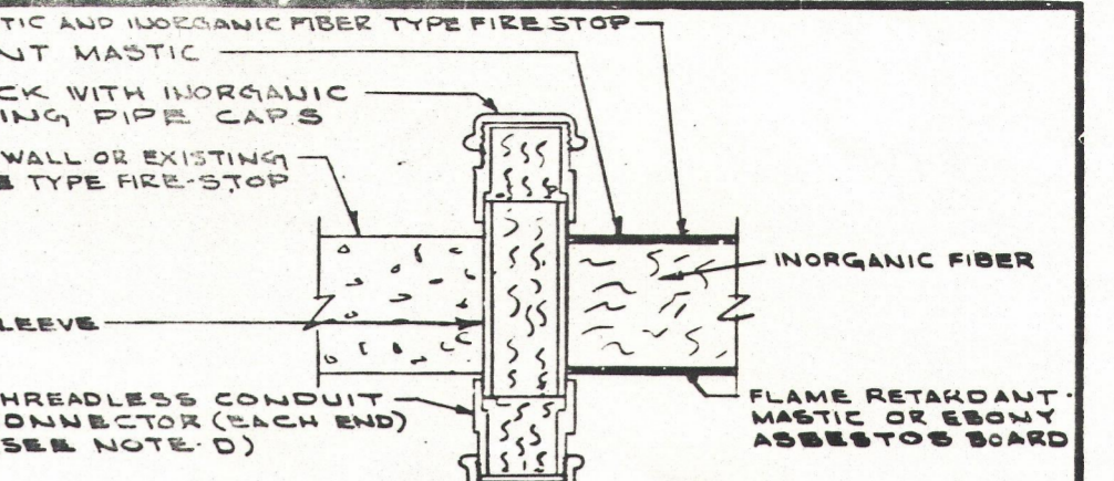
DETAIL 4 SLEEVES WITH THREADLESS ENDS
