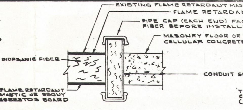
DETAIL 3 SLEEVES WITH THREADED ENDS
