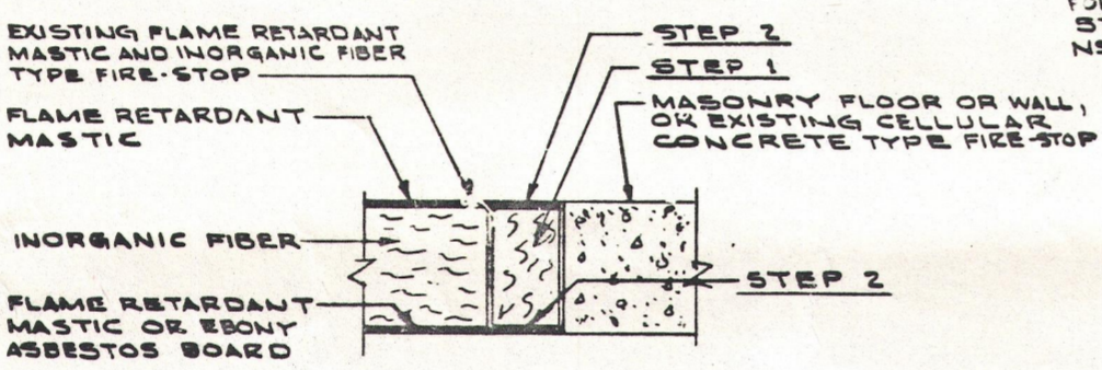
DETAIL 7 UNUSED CABLE OPENING WITH OR WITHOUT FLUSH CONDUIT SLEEVE
