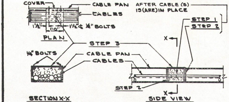
DETAIL 9 DIFFERENT ESS DIVISIONS IN SAME CABLE PAN
