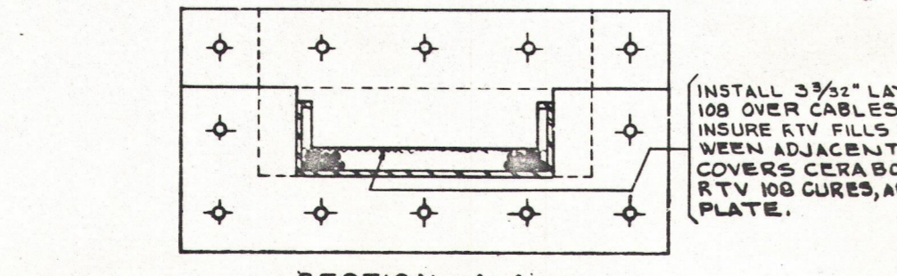
DETAIL 12 CABLE PAN THROUGH WALL
