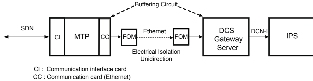
Figure 4-22 Data Communication from MTP to IPS
