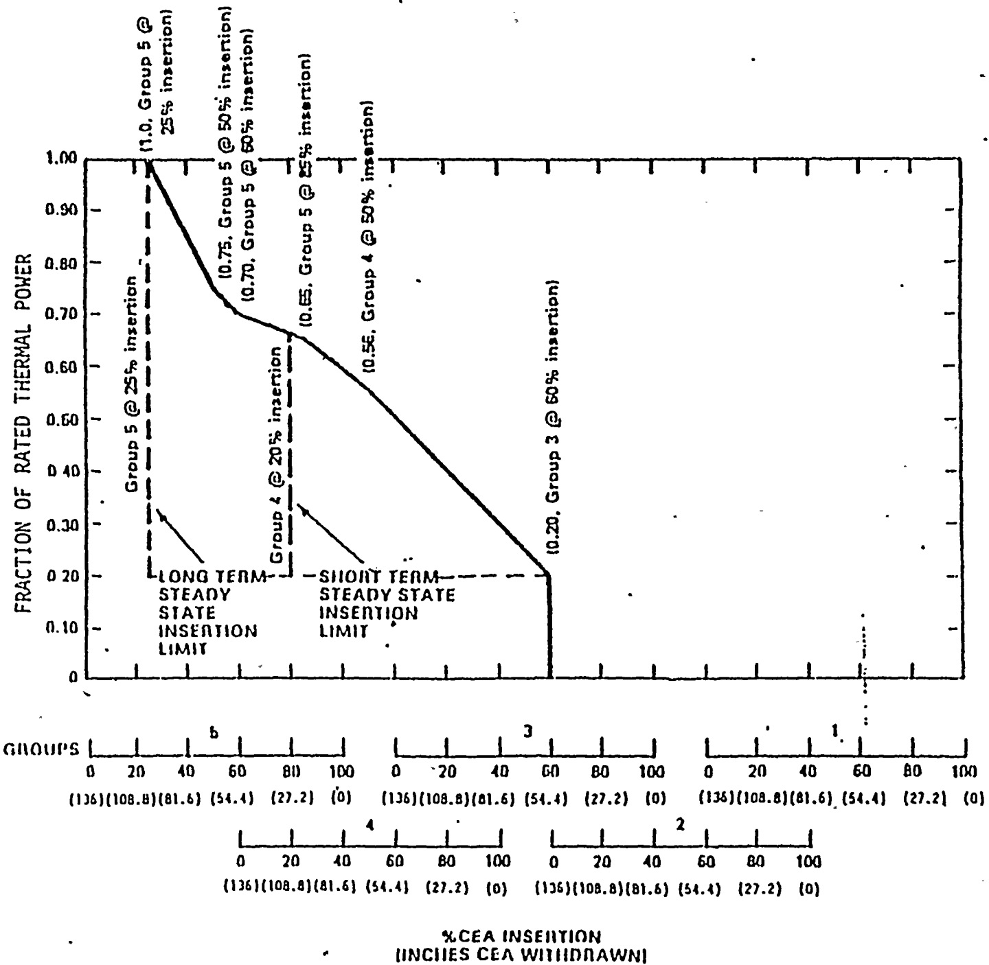
FIGURE 3.1-2 CEA Group Insertion Limits vs. THERMAL POWER
