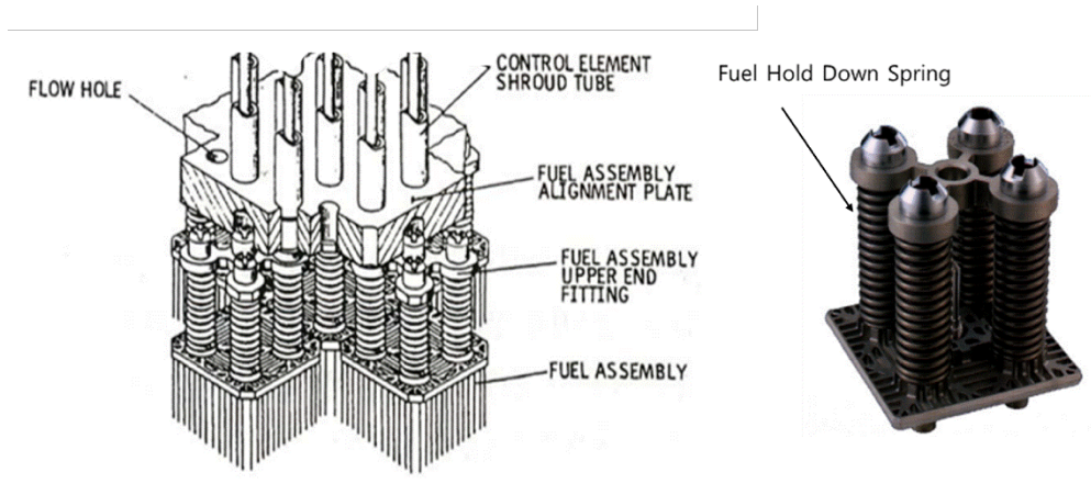
Figure 6-2 Design of CEA Guide Tube to Fuel Assembly
