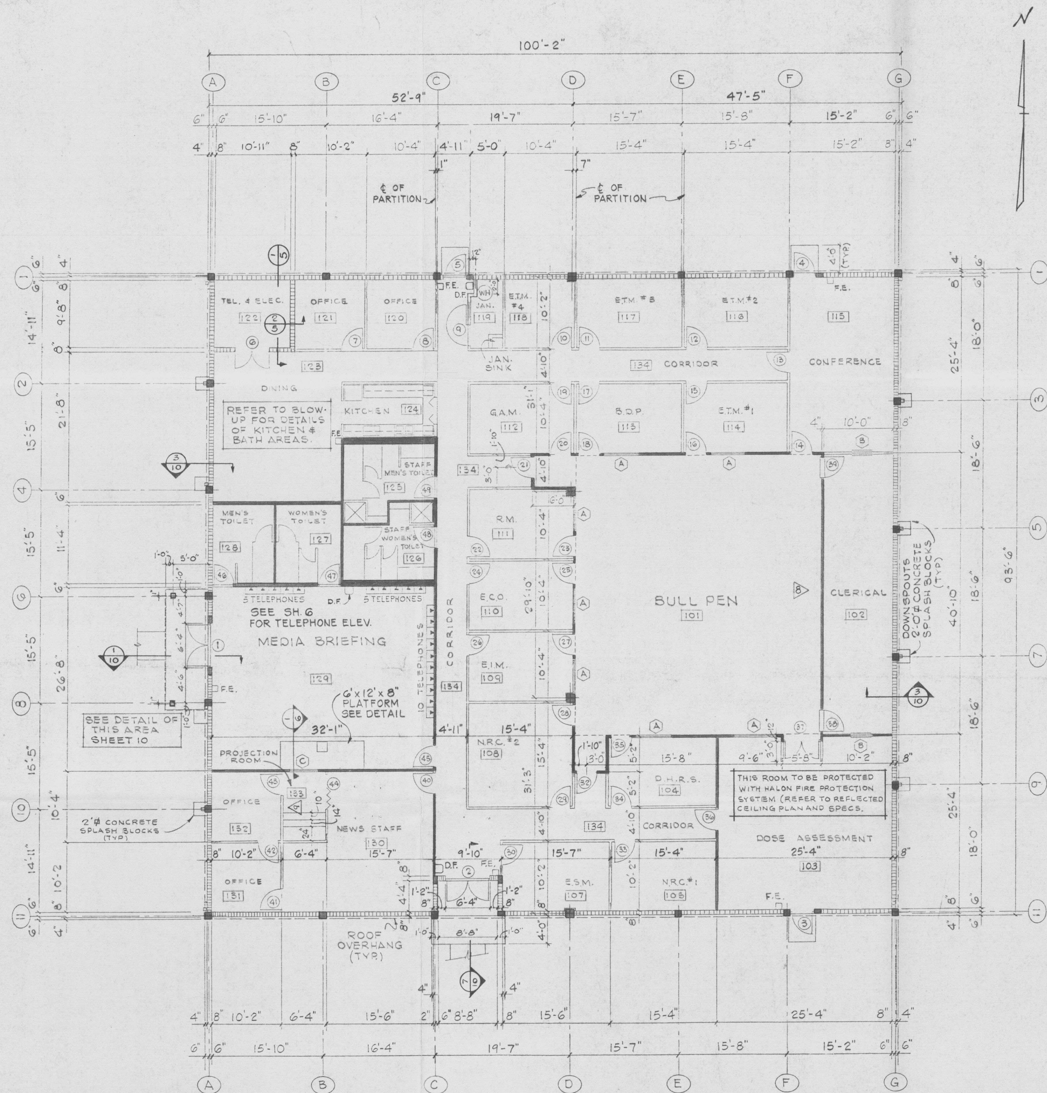
FLOOR PLAN
