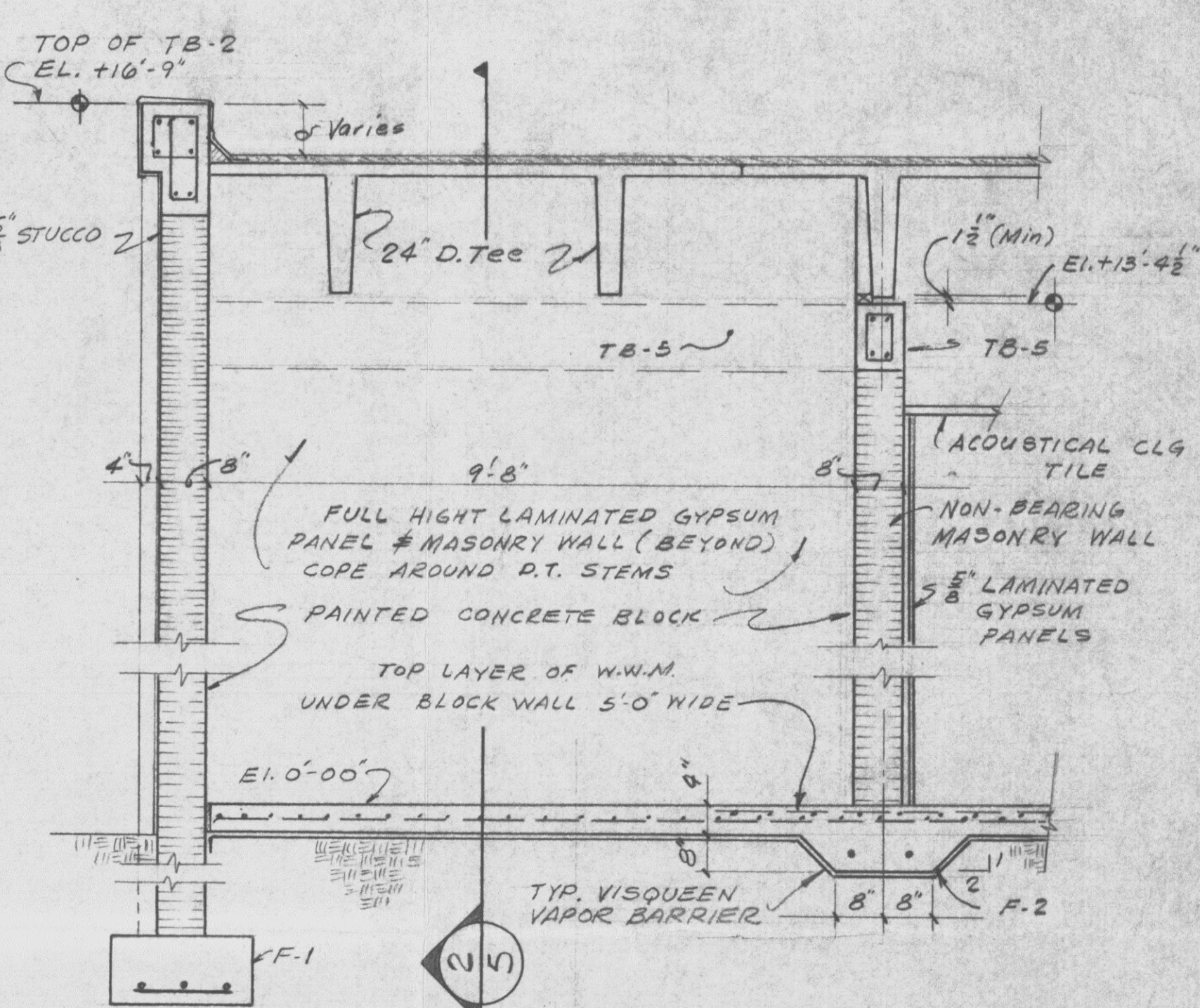
SECTION AT TELEPHONE AND ELECTRICAL ROOM
