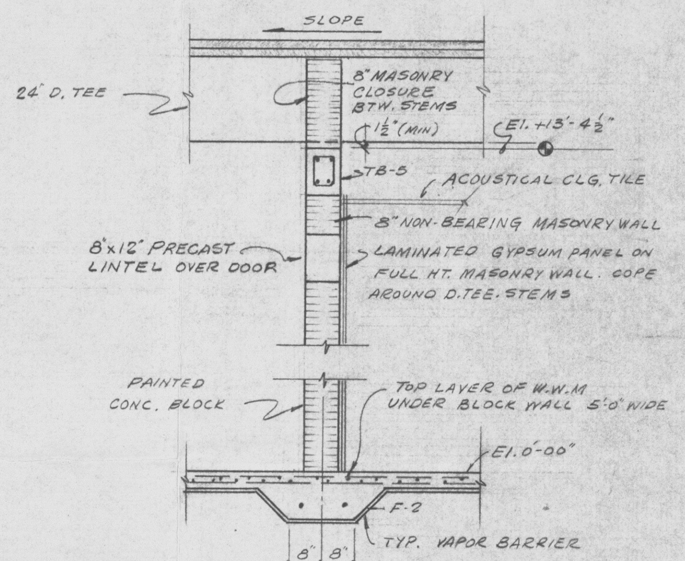
SECTION AT TELEPHONE AND ELECTRICAL ROOM
