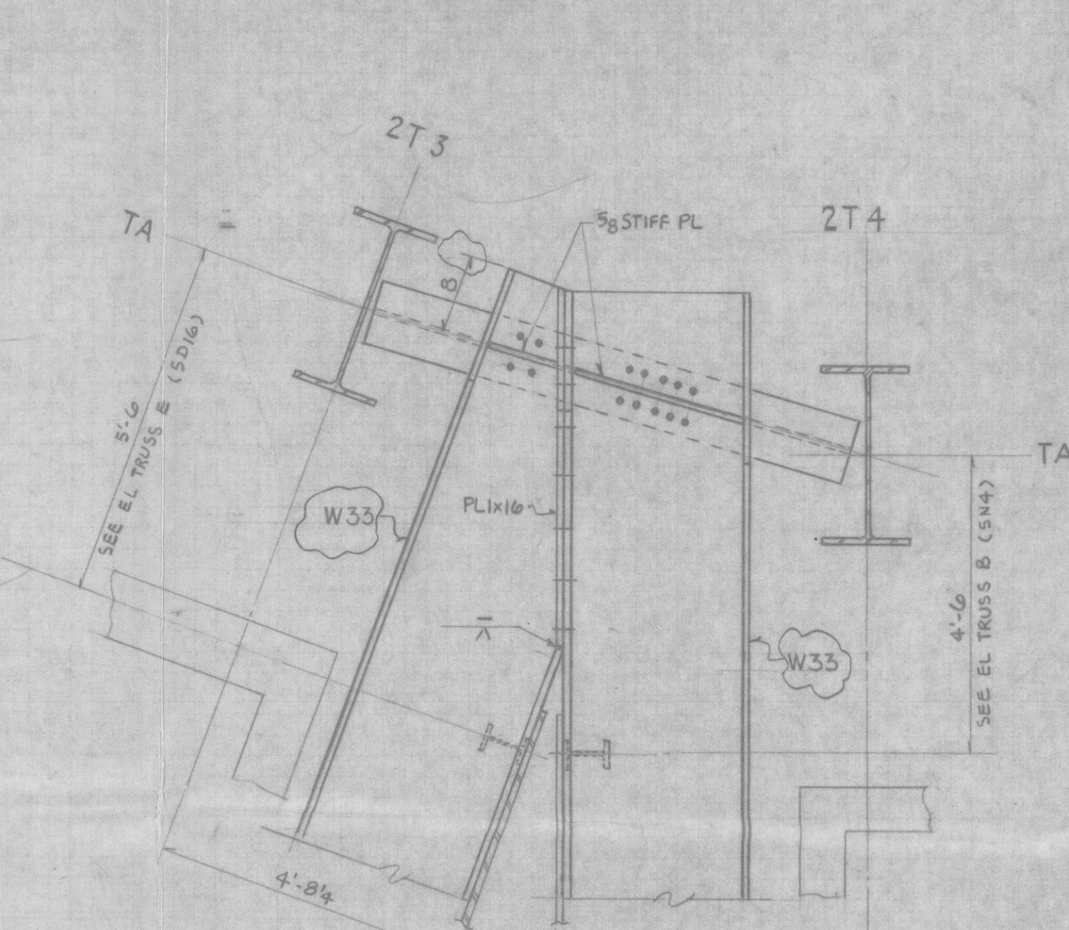
SECT GE (G14) SECT GG (G14)
