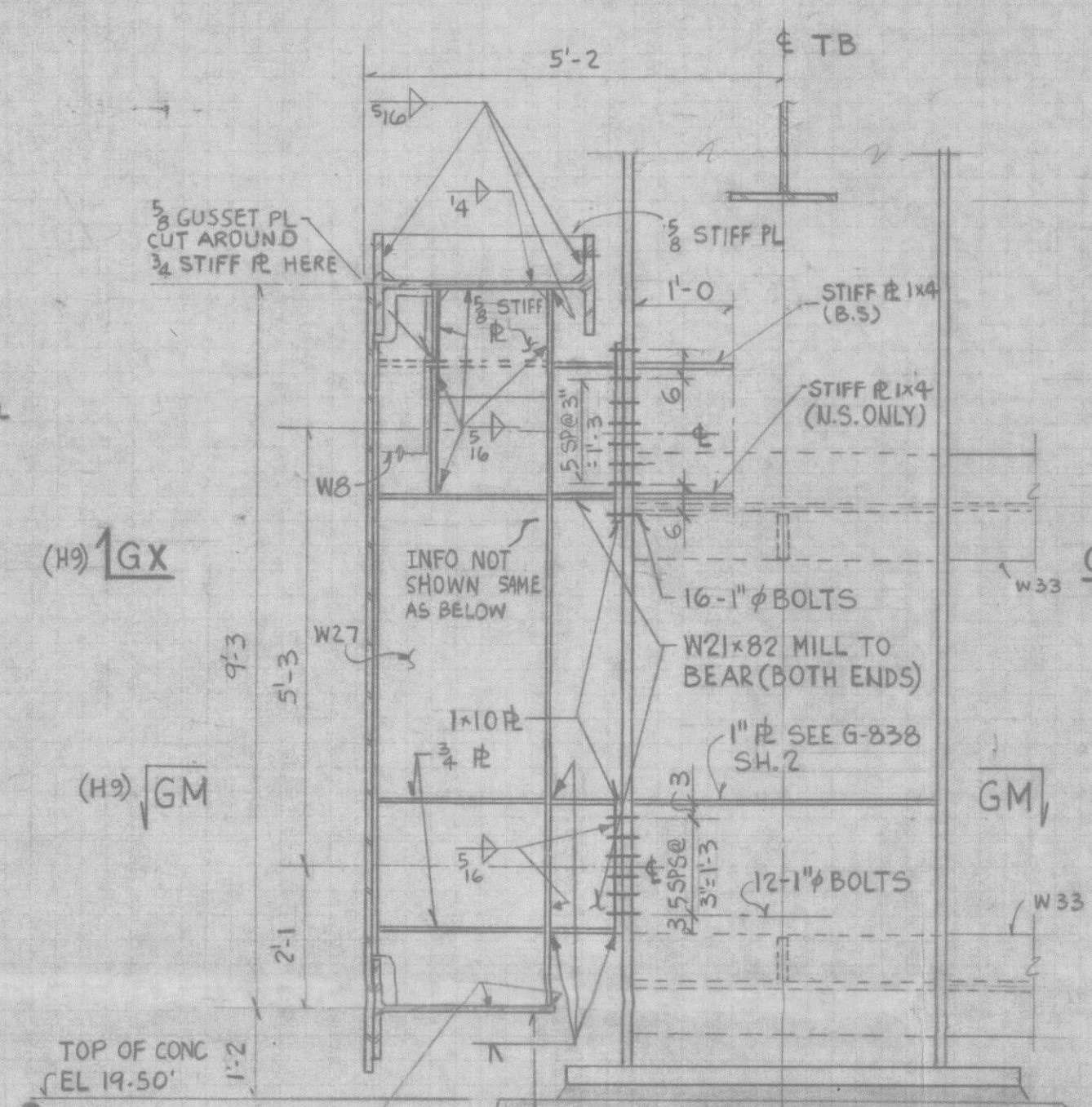
SECT GC (SE1, SG4, SF3, SF6)
