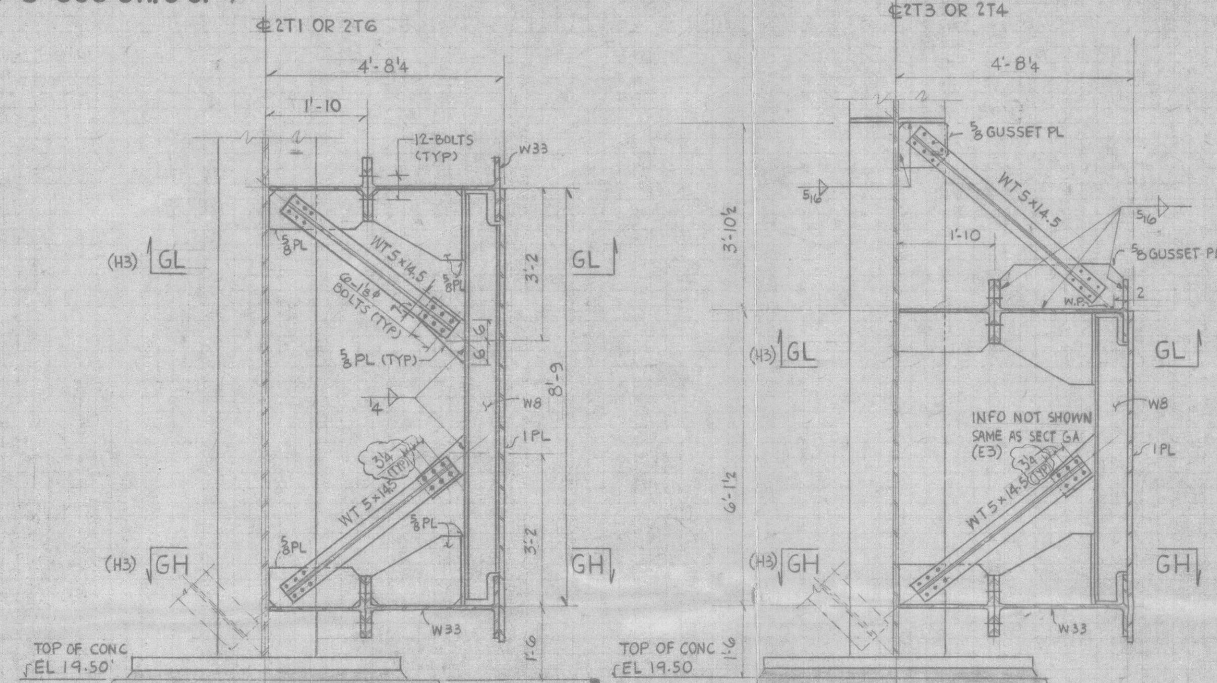
SECT GA (S82, SC4, SE1, SF6)
