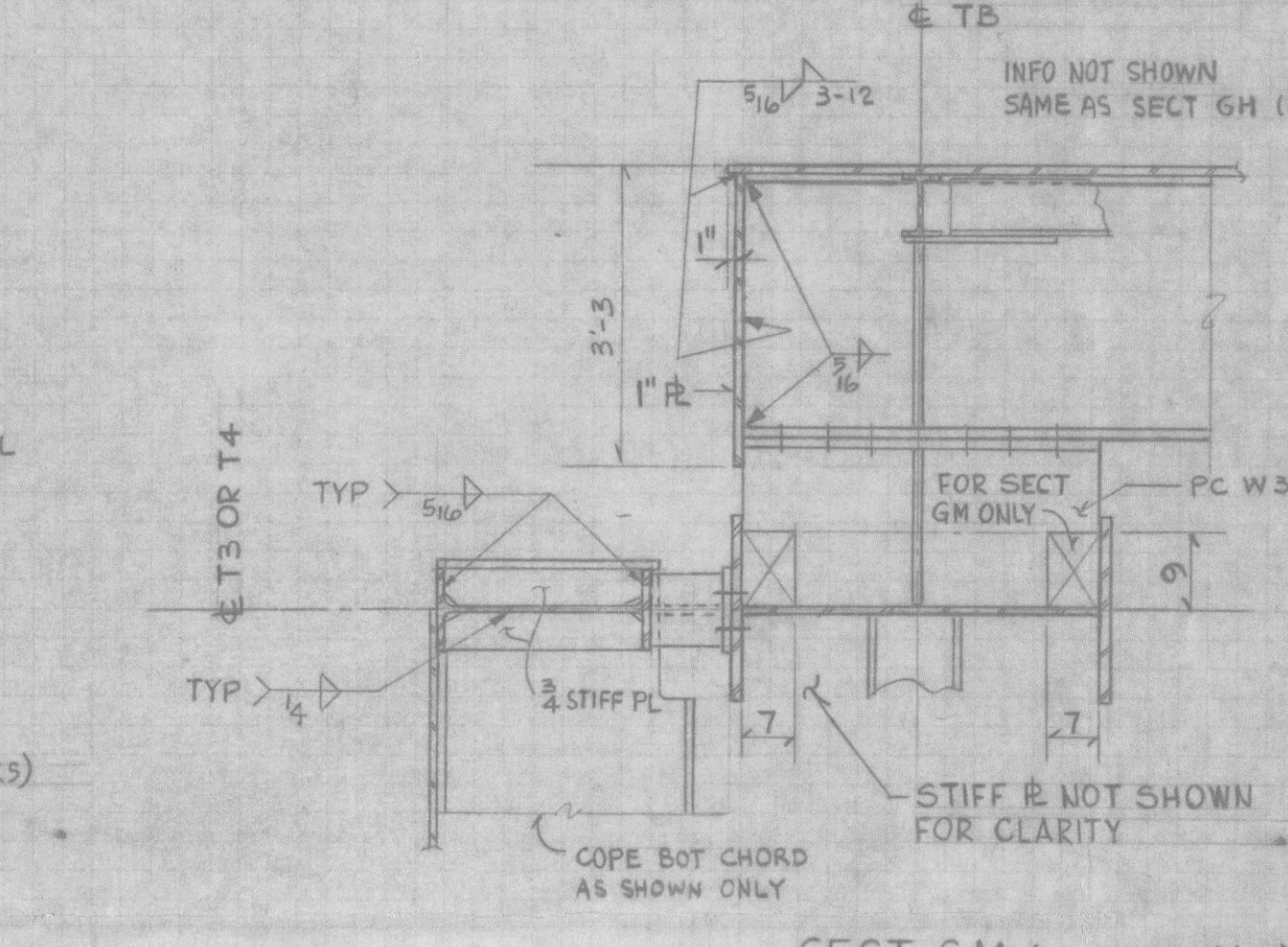
SECT GM (AS SHOWN) (C7) SECT GX (OPP HAND) (B7)
