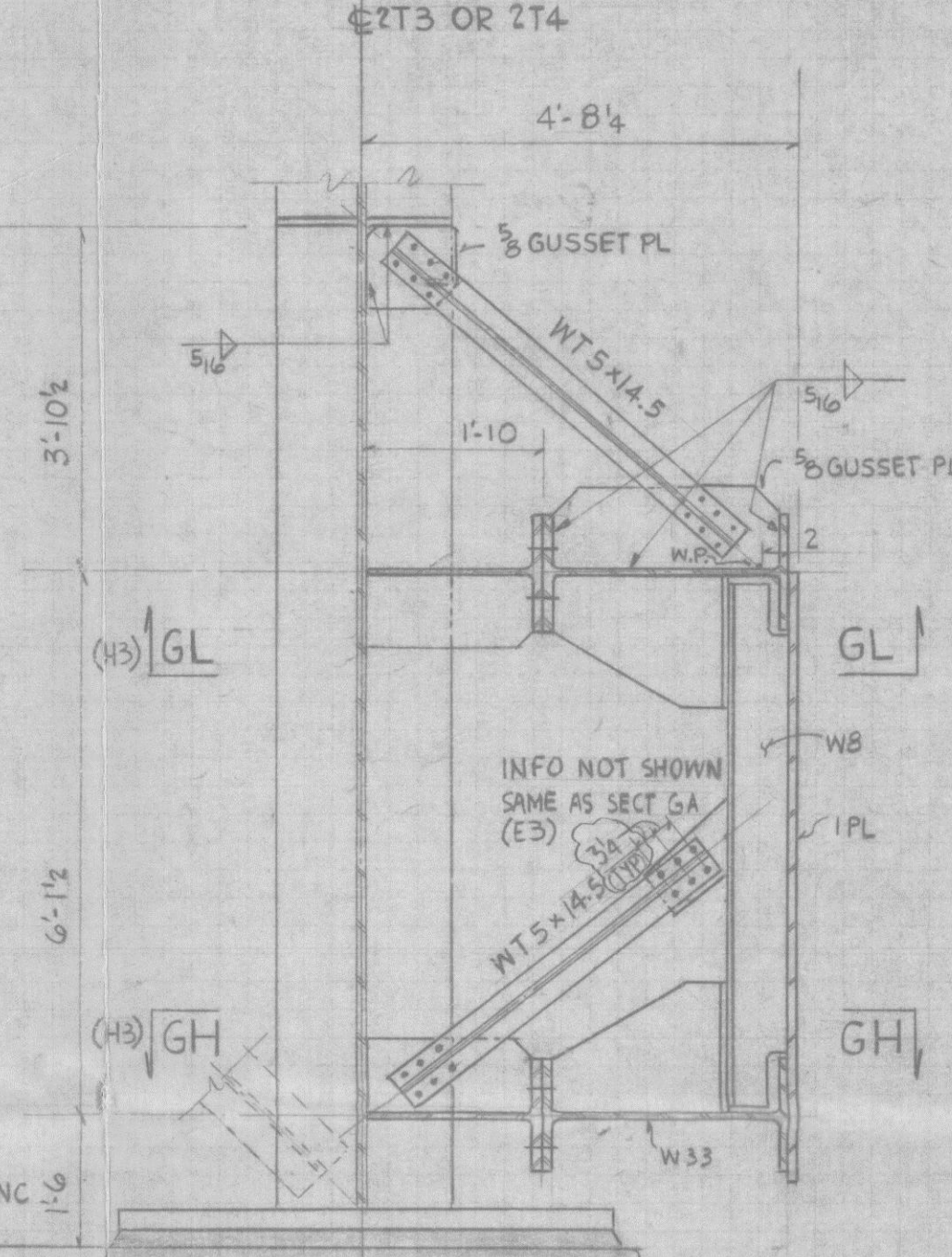
SECT GB (SG4, SF3)
