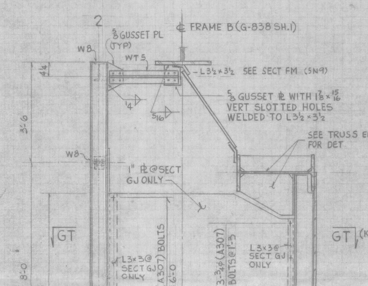
SECT GB (SG4, SF3)
