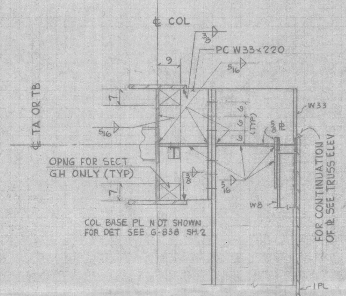
SECT GH (AS SHOWN) (D1, D5) SECT GL (OPP HAND) (B1, B5)
