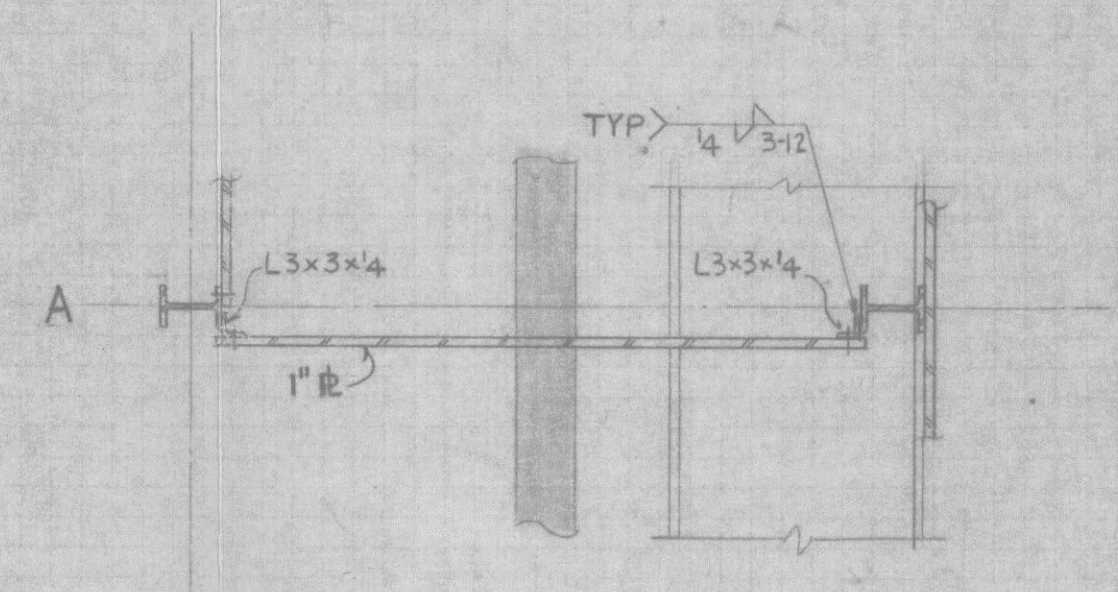
SECT GT (H7)
