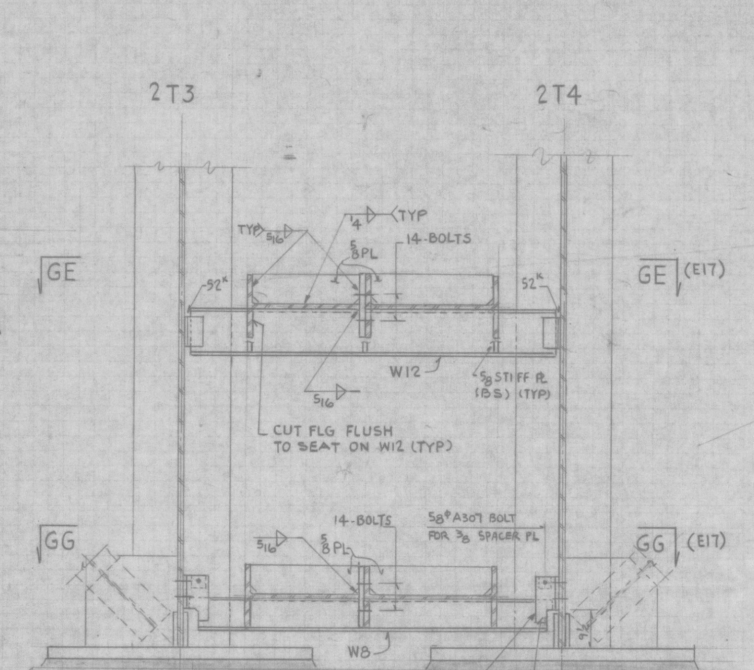
SECT GD (SC4)
