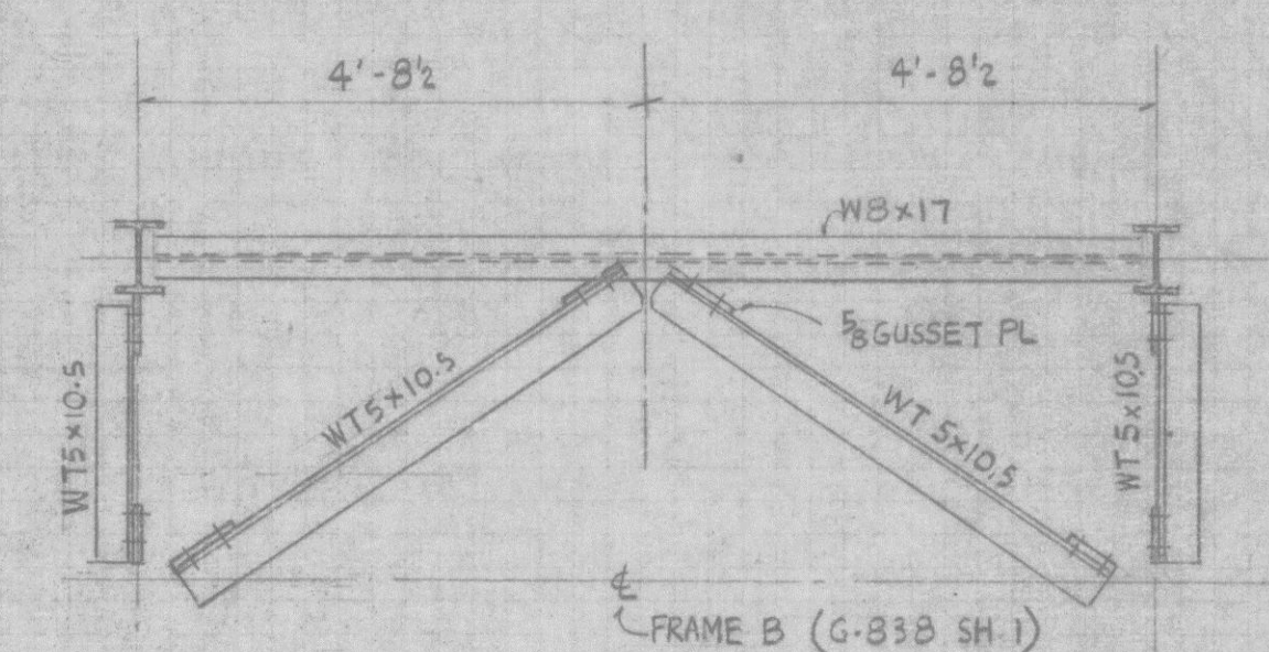
SECT GS (F18)
