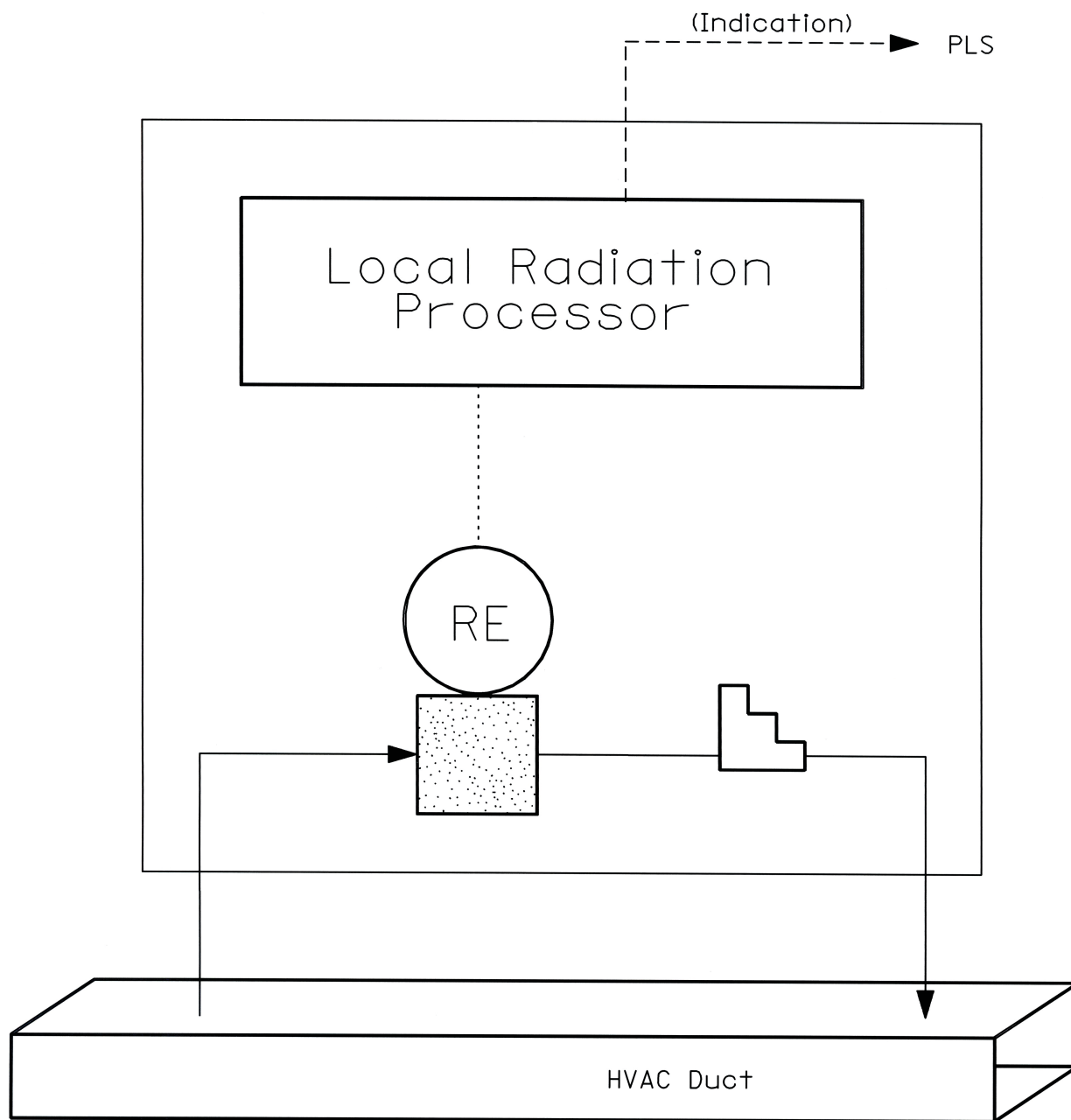
Figure 11.5-9 HVAC Duct Particulate Radiation Monitor
