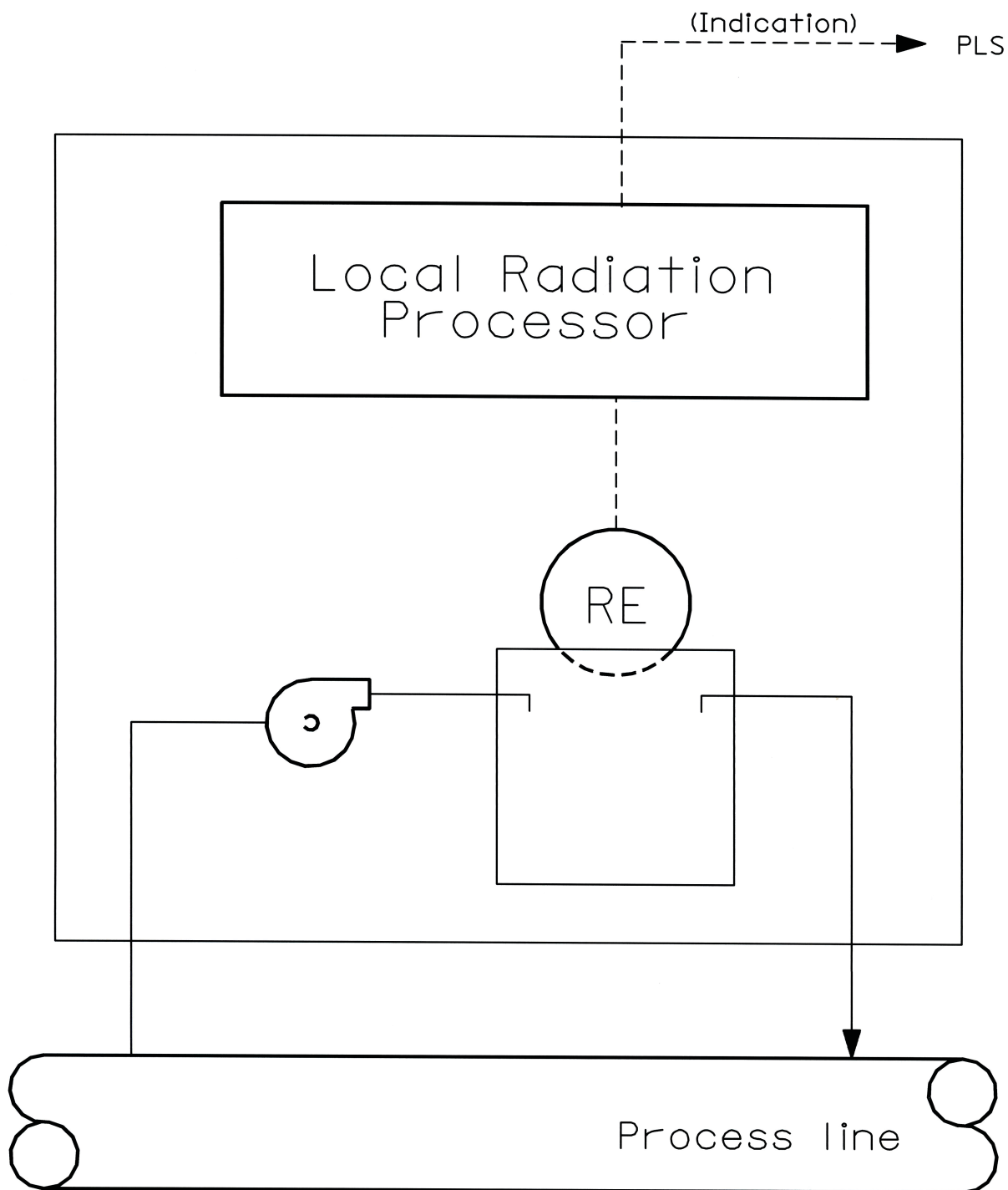
Figure 11.5-7 Liquid Offline Radiation Monitor
