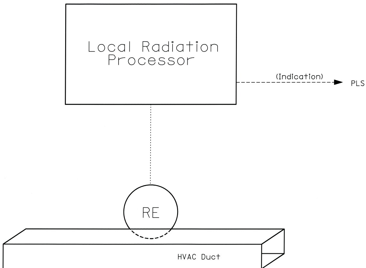
Figure 11.5-5 In-Line HVAC Duct Radiation Monitor
