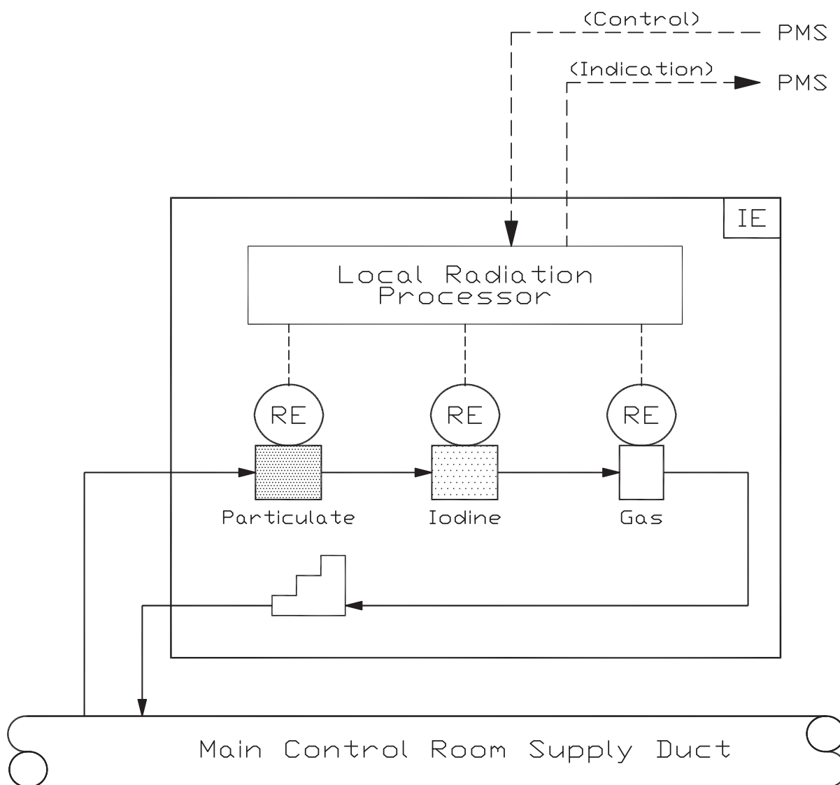
Figure 11.5-6 Safety-Related Main Control Room Supply Duct Radiation Monitor
