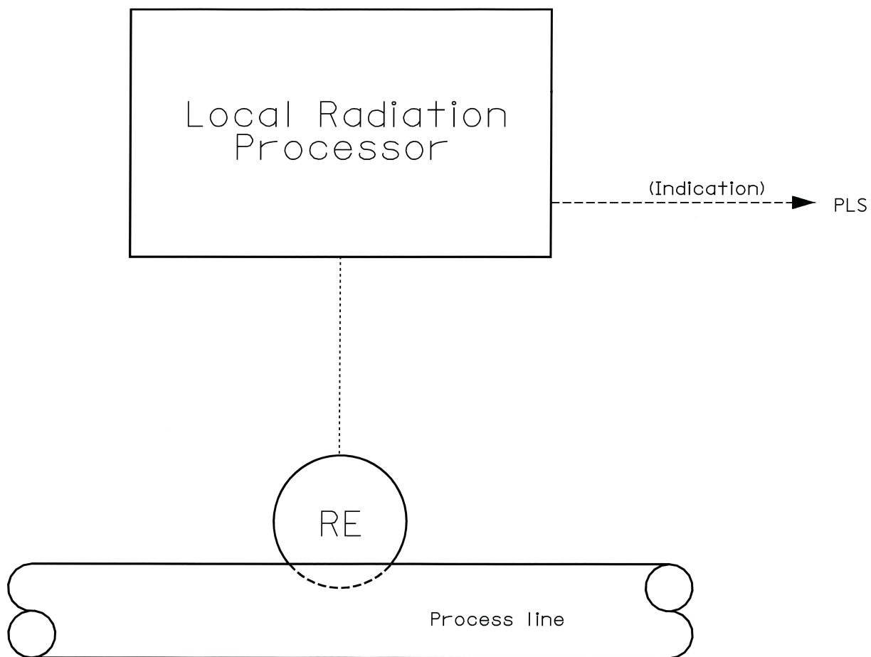
Figure 11.5-1 Process In-Line Radiation Monitor
