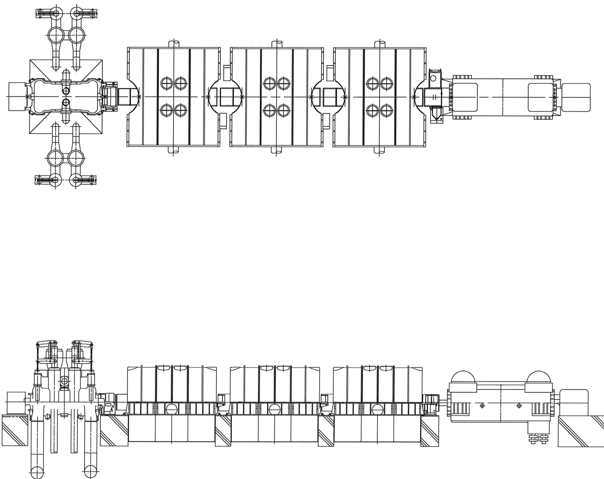
Figure 10.2-1 (Sheet 1 of 2) Turbine Generator Outline Drawing
