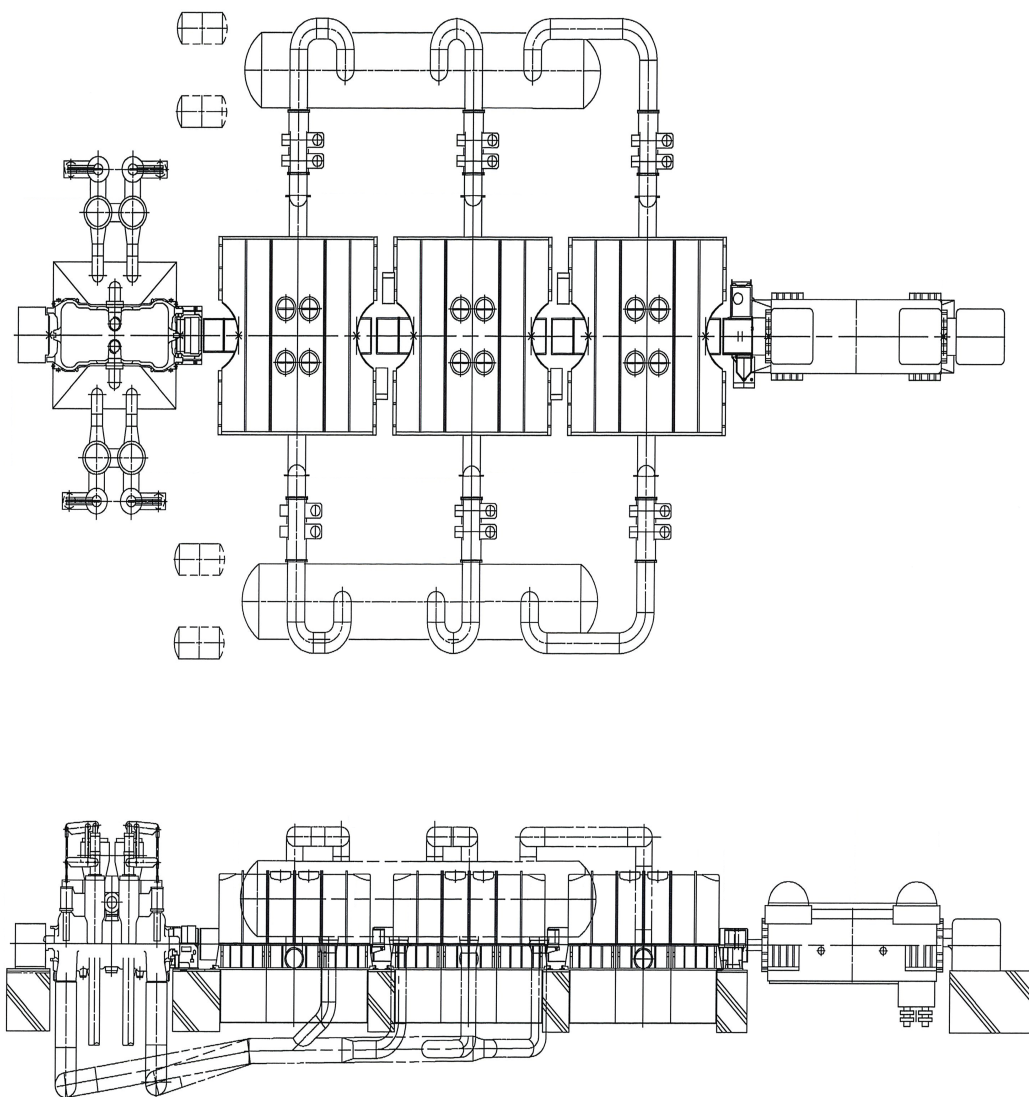
Figure 10.2-1 (Sheet 2 of 2) Turbine Generator Outline Drawing
