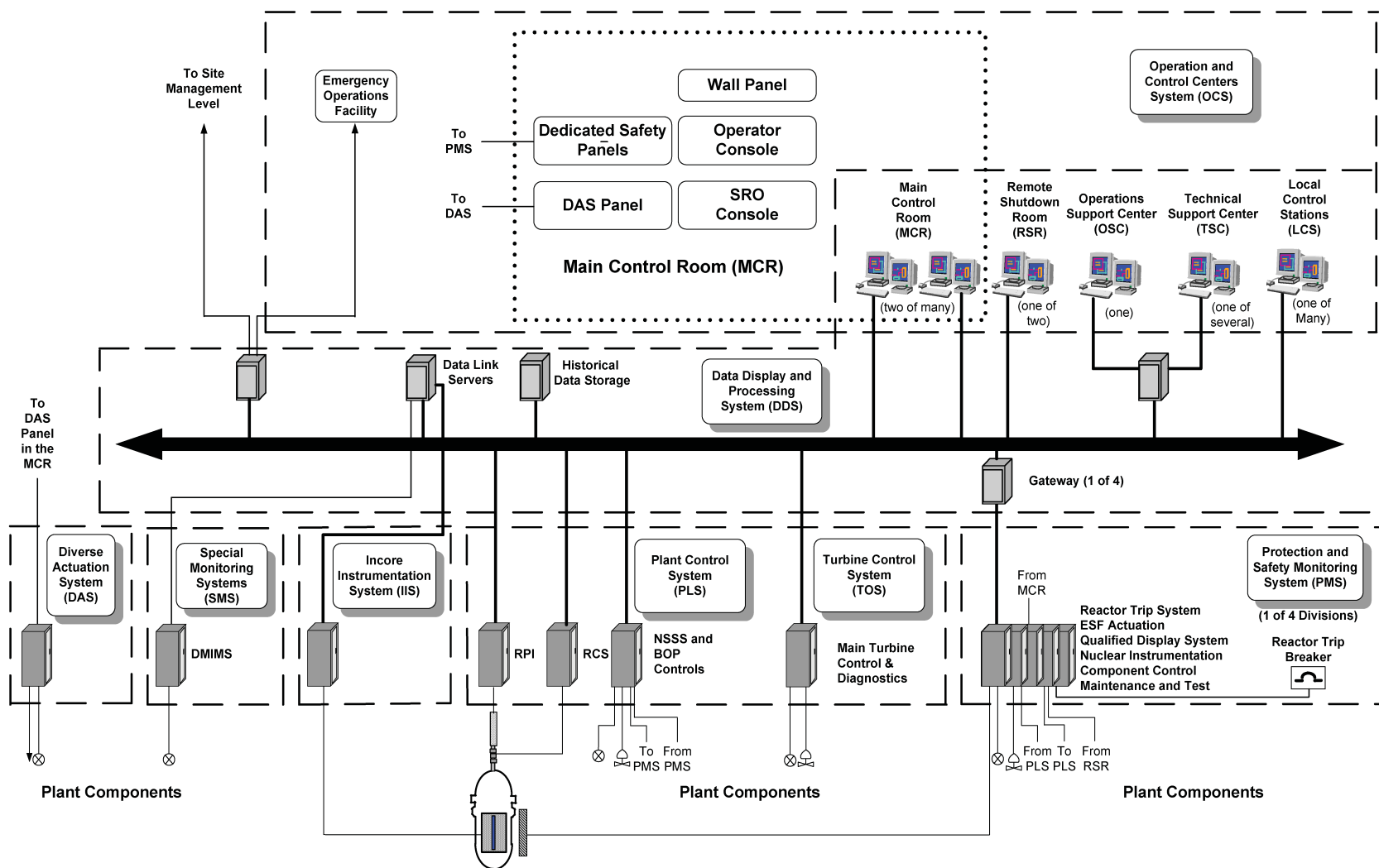
Figure 7.1-1 Instrumentation and Control Architecture
