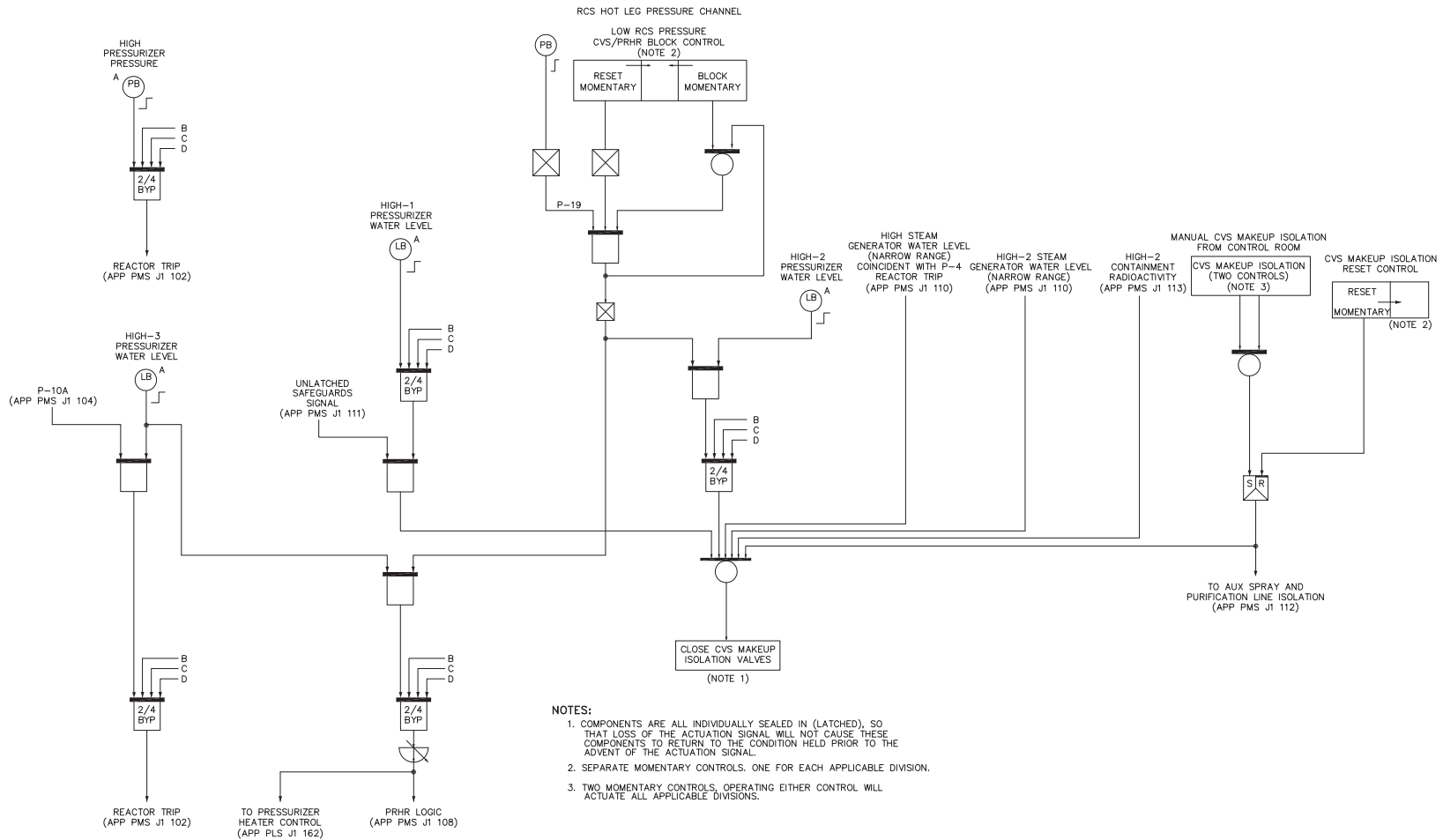
Figure 7.2-1 (Sheet 6 of 21) Functional Diagram Primary Overpressure & Loss of Heat Sink Protection
