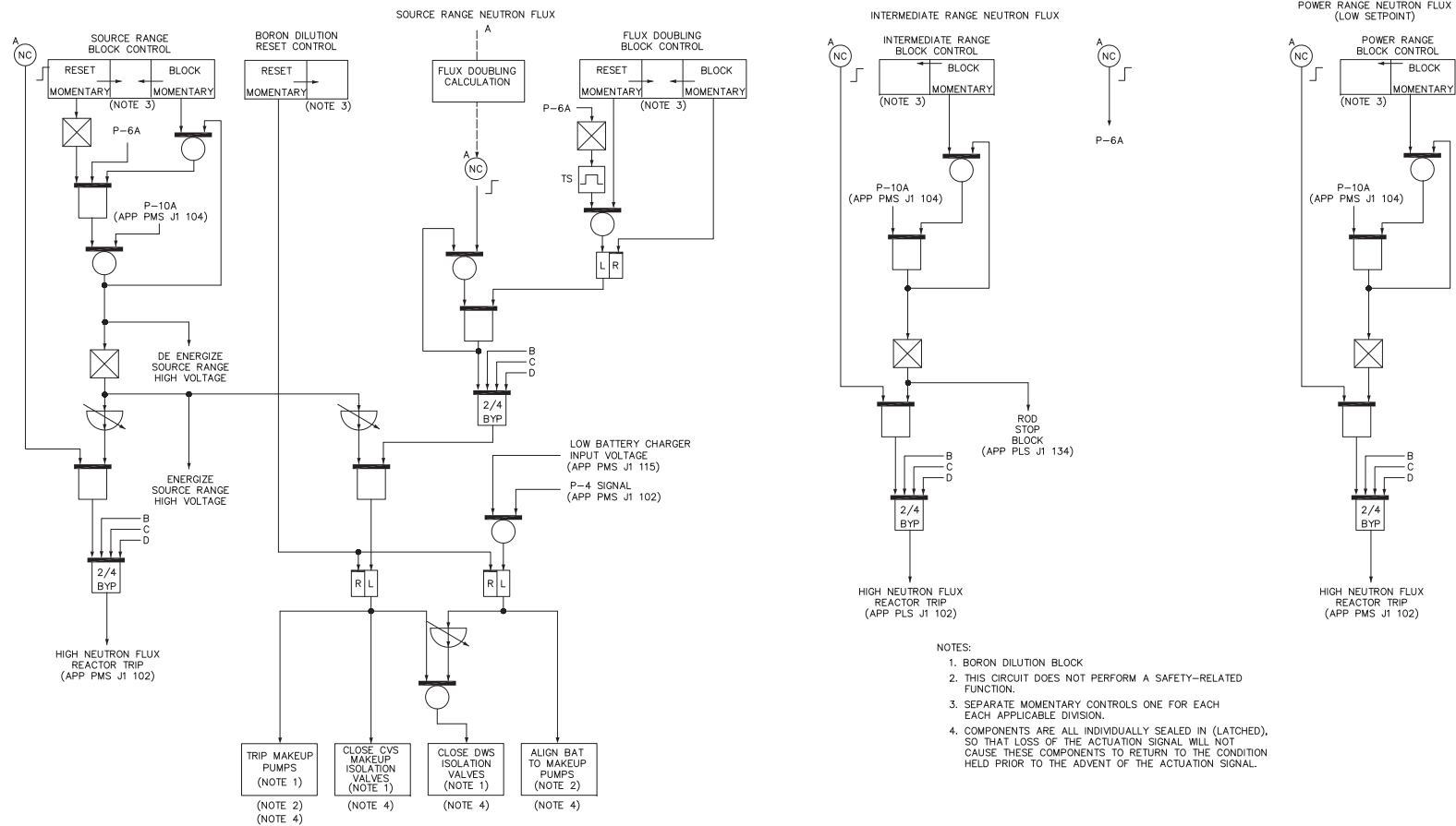
Figure 7.2-1 (Sheet 3 of 21) Functional Diagram Nuclear Startup Protection
