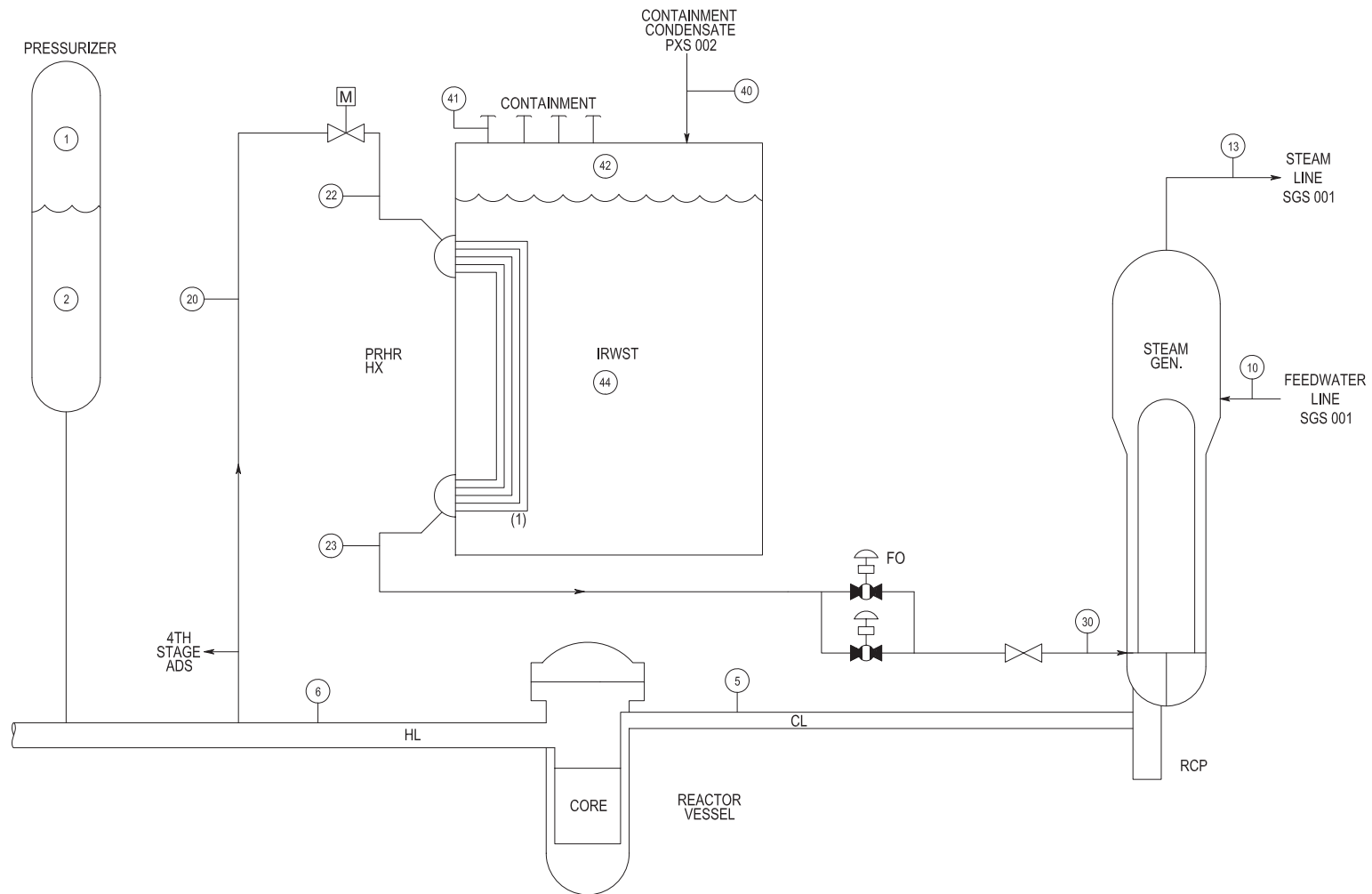
Inside Reactor Containment Figure 6.3-3 Passive Decay Heat Removal (REF) RCS & PXS
