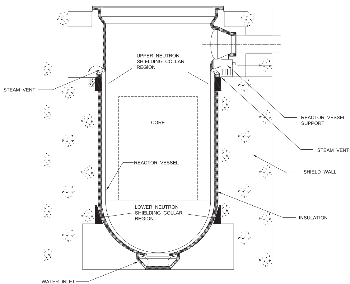
Figure 5.3-7 Schematic of Reactor Vessel Insulation
