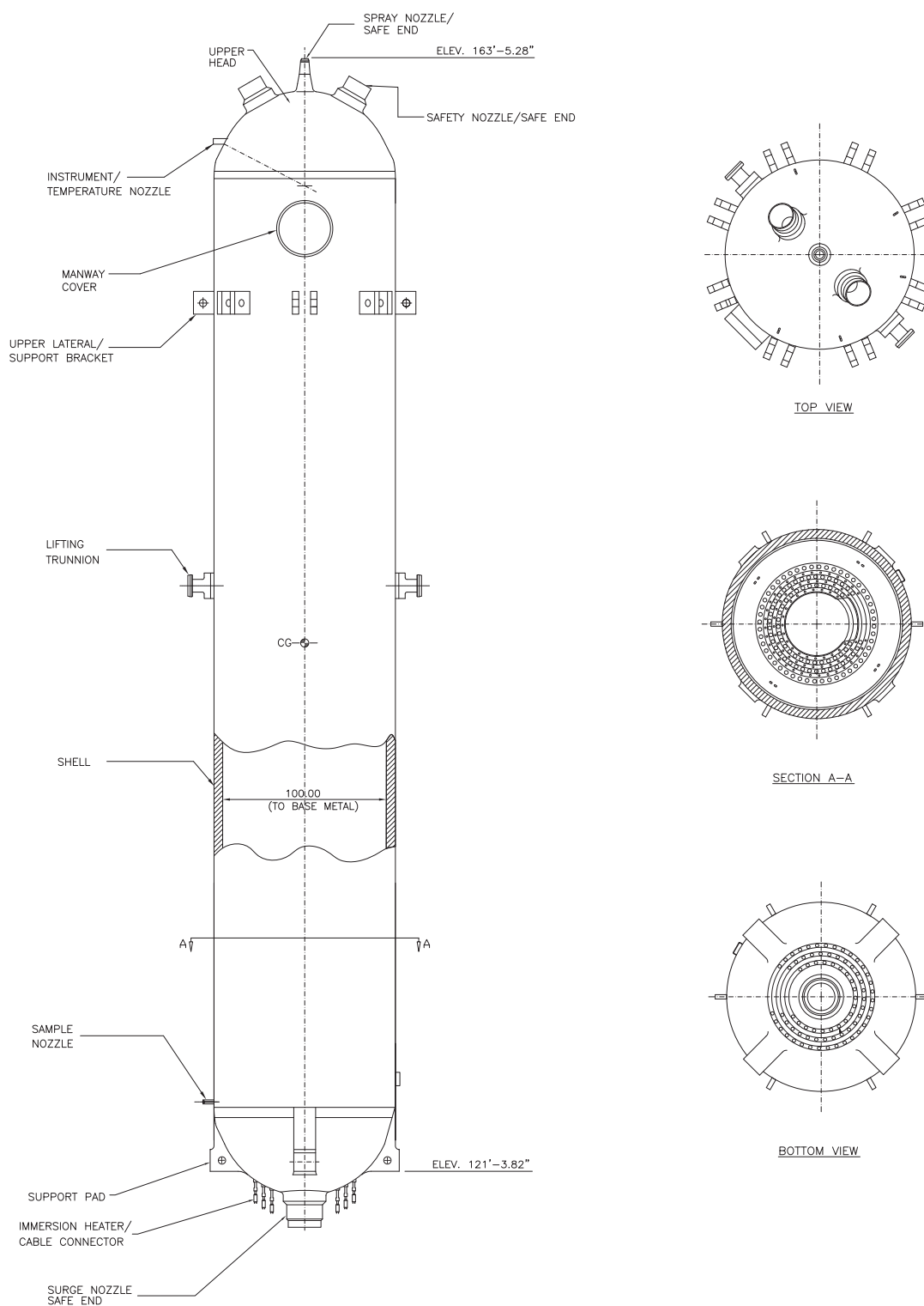
Figure 5.4-5 Pressurizer
