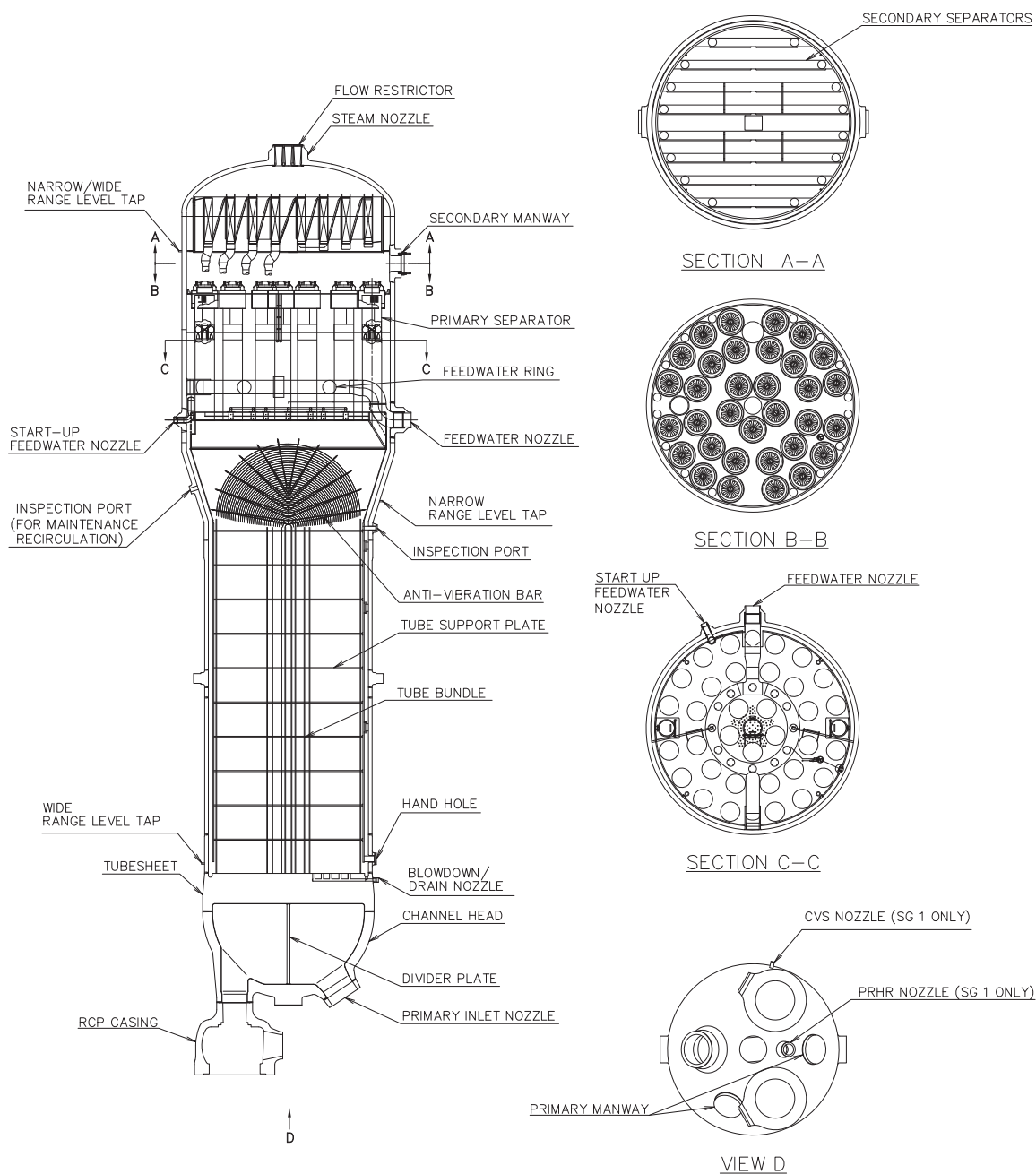
Figure 5.4-2 Steam Generator
