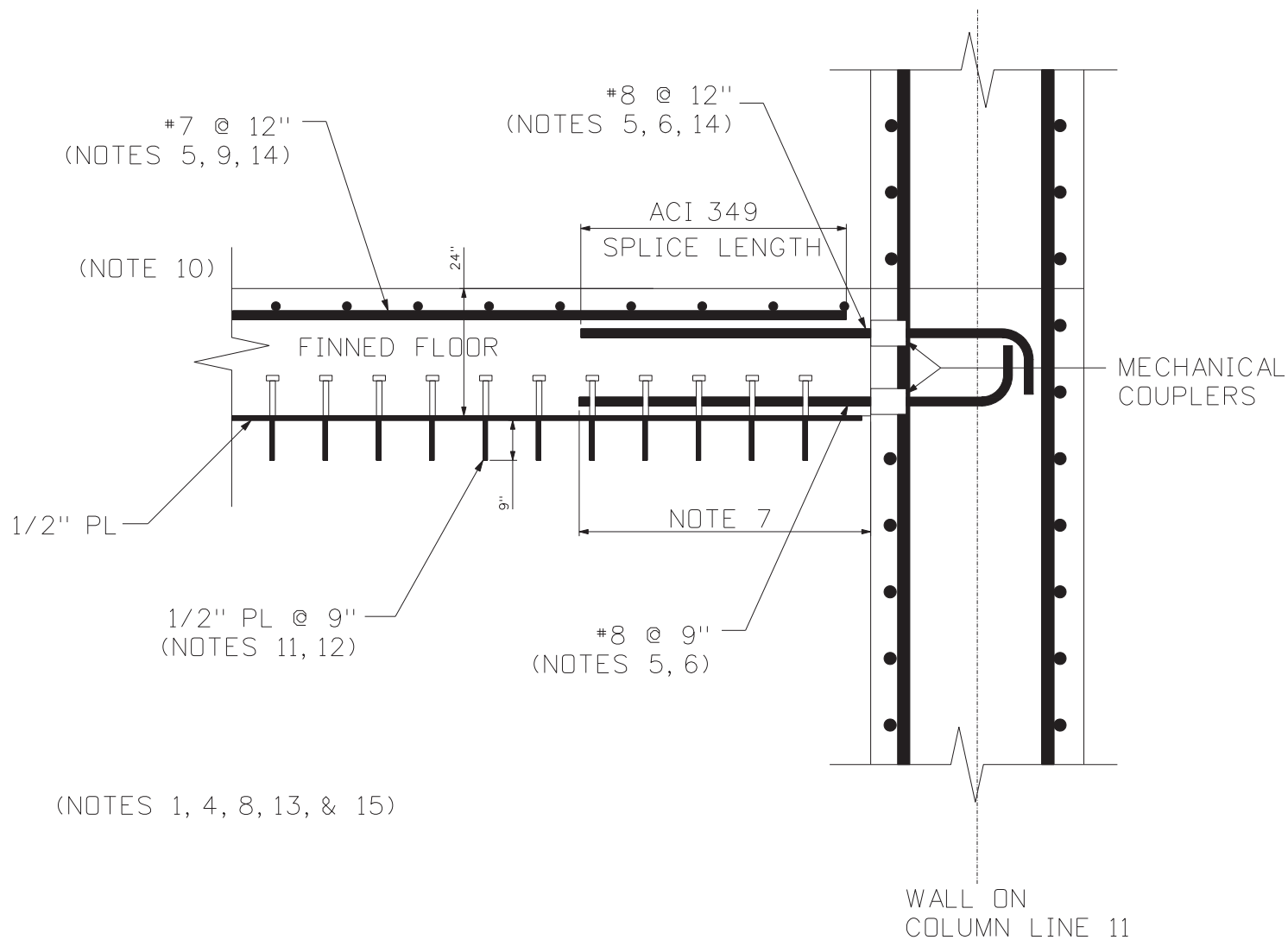
Figure 3H.5-9 (Sheet 2 of 3) [Auxiliary Building Finned Floor]*
