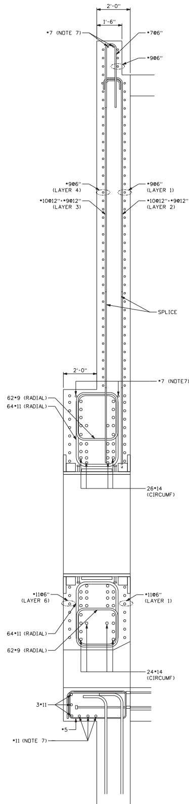
Figure 3H.5-5 (Sheet 3 of 3) [Wall 11 at Main Steamline Anchor Section A-A]*
