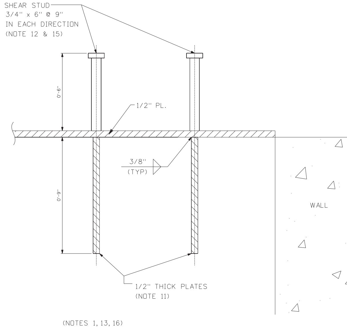
Figure 3H.5-9 (Sheet 3 of 3) [Auxiliary Building Finned Floor]*
