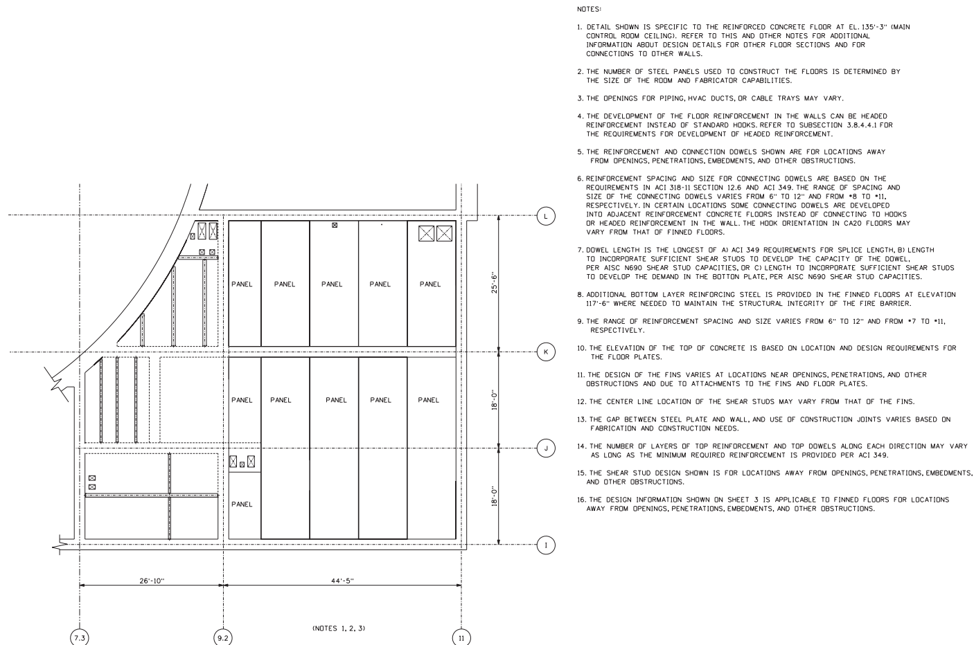
Figure 3H.5-9 (Sheet 1 of 3) [Auxiliary Building Finned Floor]*
