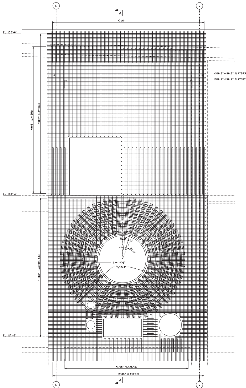
Figure 3H.5-5 (Sheet 1 of 3) [Concrete Reinforcement in Wall 11]*
