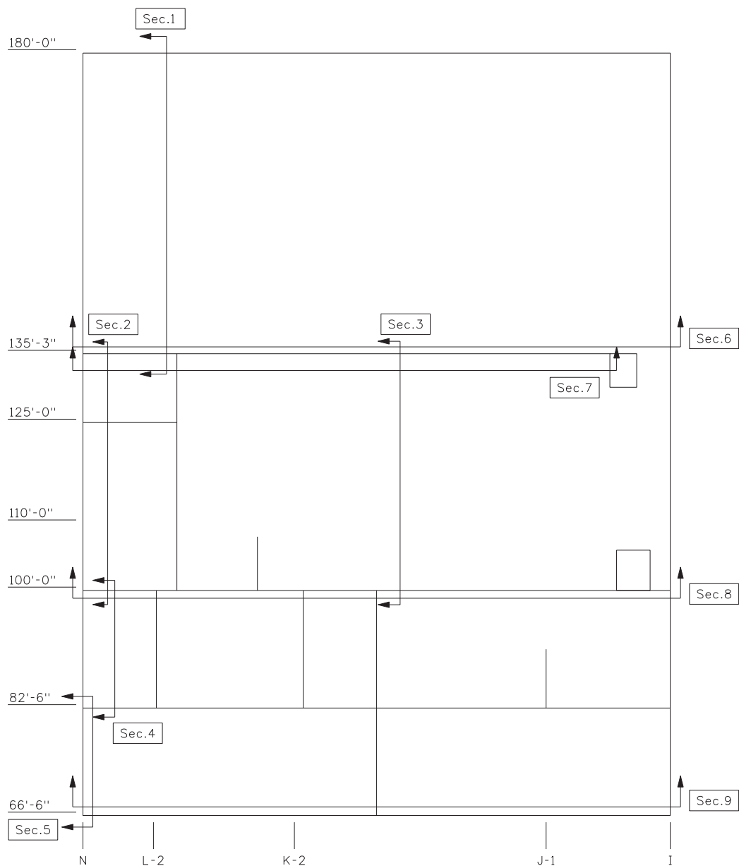
Figure 3H.5-2 (Sheet 1 of 3) [Wall on Column Line 1]*
