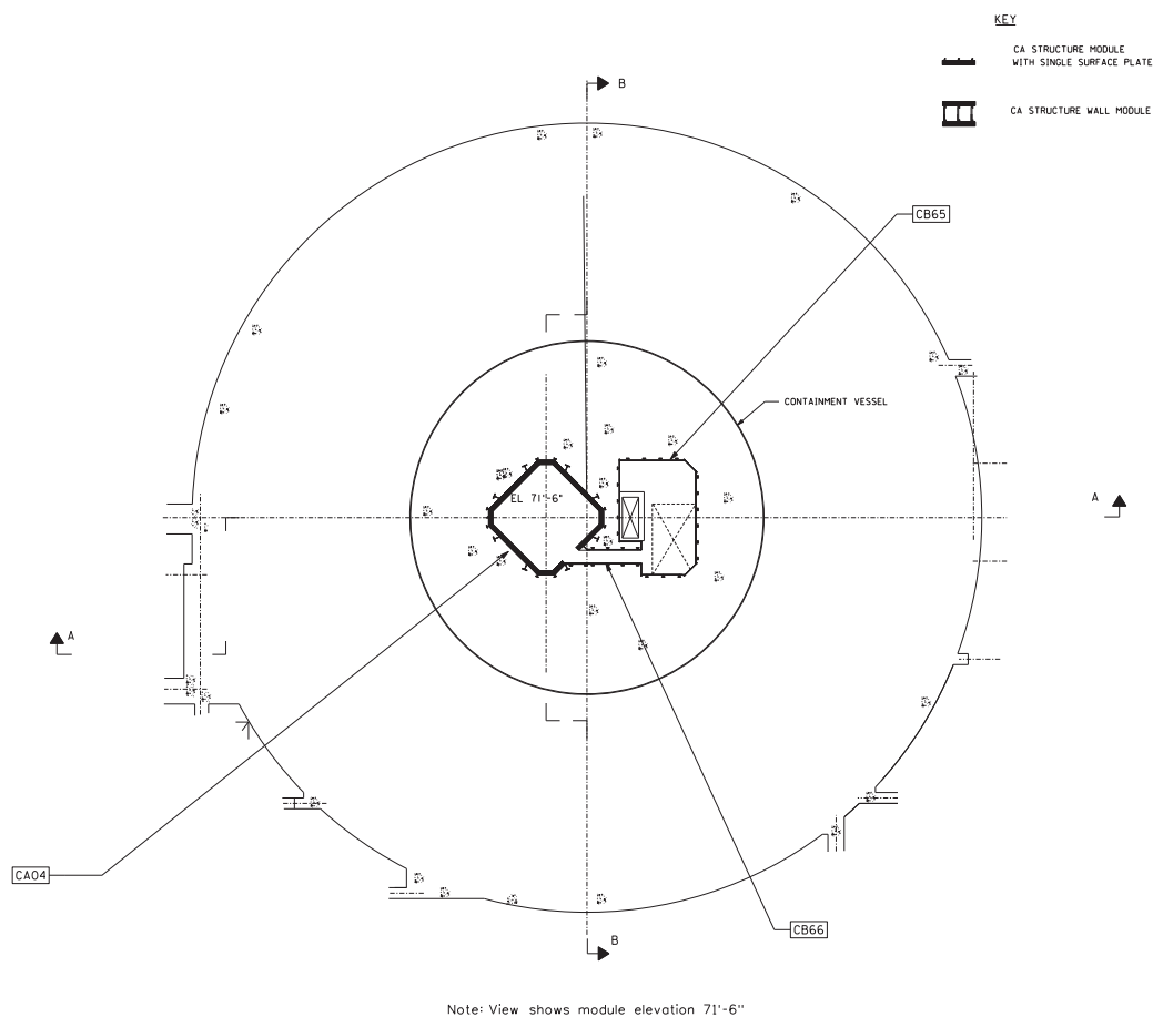
Figure 3.8.3-1 (Sheet 1 of 7) [Structural Modules in Containment Internal Structures]*
