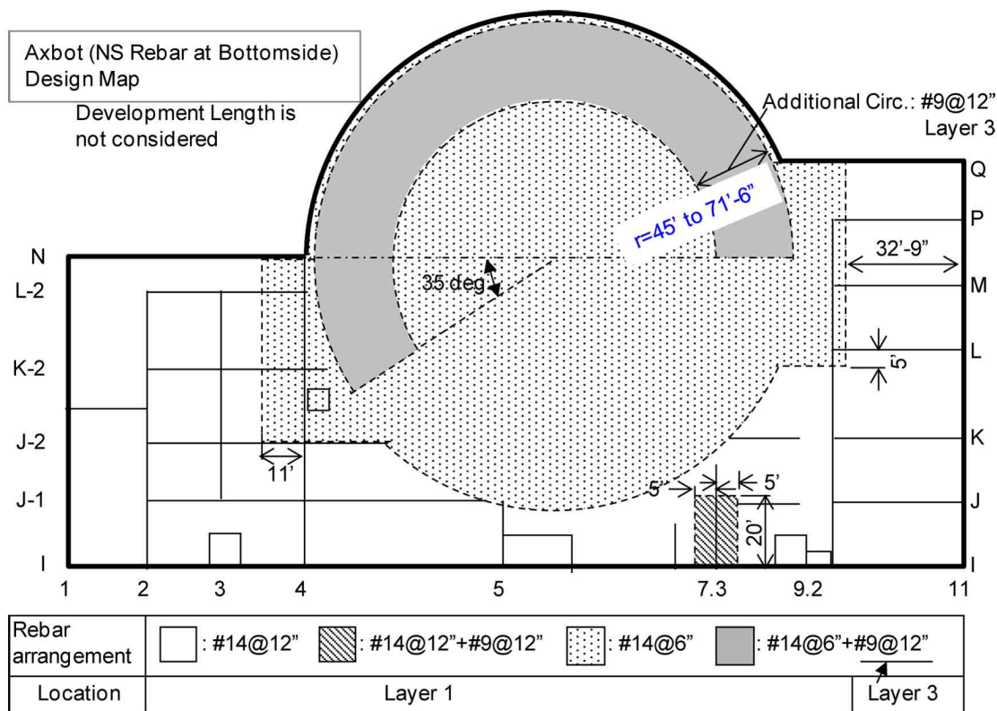
Figure 3.8.5-3 (Sheet 5 of 7) Longitudinal Reinforcement, Bottom Side of DISH and 6' Basemat (NS)
