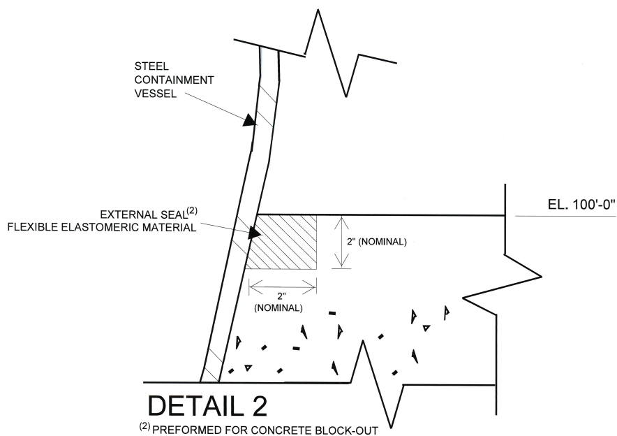
Figure 3.8.2-8 (Sheet 2 of 2) Seal Sections and Details
