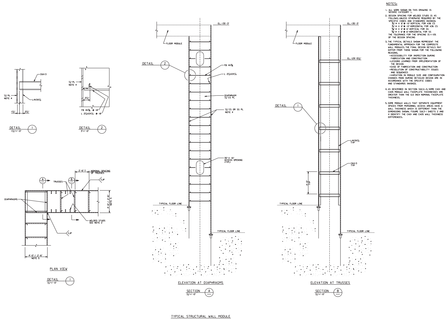
Figure 3.8.3-8 (Sheet 1 of 3) [Structural Modules – Typical Design Details]*
