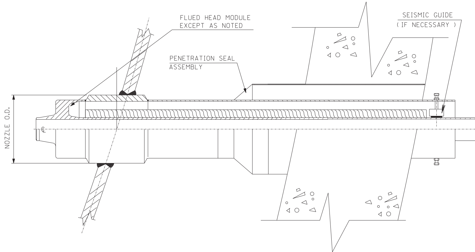
Figure 3.8.2-4 (Sheet 2 of 7) Containment Penetrations Startup Feedwater
