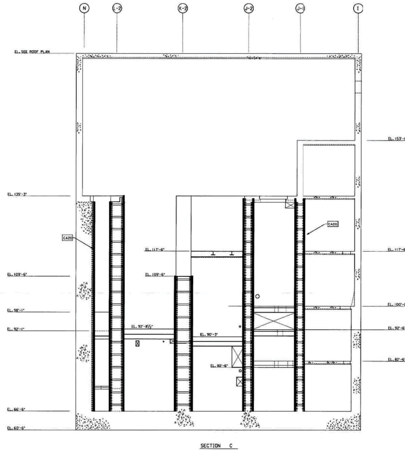
Figure 3.8.4-4 (Sheet 5 of 5) [Structural Modules in Auxiliary Building]*
