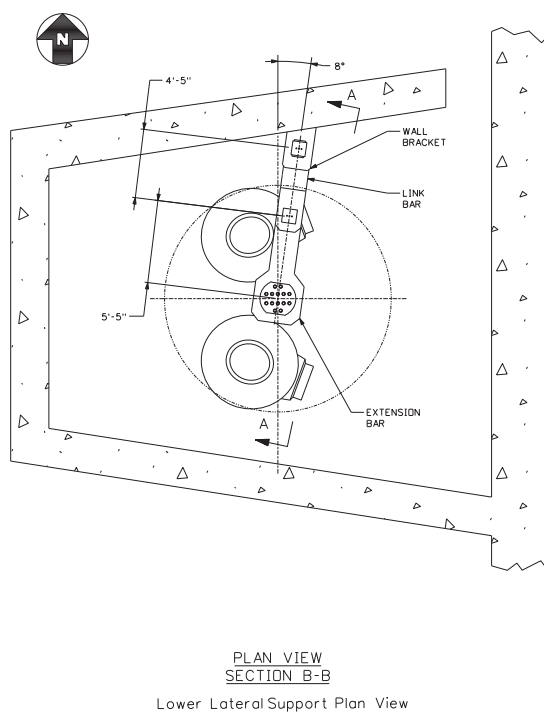
Figure 3.8.3-5 (Sheet 3 of 5) Steam Generator Supports
