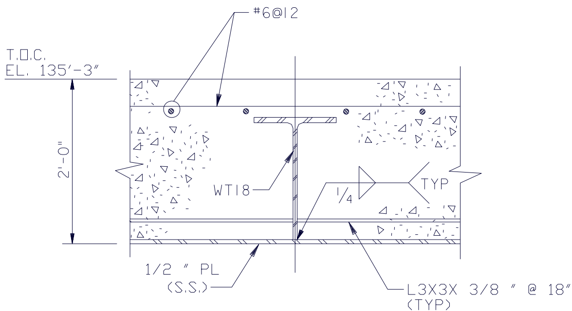
Figure 3.8.3-3 Structural Floor Module
