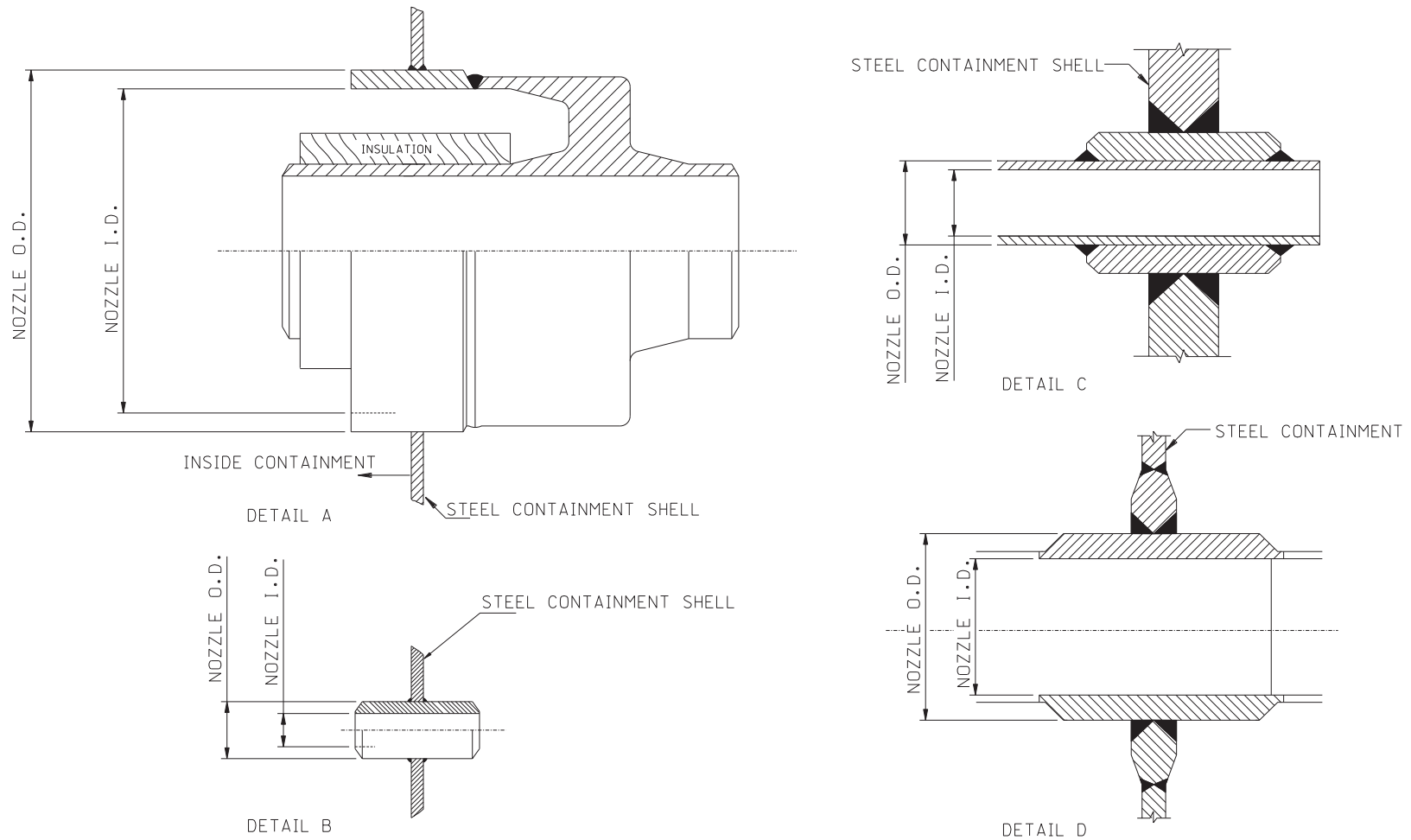
Figure 3.8.2-4 (Sheet 4 of 7) Containment Penetrations
