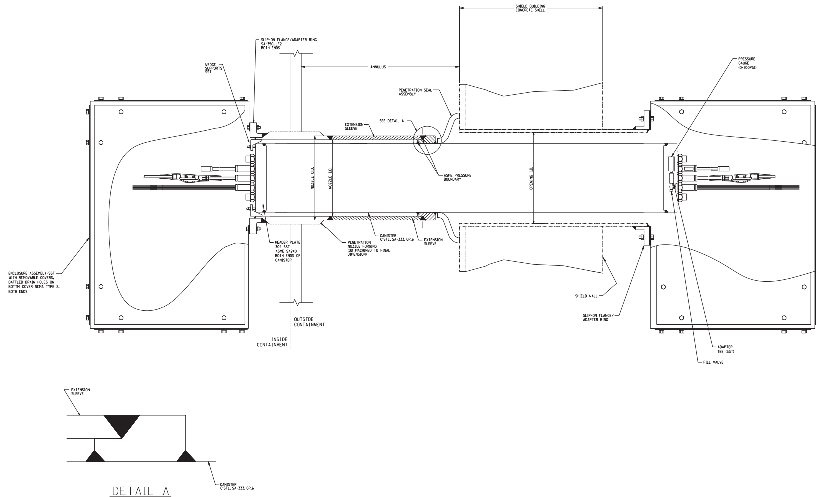
Figure 3.8.2-4 (Sheet 6 of 7) Containment Penetrations Typical Electrical Penetration
