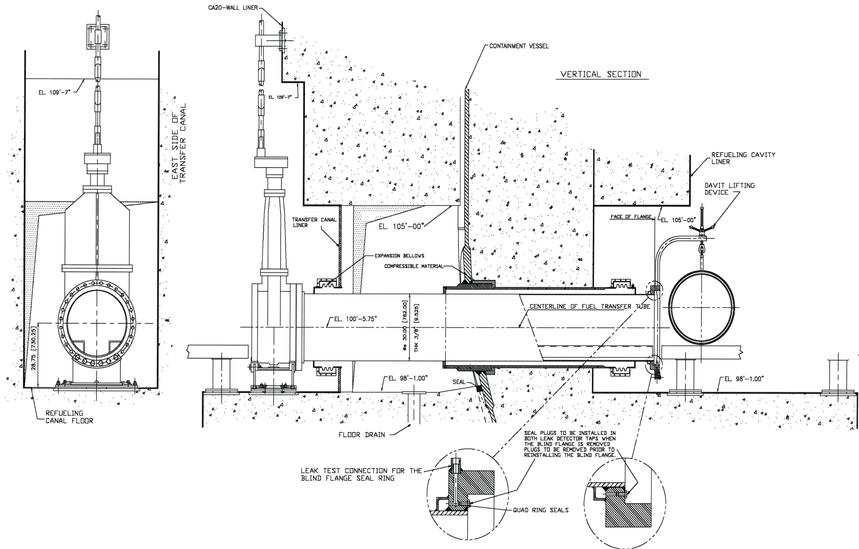
Figure 3.8.2-4 (Sheet 5 of 7) Containment Penetrations Fuel Transfer Penetration
