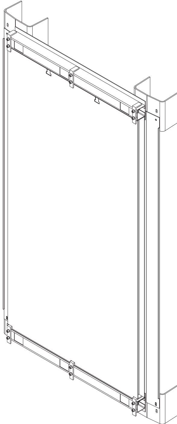
Figure 3.8.4-1 (Sheet 3 of 4) Containment Air Baffle Typical Panel on Cylinder
