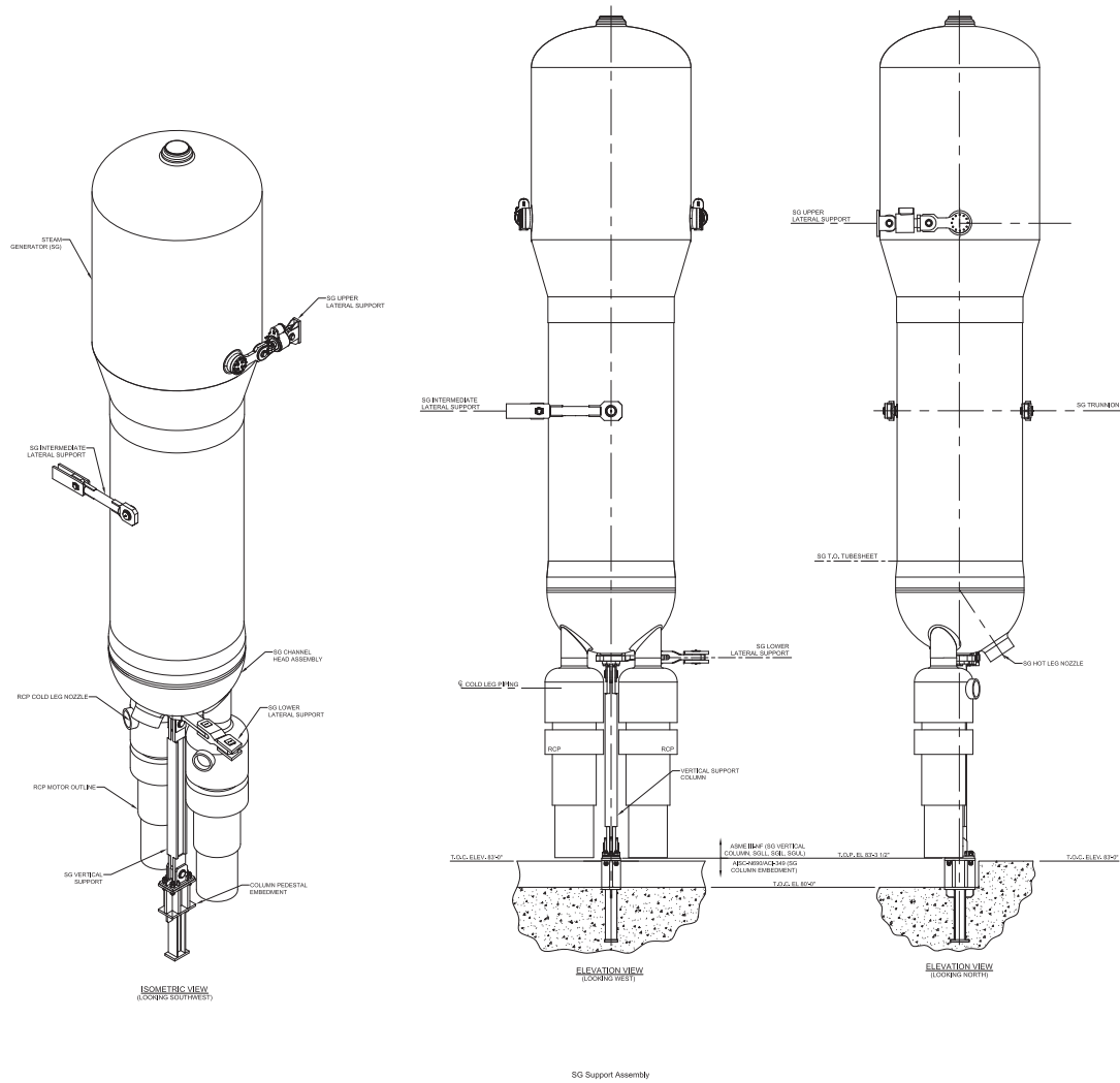
Figure 3.8.3-5 (Sheet 1 of 5) Steam Generator Supports
