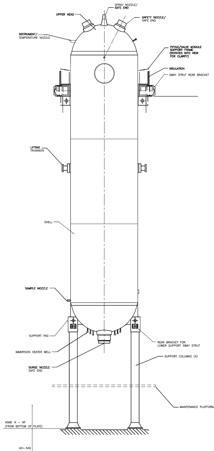
Figure 3.8.3-6 (Sheet 1 of 4) Pressurizer Support Columns
