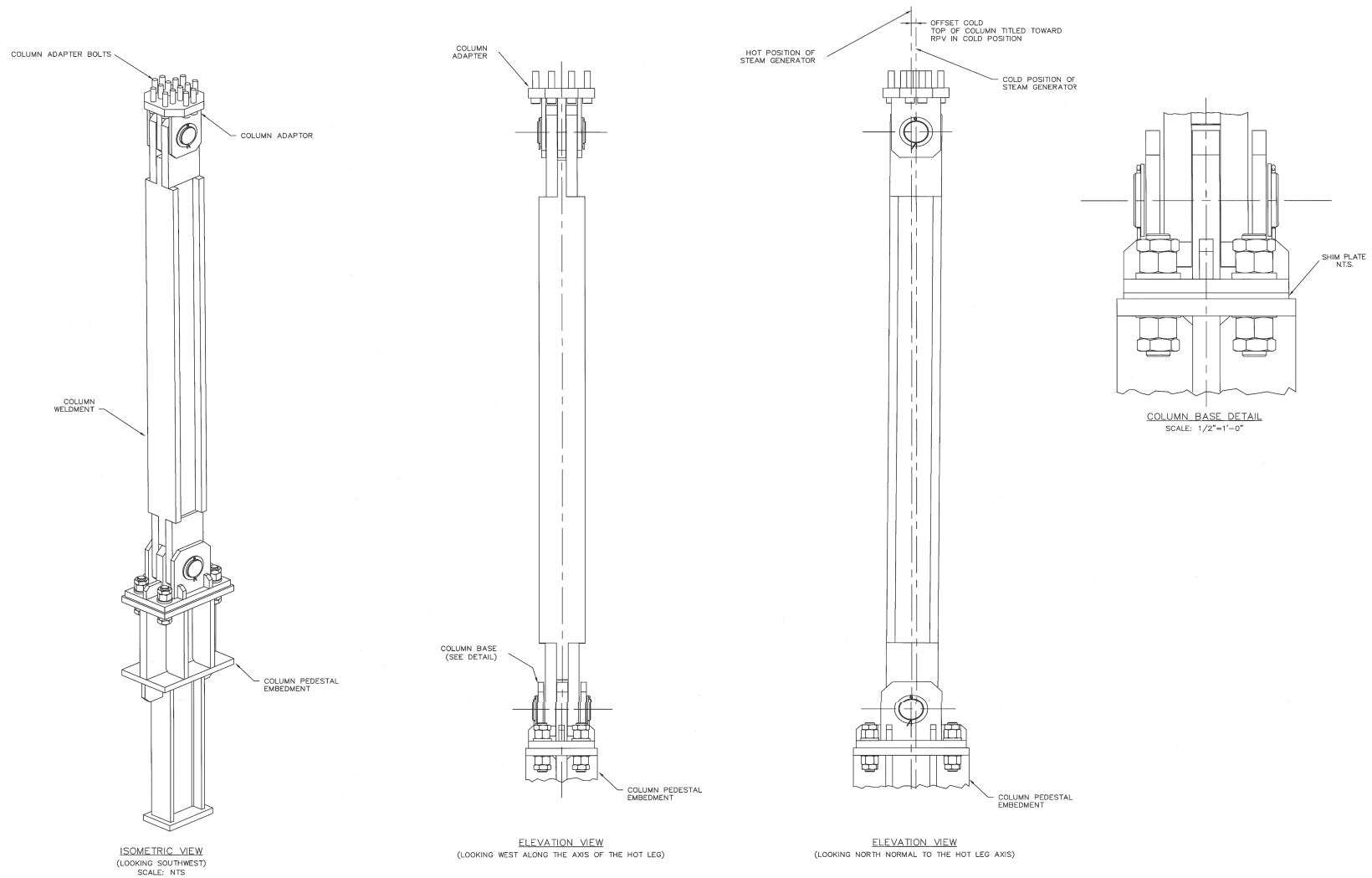
Figure 3.8.3-5 (Sheet 2 of 5) Steam Generator Supports
