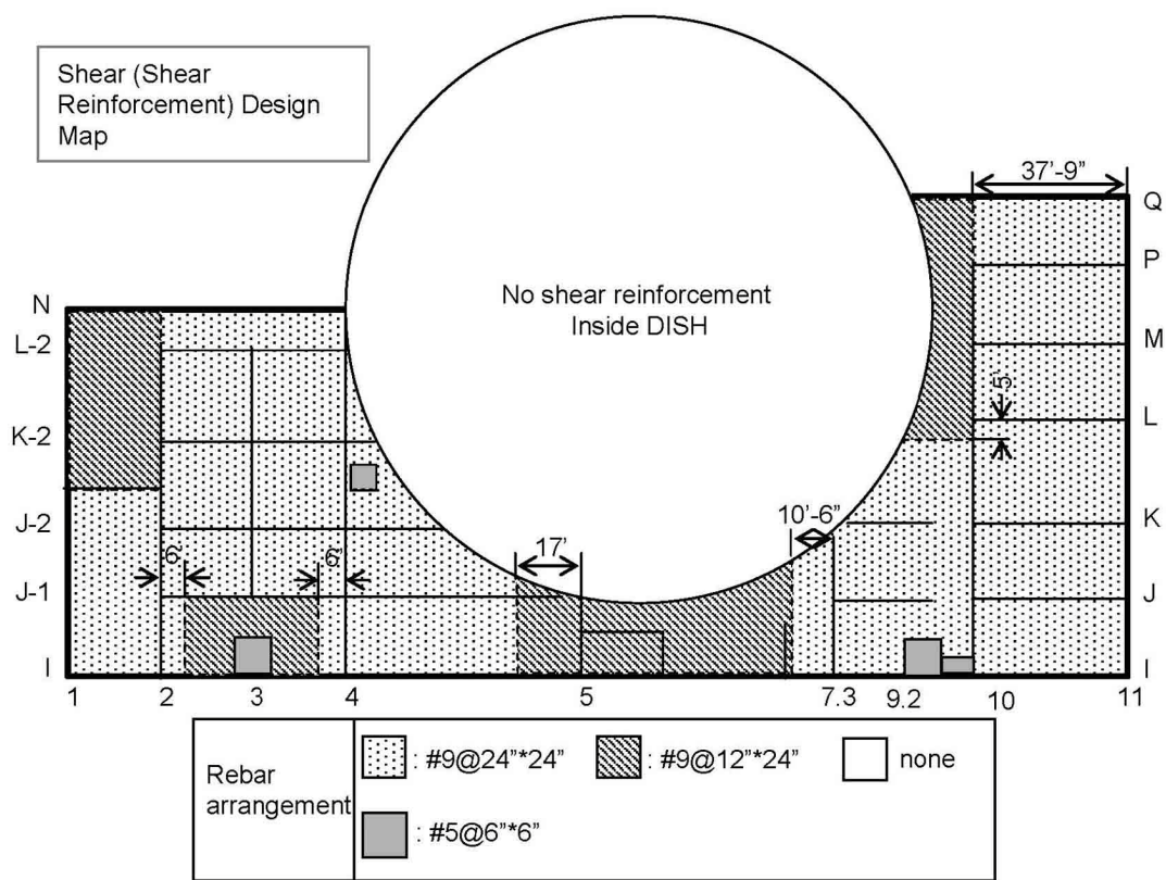
Figure 3.8.5-3 (Sheet 7 of 7) Shear Reinforcement Map
