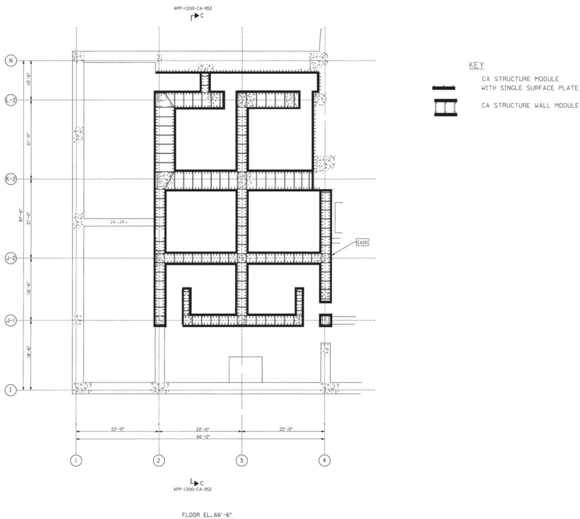
Figure 3.8.4-4 (Sheet 1 of 5) [Structural Modules in Auxiliary Building]*
