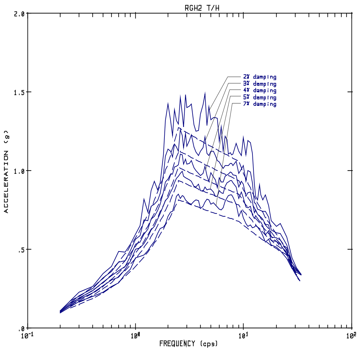
Figure 3.7.1-7 Acceleration Response Spectra of Design Horizontal Time History, "H2"
