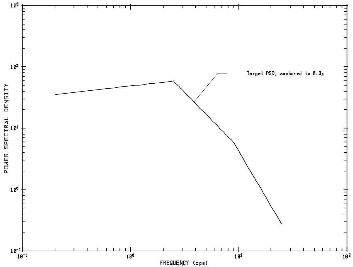
Figure 3.7.1-9 Minimum Power Spectral Density Curve (Normalized to 0.3g)
