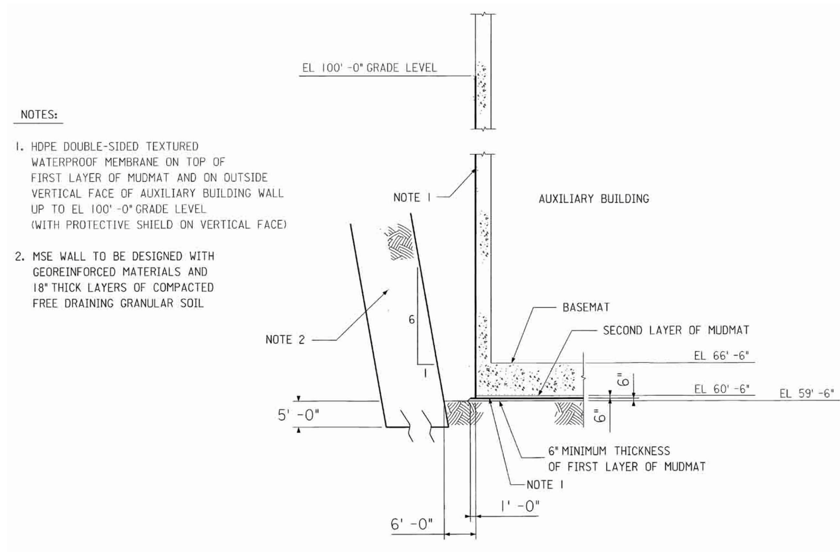
Figure 3.4-1 Typical Details of Nuclear Island Waterproofing Below Grade
