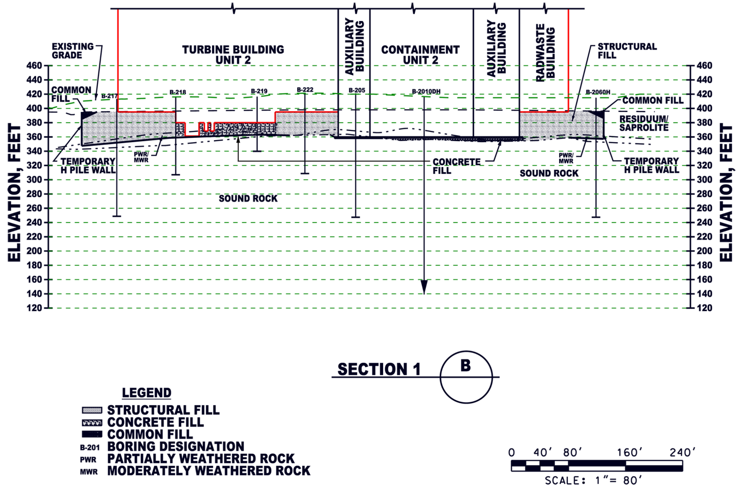
Figure 2.5.4-221 Cross-Section of Structure Foundation B-B
