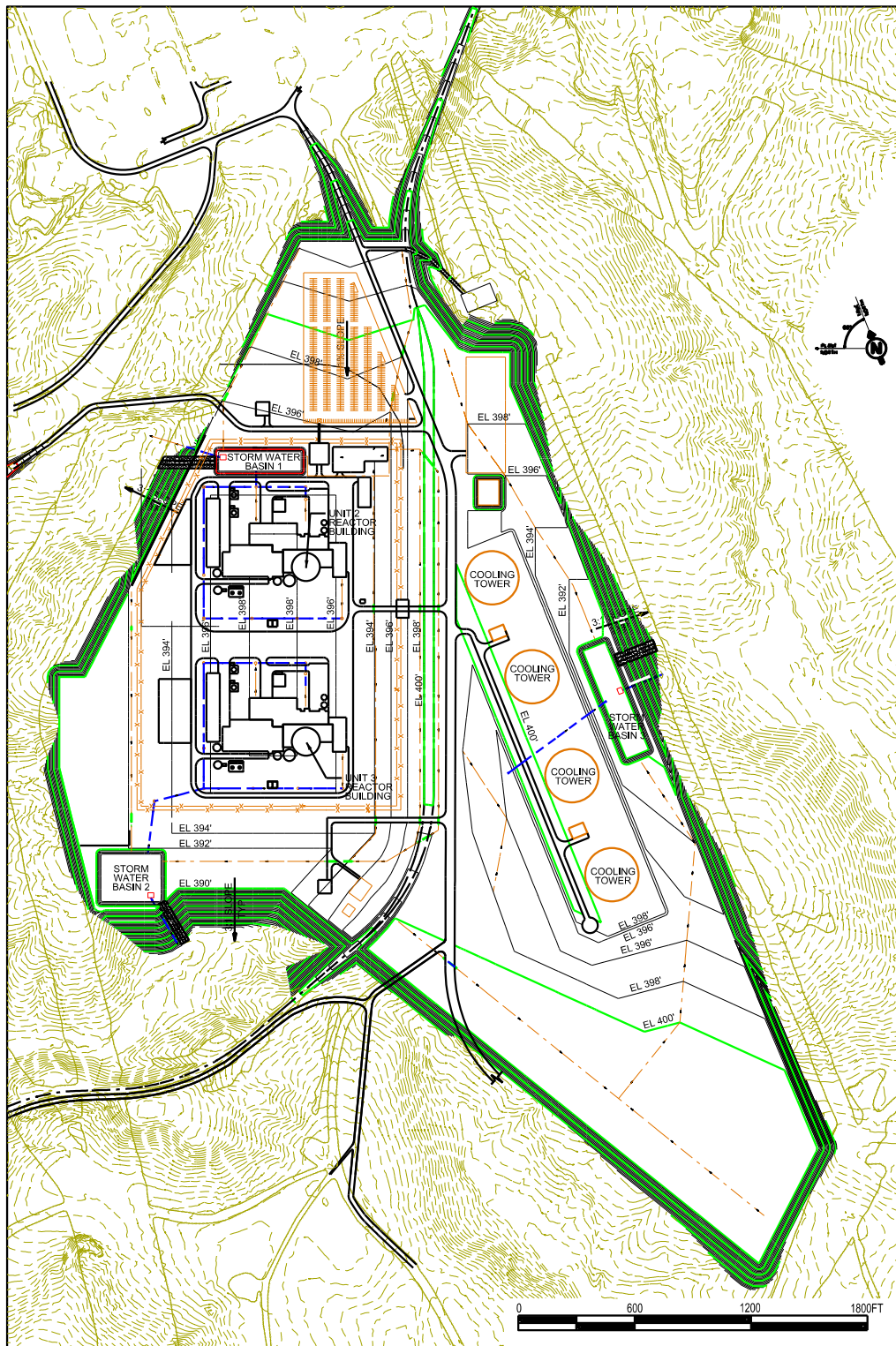
Figure 2.5.4-245 Site Grade Plan
