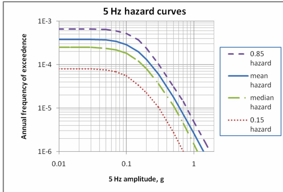
Figure 2.5.2-231 Mean and Fractile 5 Hz Seismic Hazard Curves
