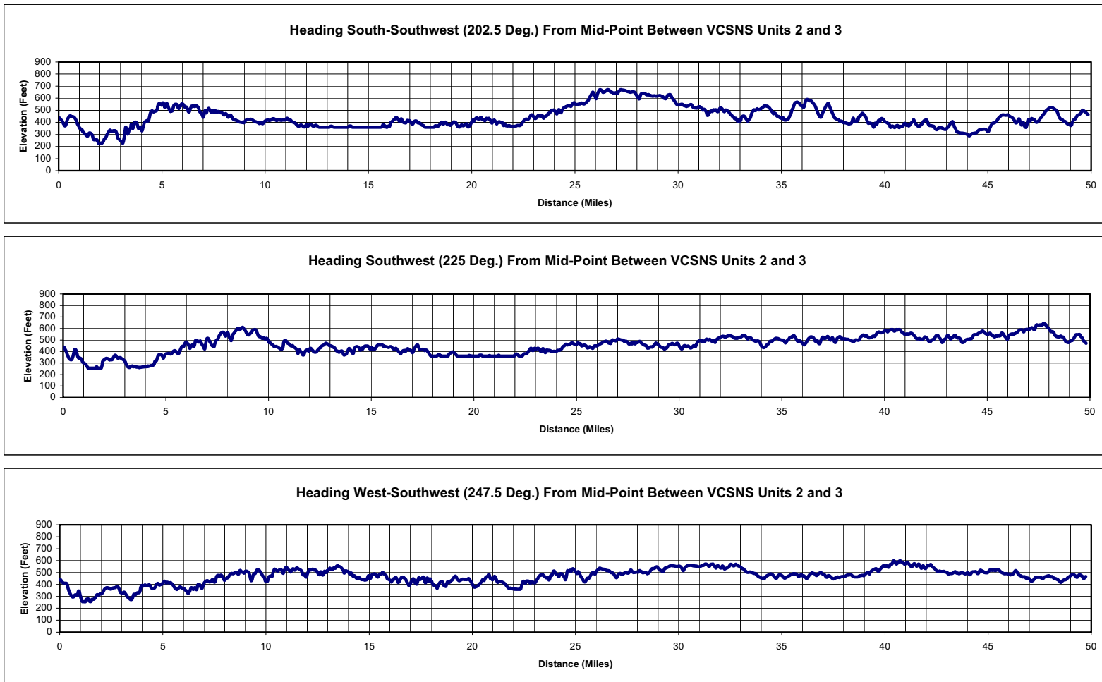
Figure 2.3-215 Terrain Elevation Profiles Within 50 Miles of the Site for Units 2 and 3 (Sheet 4 of 6)
