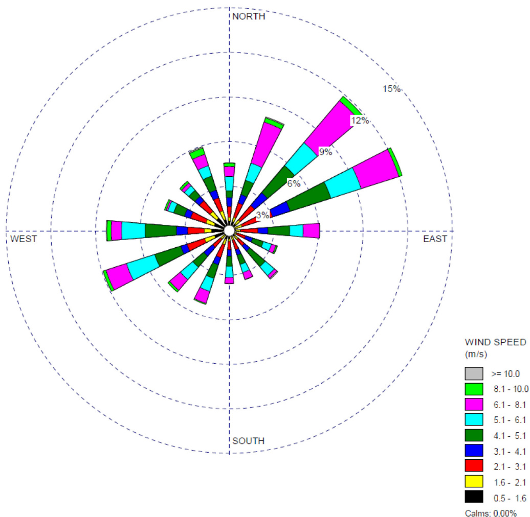
Figure 2.3-212 60-Meter Level Composite Wind Rose for the Units 2 and 3 Monitoring Program (January 1, 2007–December 31, 2008) — Autumn
