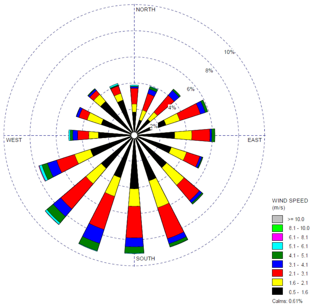
Figure 2.3-205 10-Meter Level Composite Wind Rose for the Units 2 and 3 Monitoring Program (January 1, 2007–December 31, 2008) — Summer
