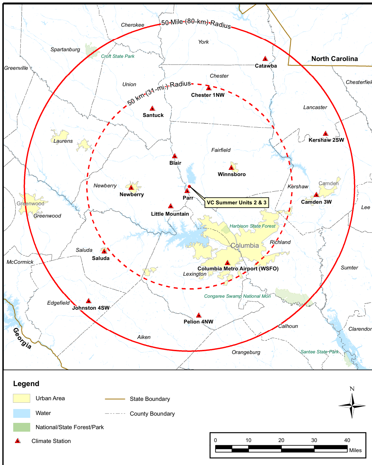
Figure 2.3-201 Climatological Observing Stations Near the VCSNS Site
