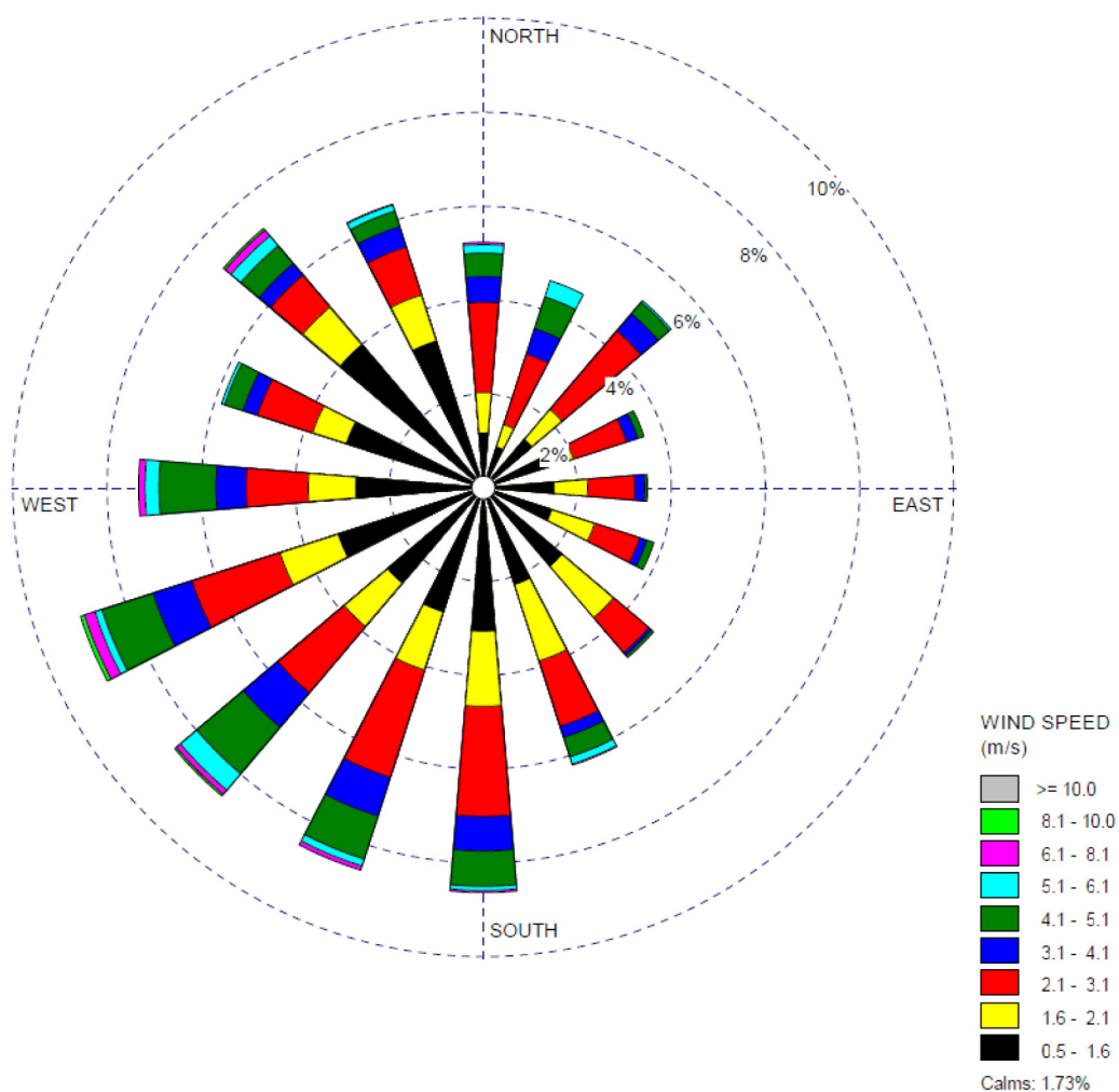
Figure 2.3-204 10-Meter Level Composite Wind Rose for the Units 2 and 3 Monitoring Program (January 1, 2007–December 31, 2008) — Spring
