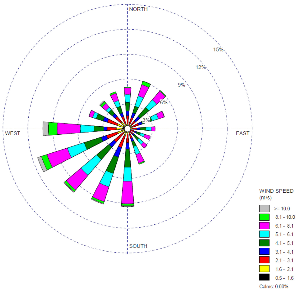
Figure 2.3-210 60-Meter Level Composite Wind Rose for the Units 2 and 3 Monitoring Program (January 1, 2007–December 31, 2008) — Spring
