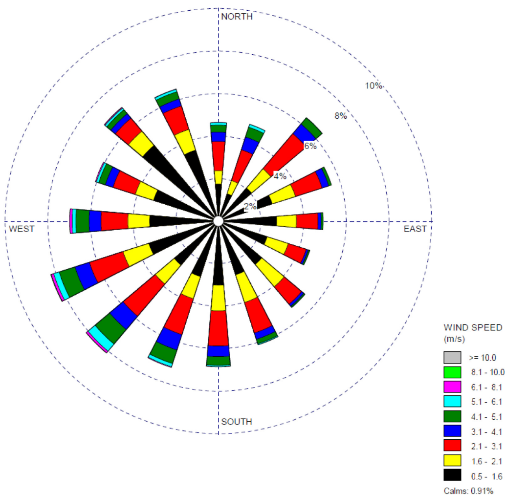
Figure 2.3-202 10-Meter Level Composite Wind Rose for the Units 2 and 3 Monitoring Program (January 1, 2007–December 31, 2008) — Annual
