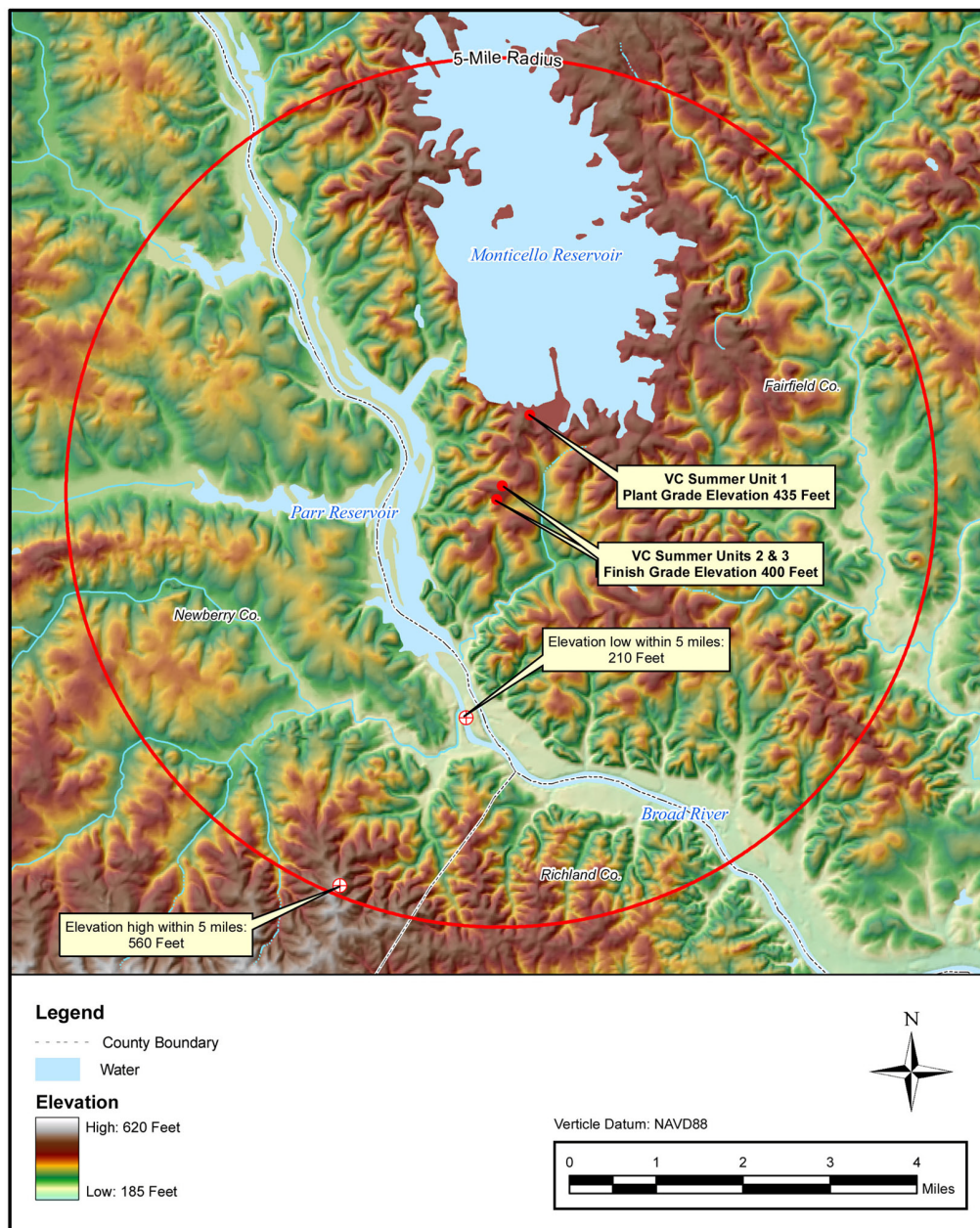
Figure 2.3-216 Site and Vicinity Map (5-Mile Radius)
