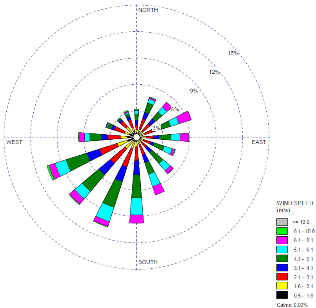
Figure 2.3-211 60-Meter Level Composite Wind Rose for the Units 2 and 3 Monitoring Program (January 1, 2007–December 31, 2008) — Summer
