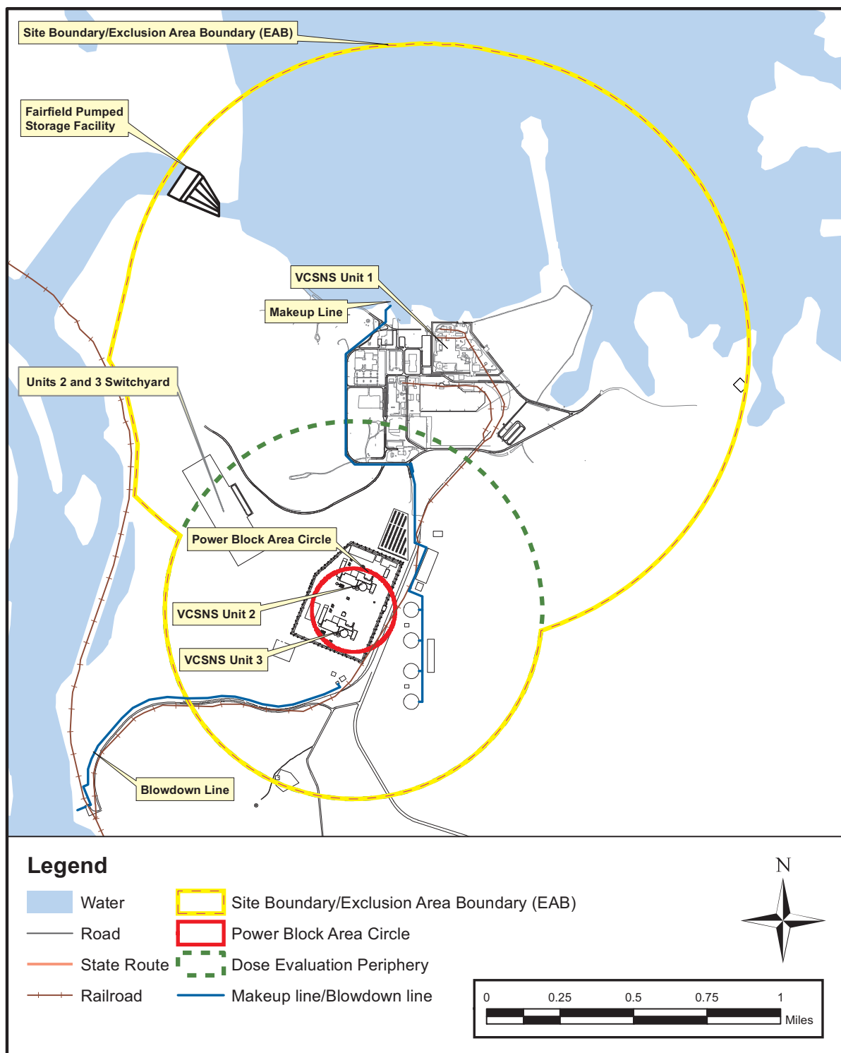
Figure 2.1-203 VCSNS Exclusion Area Boundary
