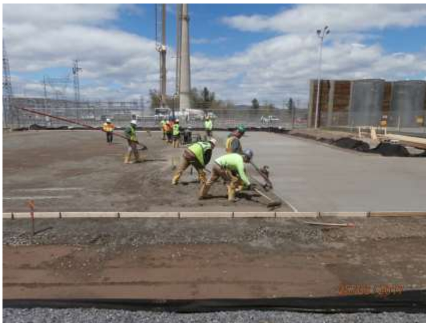
Pouring of Leveling Slab for ISFSI Pad 2
