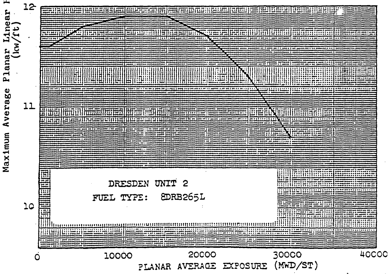
Figure 3.5.1-B Maximum Average Planar Linear Heat Generation Rate (MAPLHGR) vs. Planar Average Exposure Amendment No. 45 81C-1
