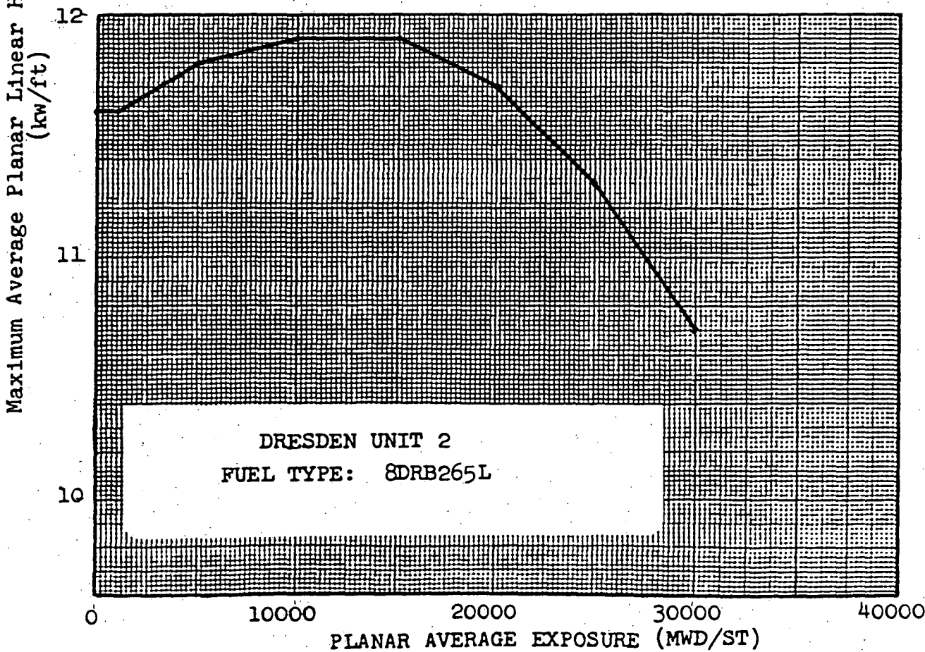
Figure 3.5.1-B Maximum Average Planar Linear Heat Generation Rate (MAPLHGR) vs. Planar Average Exposure
