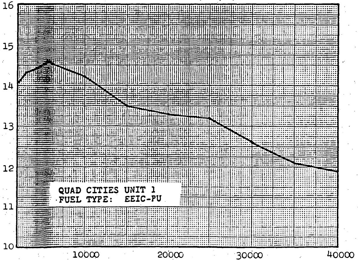
Figure 3.5-1 Maximum Average Planar Linear Heat Generation Rate (MAPLHGR) vs. Planar Average Exposure (Sheet 3 of 3)
