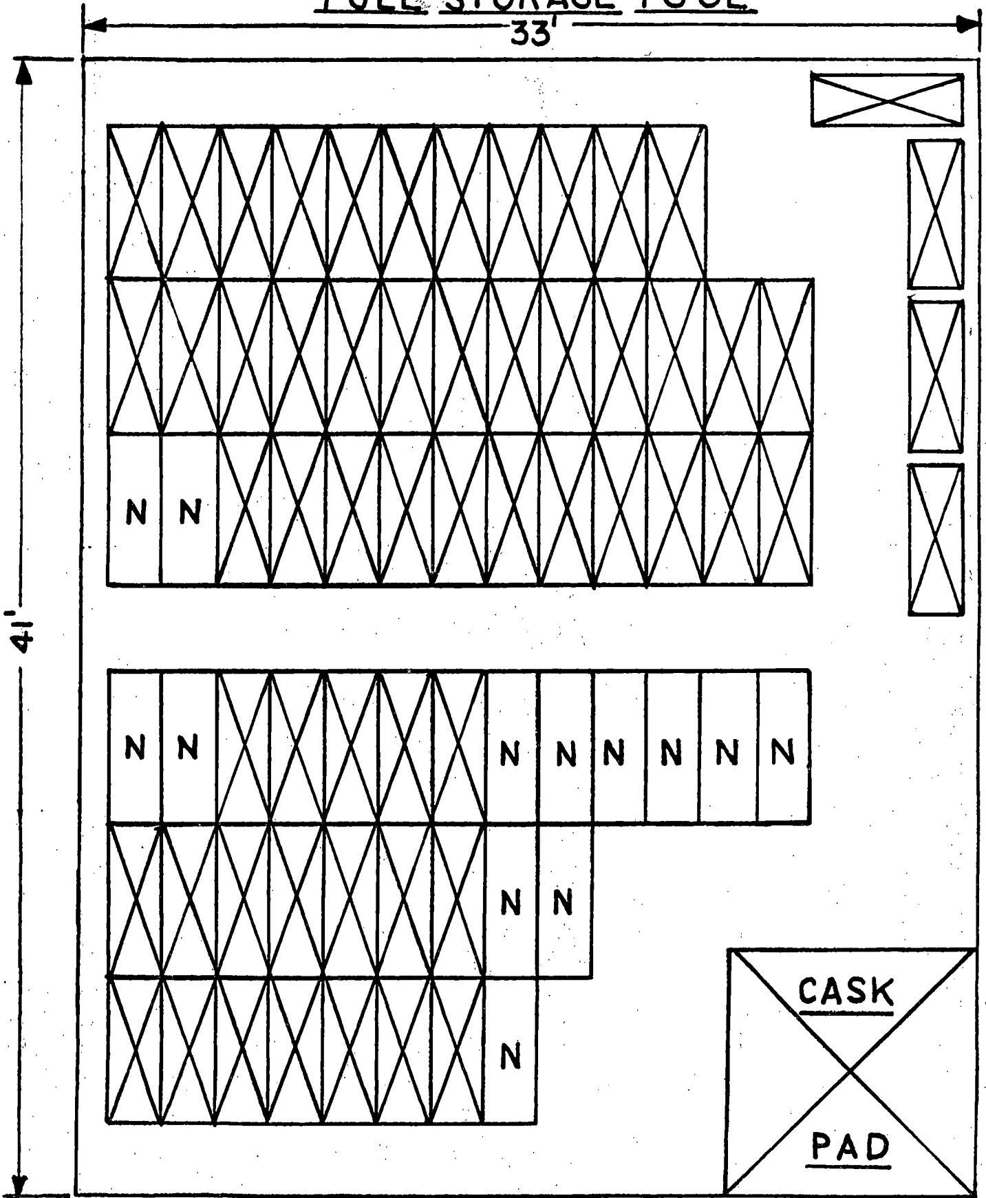
RACK ARRANGEMENT FIGURE 3-2
