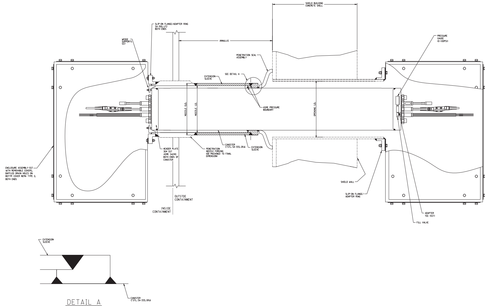
Figure 3.8.2-4 (Sheet 6 of 7) Containment Penetrations Typical Electrical Penetration
