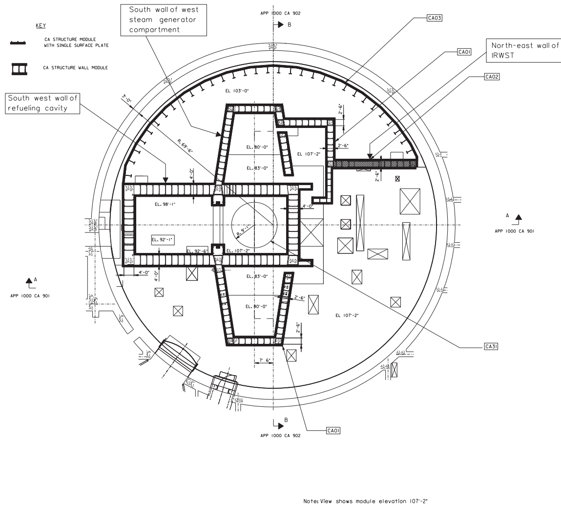
Figure 3.8.3-18 [Location of Structural Wall Modules]*
