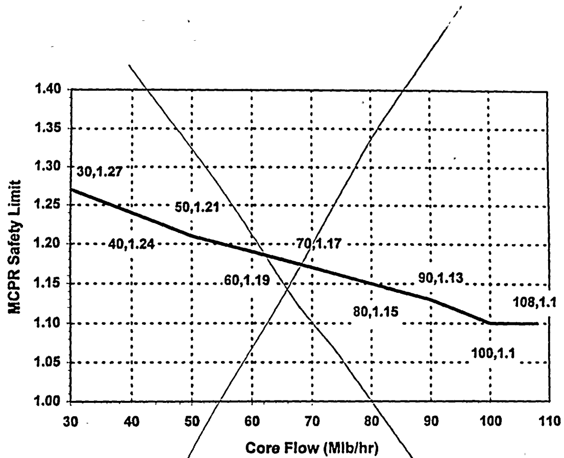
Figure 2.1.2-1 MCPR Safety Limit vs Core Flow
