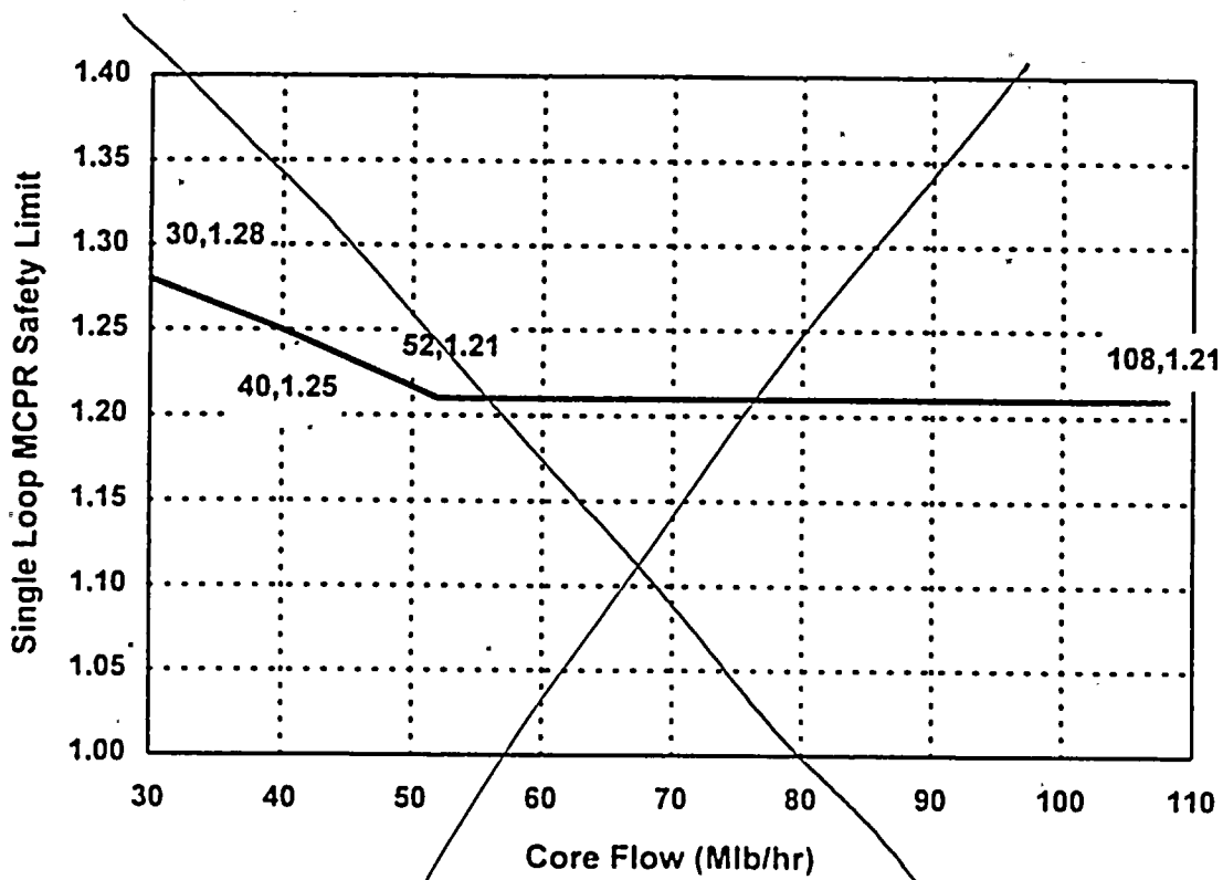
Figure 3.4.1.1.2-1 MCPR Safety Limit vs Core Flow Single Loop Operation
