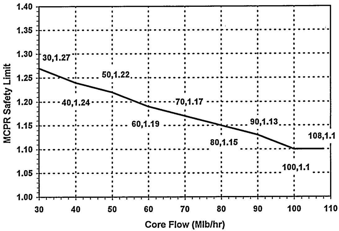
Figure 2.1.2-1 MCPR Safety Limit vs Core Flow
