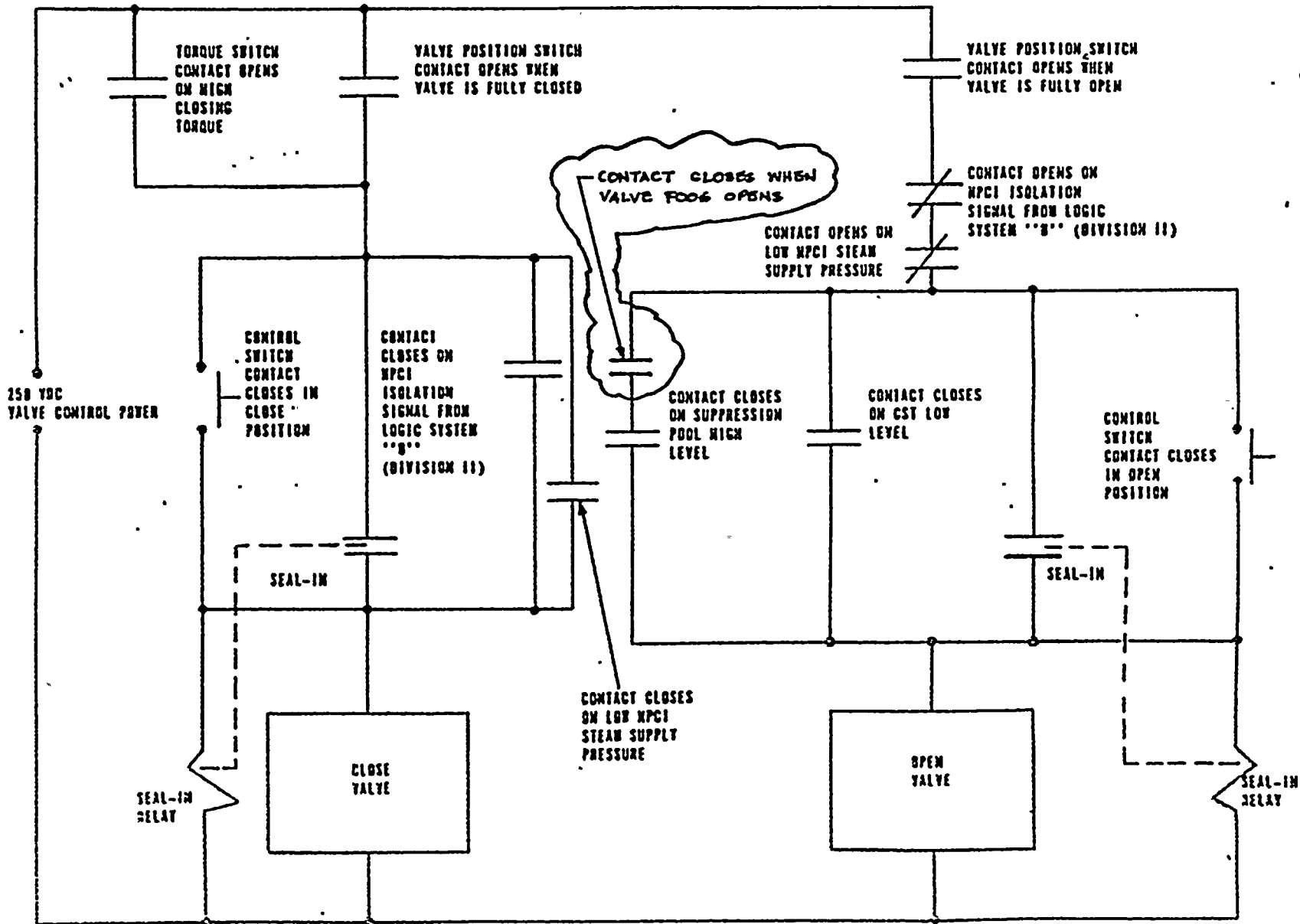
SIMPLIFIED SCHEMATIC DIAGRAM OF VALVE F942 CONTROL CIRCUIT
