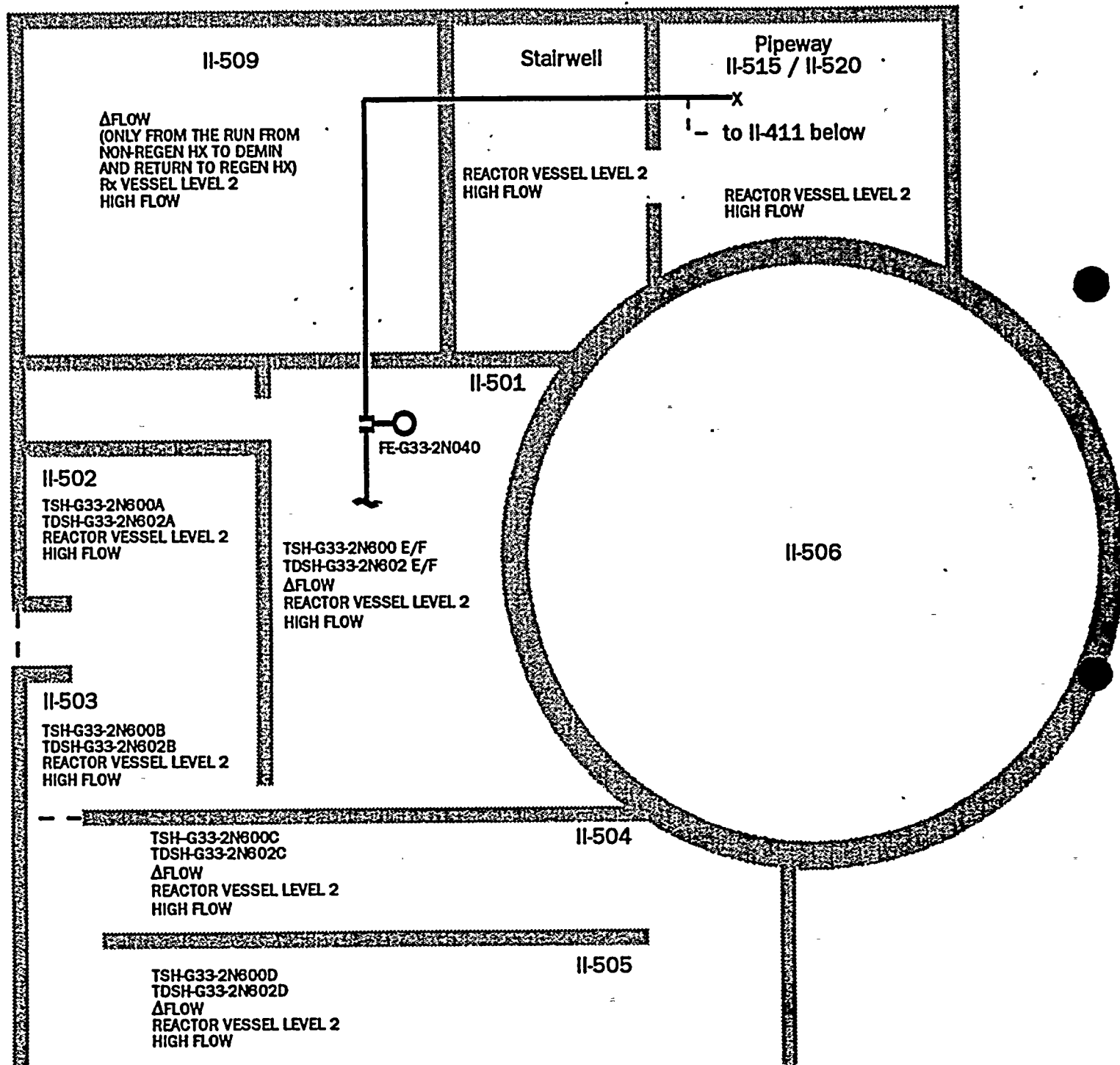
FIGURE 2: ROOM LAYOUT FOR RWCU PIPING (not to scale)
