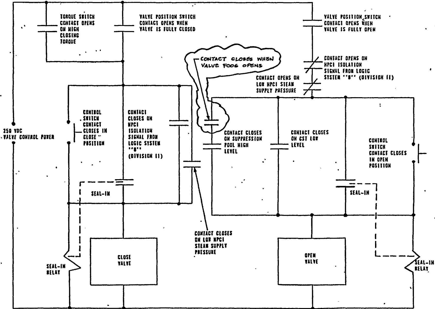
SIMPLIFIED SCHEMATIC DIAGRAM OF VALVE FB42 CONTROL CIRCUIT
